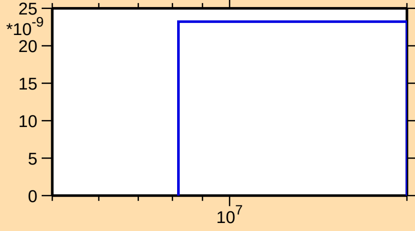
\sigma vs. E for ^{153}\text{Pr}(n,nt)
