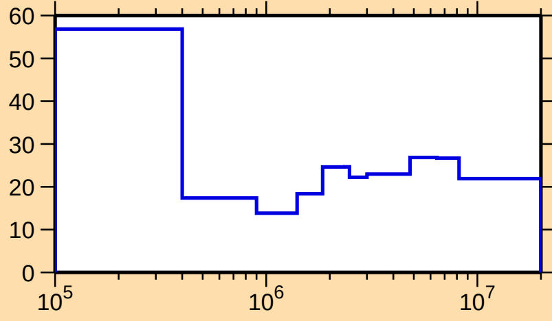
\Delta\sigma/\sigma vs. E for ^{153}\text{Pr}(n,\text{tot.})
