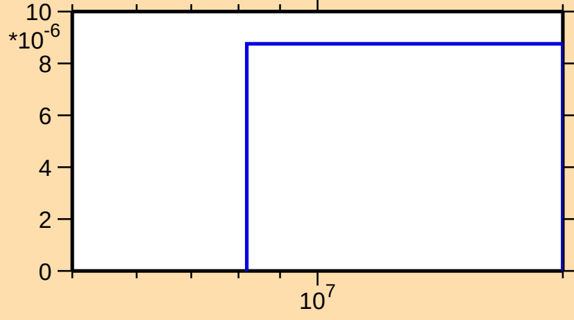
\sigma vs. E for ^{153}\text{Pr}(n,np)
