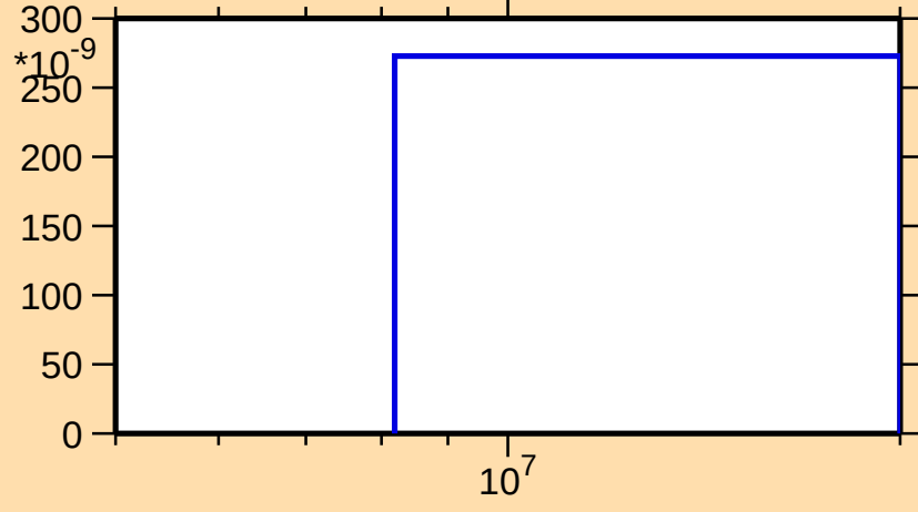
\sigma vs. E for ^{153}\text{Pr}(n,n\alpha)
