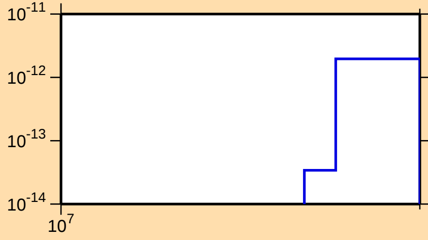
\sigma vs. E for ^{189}\text{Pt}(n,3n\alpha)
