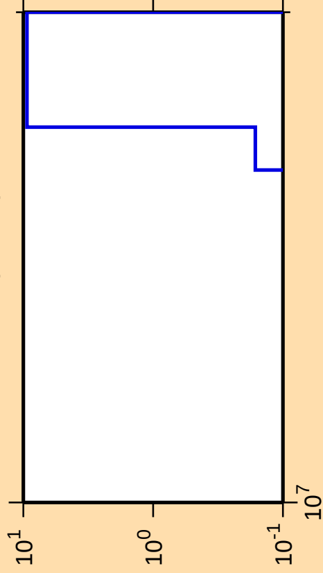
\Delta\sigma/\sigma vs. E for ^{189}\text{Pt}(n,3n\alpha)
