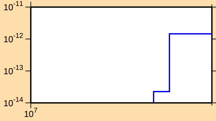
\sigma vs. E for ^{189}\text{Pt}(n,\text{pd})
