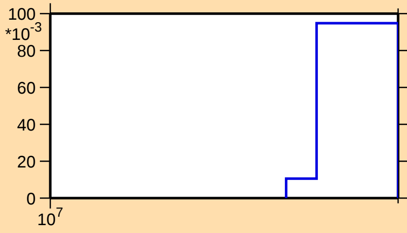
\sigma vs. E for ^{189}\text{Pt}(n,3n)
