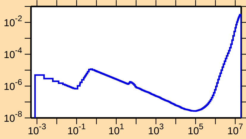
\sigma vs. E for ^{189}\text{Pt}(n,p)
