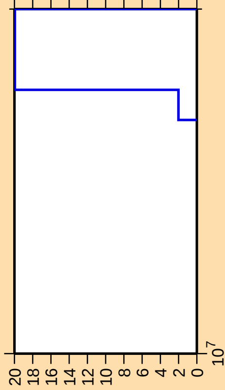
\Delta\sigma/\sigma vs. E for ^{189}\text{Pt}(\text{mt117})
