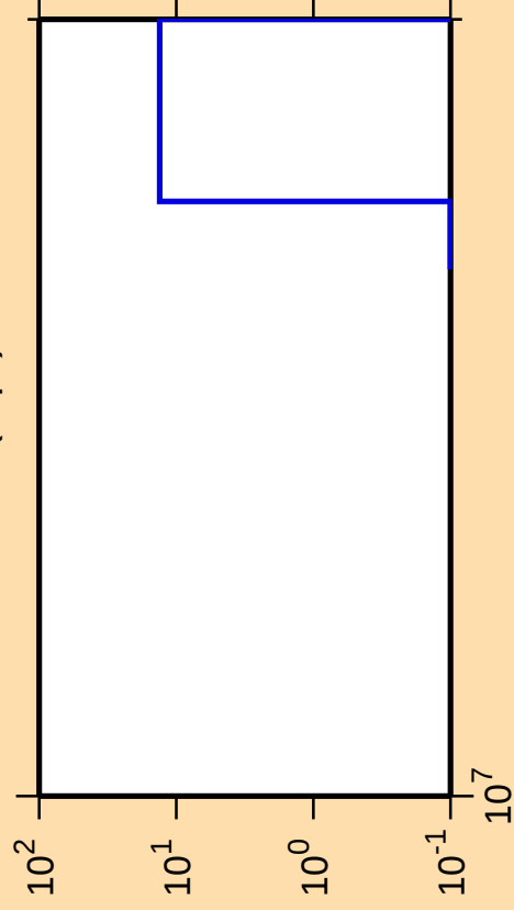
\Delta\sigma/\sigma vs. E for ^{189}\text{Pt}(n,\text{pt})
