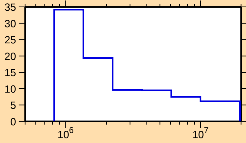
\Delta\sigma/\sigma vs. E for ^{189}\text{Pt}(n,n\text{onel.})
