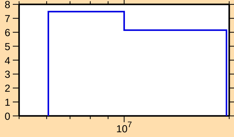
\Delta\sigma/\sigma vs. E for ^{189}\text{Pt}(n,\text{nonel.})
