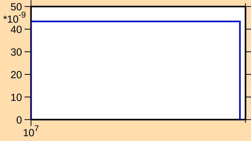
\sigma vs. E for ^{189}\text{Pt}(n,\text{nd})
