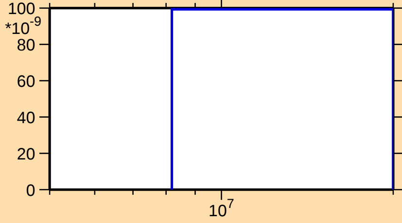
\sigma vs. E for ^{189}\text{Pt}(n,2np)
