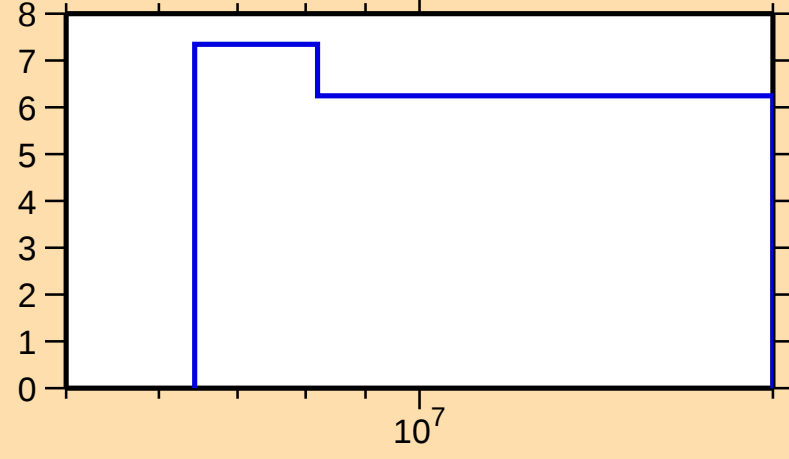
\Delta\sigma/\sigma vs. E for ^{189}\text{Pt}(n,\text{nonel.})
