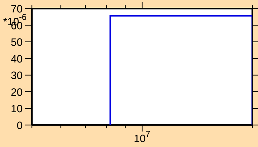
\sigma vs. E for ^{189}\text{Pt}(n,t)
