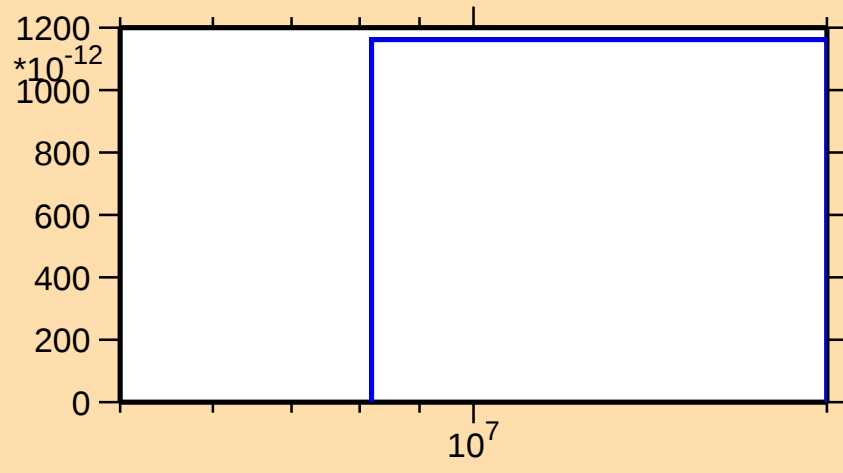
\sigma vs. E for ^{189}\text{Pt}(n,p\alpha)
