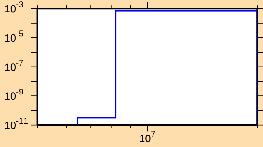
\sigma vs. E for ^{189}\text{Pt}(n,np)
