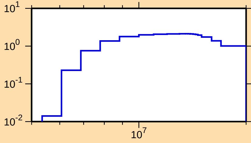
\sigma vs. E for ^{199}\text{Pt}(n,2n)
