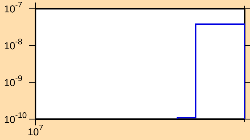
\sigma vs. E for ^{199}\text{Pt}(n,\text{nd})
