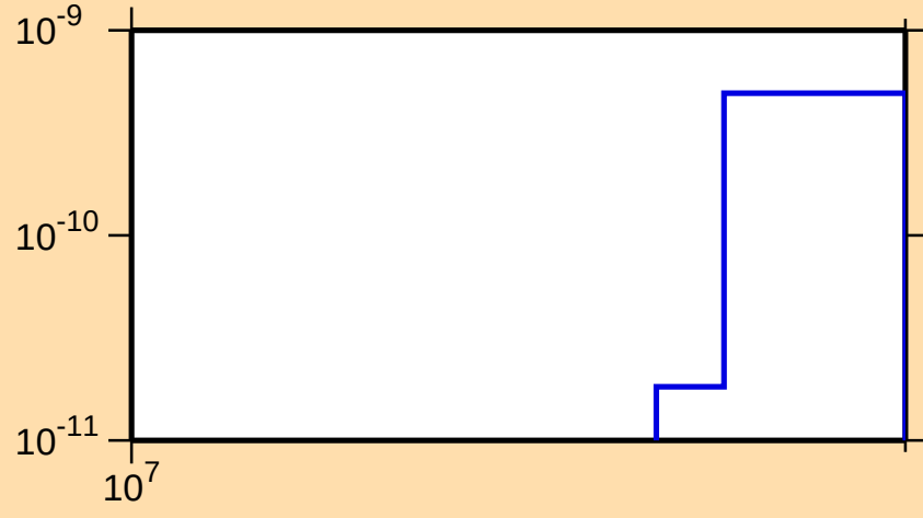
\sigma vs. E for ^{199}\text{Pt}(n,2n\alpha)
