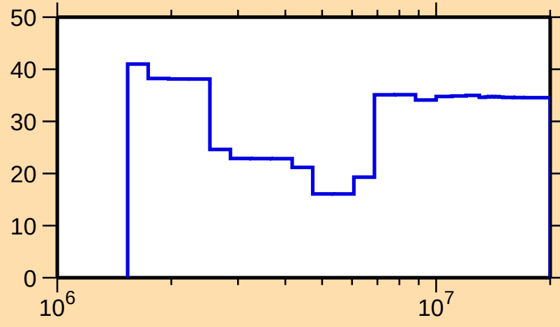
\Delta\sigma/\sigma vs. E for ^{199}\text{Pt}(n,n\text{cont.})
