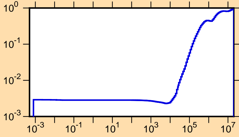
\mu vs. E for ^{231}\text{Pu}(\text{mt251})
