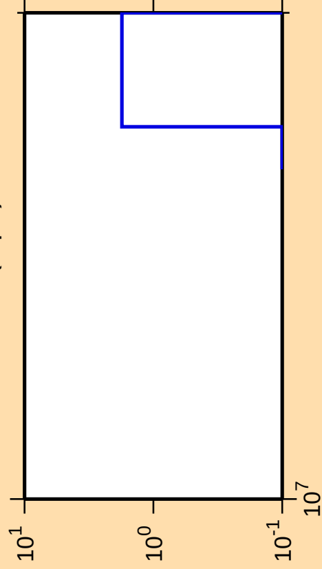
\Delta\sigma/\sigma vs. E for ^{231}\text{Pu}(n,\text{pd})
