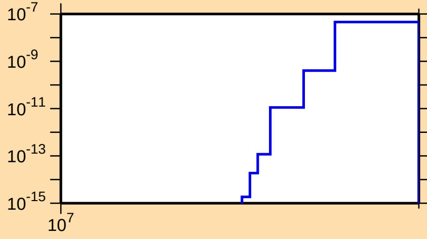
\sigma vs. E for ^{231}\text{Pu}(n,nt)
