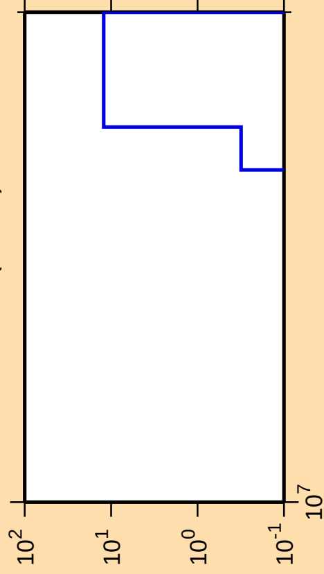
\Delta\sigma/\sigma vs. E for ^{231}\text{Pu} (mt 34)
