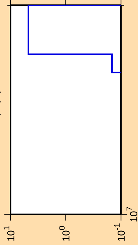
\Delta\sigma/\sigma vs. E for ^{231}\text{Pu}(n,\text{pt})
