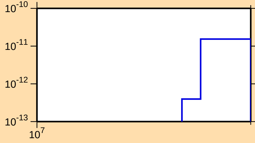
\sigma vs. E for ^{231}\text{Pu} (mt 34)
