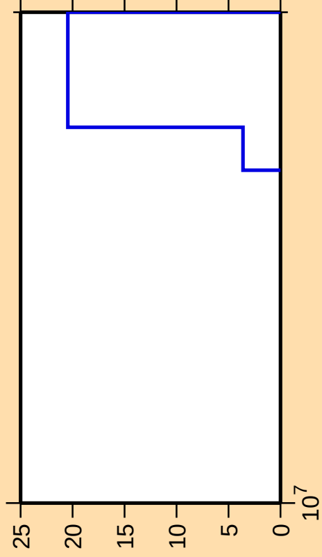
\Delta\sigma/\sigma vs. E for ^{231}\text{Pu}(\text{mt117})
