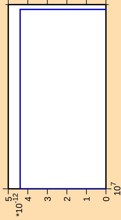
\Delta\sigma/\sigma vs. E for ^{231}\text{Pu} (mt 42)
