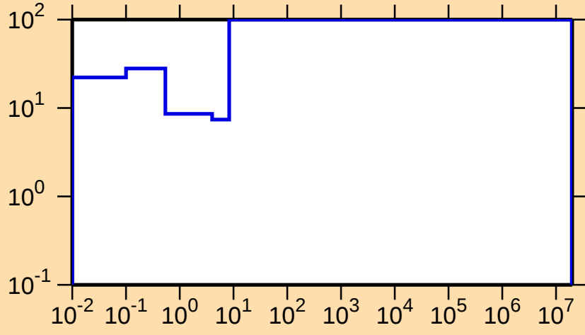
\Delta\sigma/\sigma vs. E for ^{231}\text{Pu}(n,\gamma)
