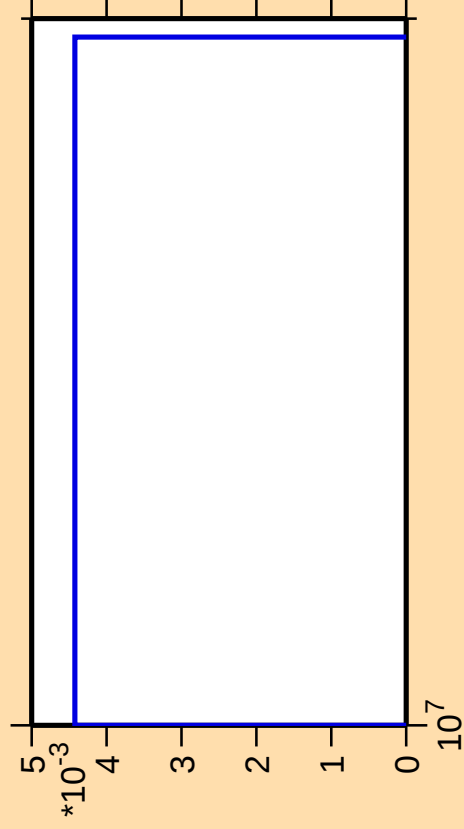
\Delta\sigma/\sigma vs. E for ^{231}\text{Pu}(n,3n\alpha)
