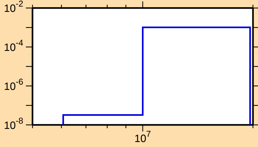
\sigma vs. E for ^{231}\text{Pu}(n,d)
