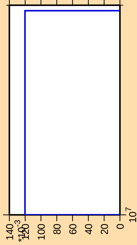
\Delta\sigma/\sigma vs. E for ^{231}\text{Pu}(\text{mt } 34)
