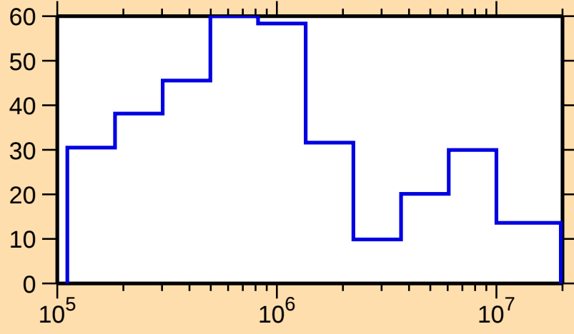
\Delta\sigma/\sigma vs. E for ^{231}\text{Pu}(n,\text{el.})
