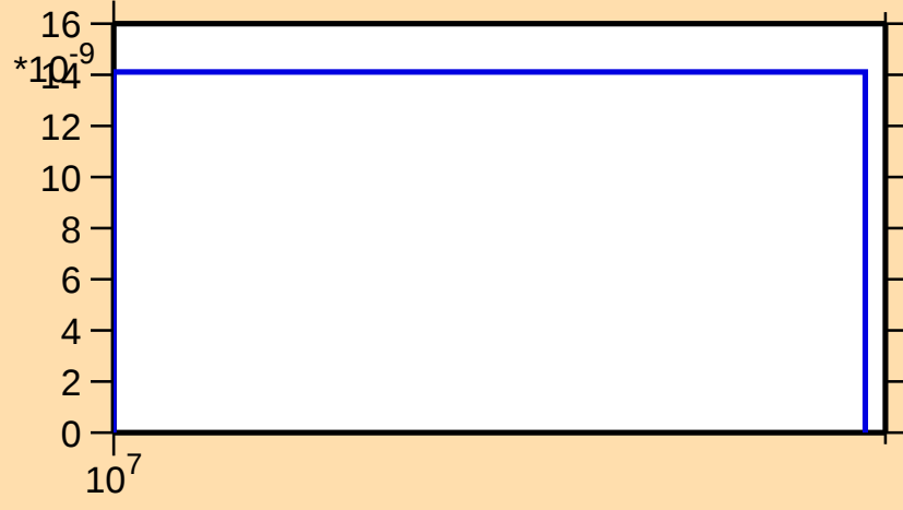
\sigma vs. E for ^{231}\text{Pu}(n,3n)
