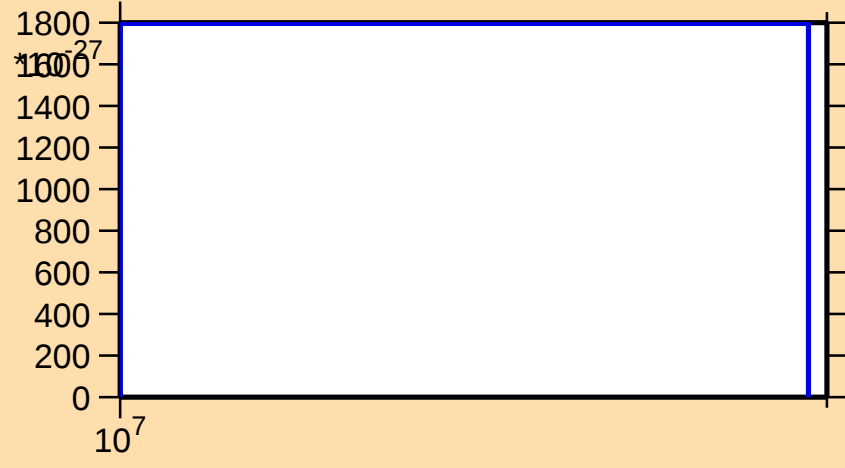
\sigma vs. E for ^{231}\text{Pu} (mt 42)
