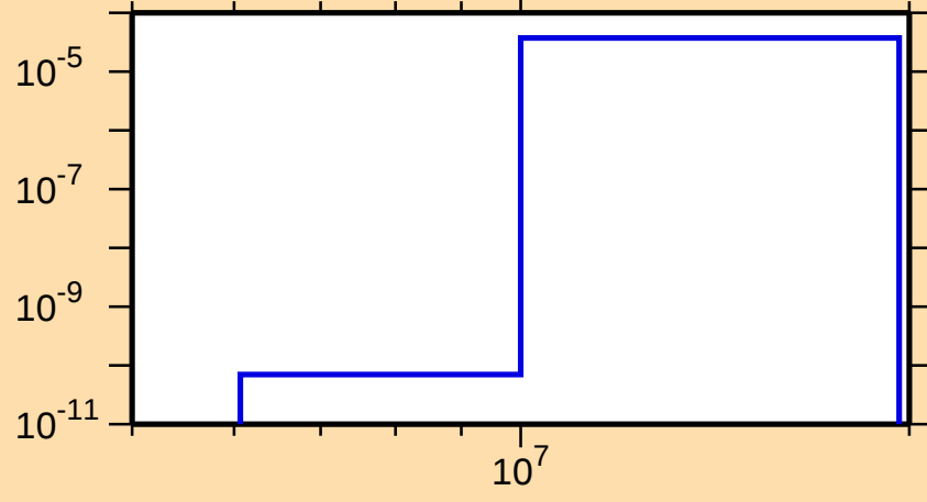
\sigma vs. E for ^{231}\text{Pu}(n,np)
