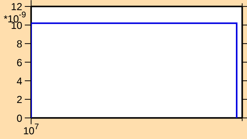
\sigma vs. E for ^{231}\text{Pu}(n,2np)
