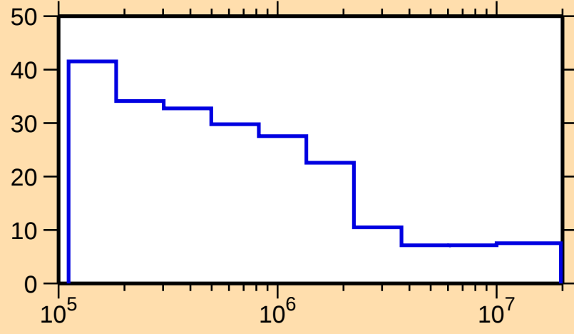
\Delta\sigma/\sigma vs. E for ^{231}\text{Pu}(n,\text{nonel.})
