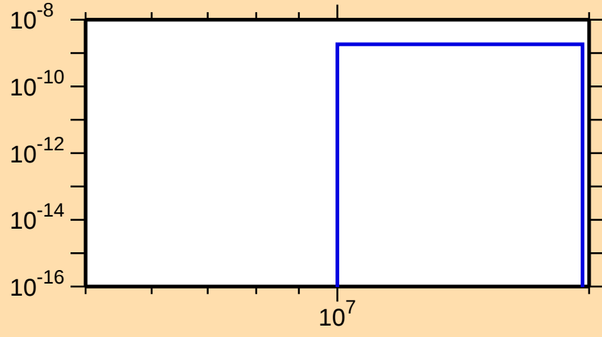
\sigma vs. E for ^{231}\text{Pu}(n,\text{He3})
