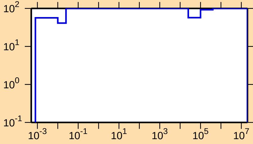
\Delta\sigma/\sigma vs. E for ^{231}\text{Pu}(n,p)
