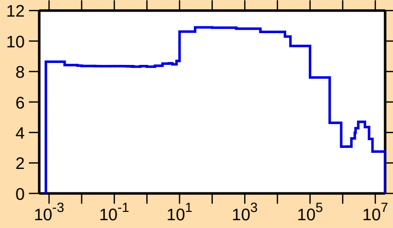
\sigma vs. E for ^{231}\text{Pu}(n,\text{el.})
