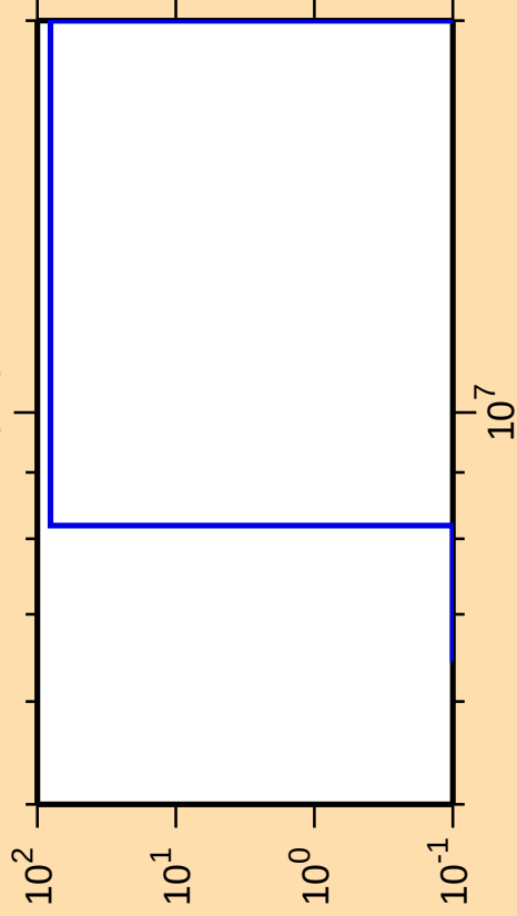
\Delta\sigma/\sigma vs. E for ^{231}\text{Pu}(n,t)
