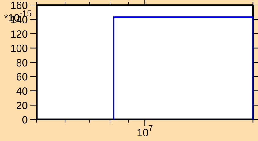
\sigma vs. E for ^{231}\text{Pu}(\text{mt } 34)
