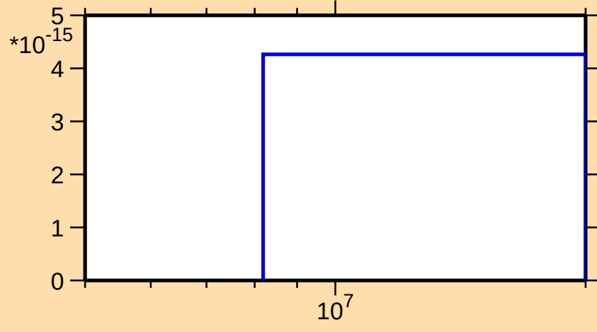
\sigma vs. E for ^{231}\text{Pu}(n,3n\alpha)
