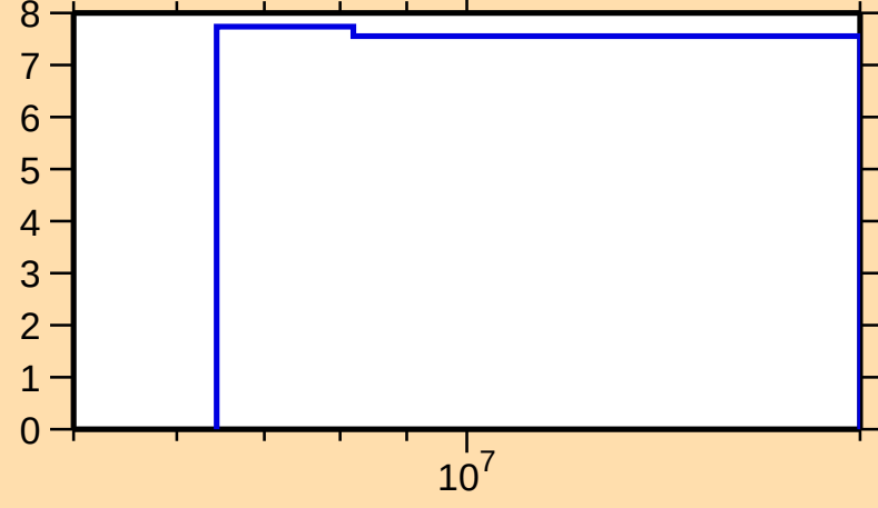
\Delta\sigma/\sigma vs. E for ^{231}\text{Pu}(n,\text{nonel.})
