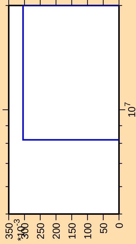
\Delta\sigma/\sigma vs. E for ^{231}\text{Pu}(\text{mt117})
