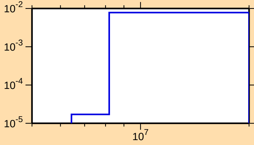
\sigma vs. E for ^{231}\text{Pu}(n,2n)
