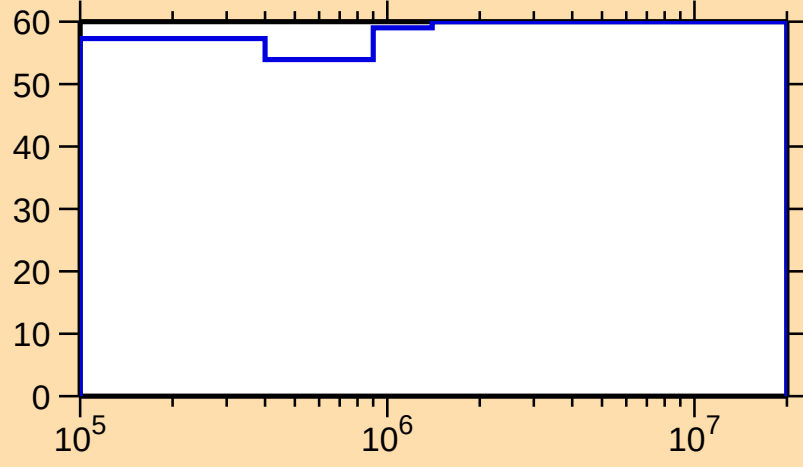
\Delta\sigma/\sigma vs. E for ^{231}\text{Pu}(n,n_1)
