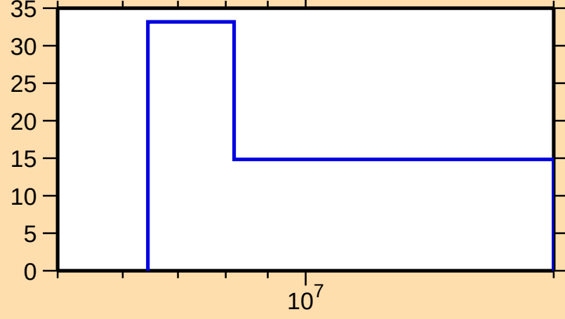
\Delta\sigma/\sigma vs. E for ^{231}\text{Pu}(n,\text{el.})
