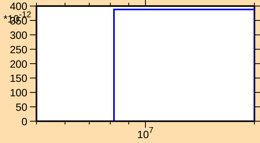
\sigma vs. E for ^{231}\text{Pu}(n,nt)
