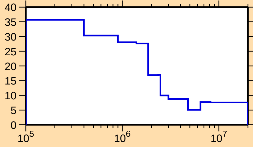
\Delta\sigma/\sigma vs. E for ^{231}\text{Pu}(n,n\text{onel.})
