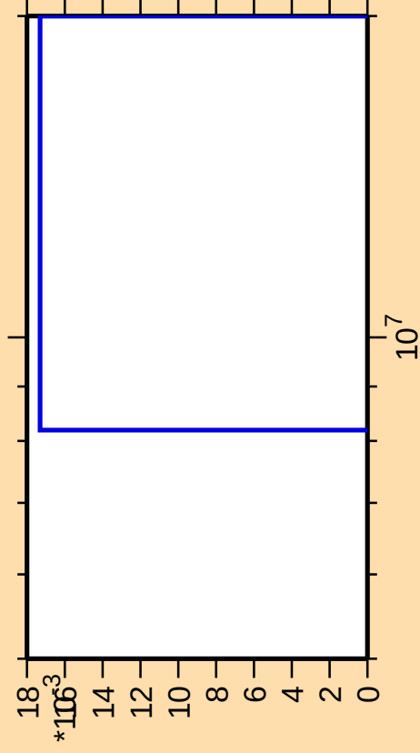
\Delta\sigma/\sigma vs. E for ^{231}\text{Pu}(n,\text{pd})
