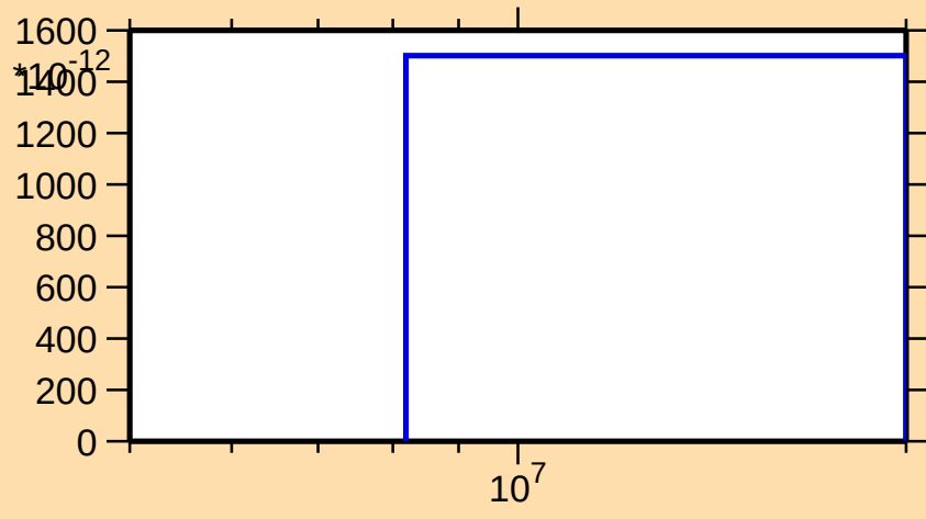
\sigma vs. E for ^{231}\text{Pu}(n,\text{He3})
