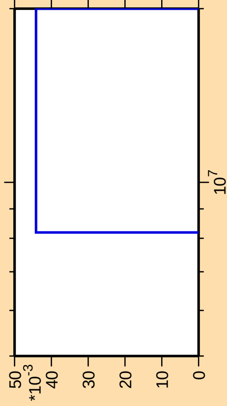
\Delta\sigma/\sigma vs. E for ^{231}\text{Pu}(n,\text{pt})
