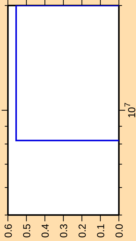
\Delta\sigma/\sigma vs. E for ^{231}\text{Pu}(\text{mt 45})
