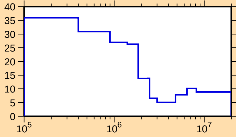
\Delta\sigma/\sigma vs. E for ^{231}\text{Pu}(n,f)
