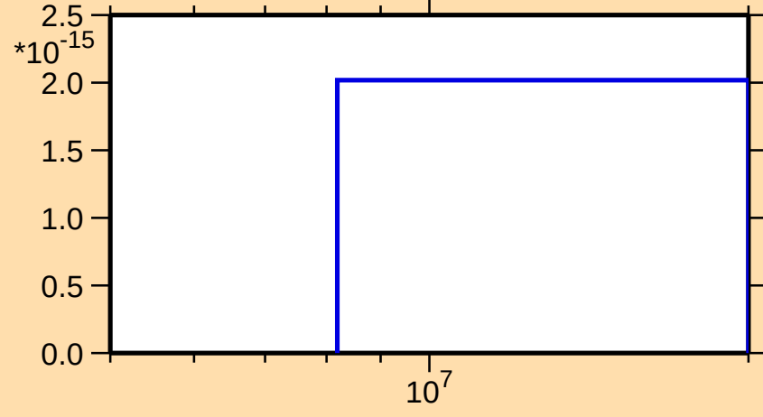
\sigma vs. E for ^{231}\text{Pu}(n,\text{pd})
