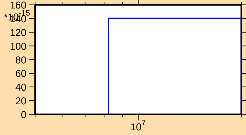
\sigma vs. E for ^{231}\text{Pu}(\text{mt 45})
