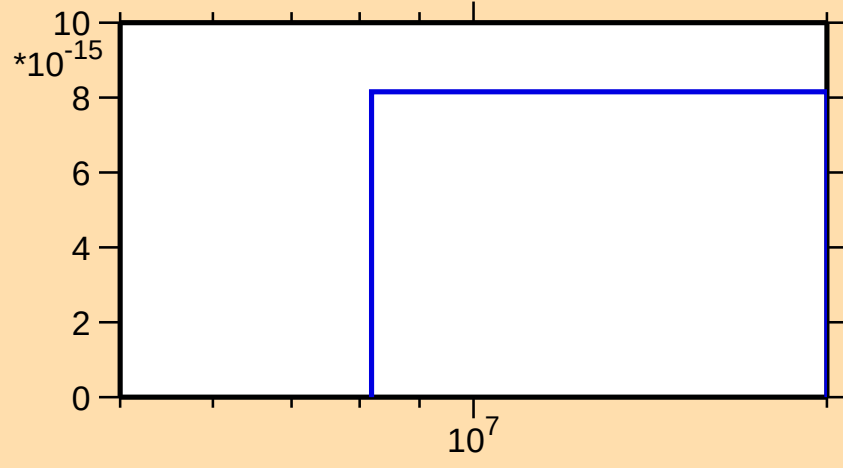
\sigma vs. E for ^{231}\text{Pu}(n,\text{pt})
