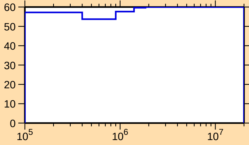
\Delta\sigma/\sigma vs. E for ^{231}\text{Pu}(n,\text{inel.})
