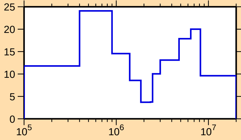
\Delta\sigma/\sigma vs. E for ^{231}\text{Pu}(n,\text{tot.})
