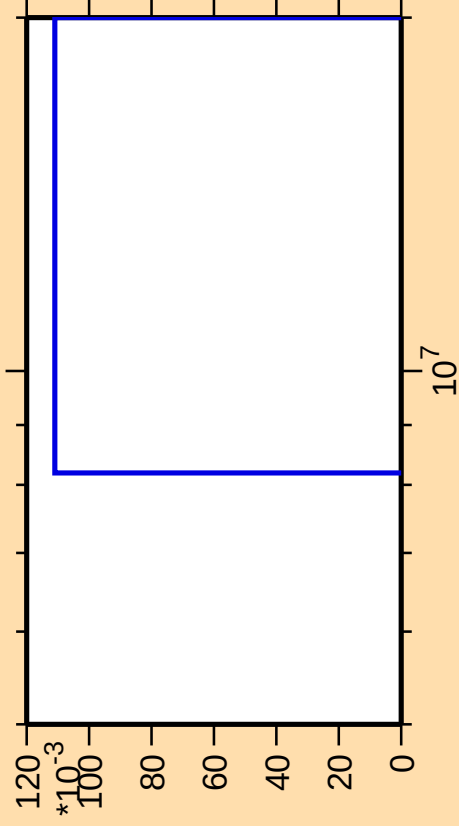
\Delta\sigma/\sigma vs. E for ^{231}\text{Pu}(\text{mt } 34)
