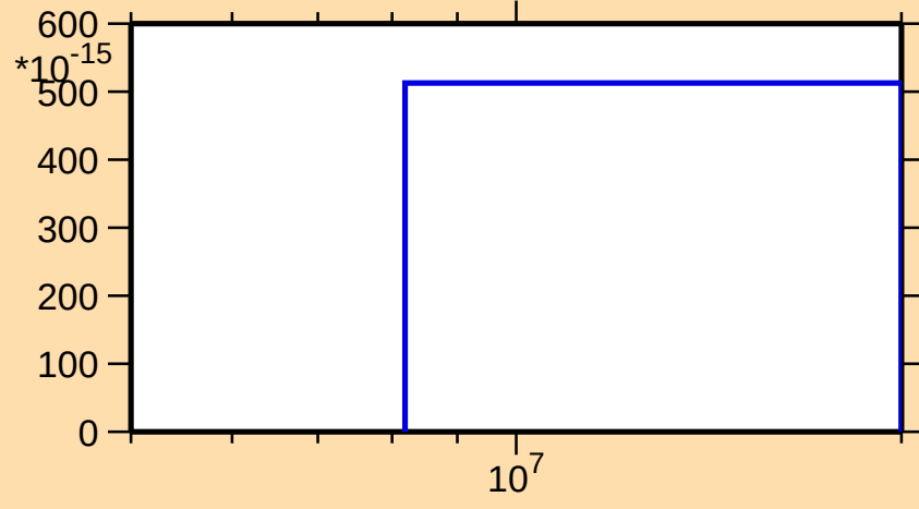
\sigma vs. E for ^{231}\text{Pu}(\text{mt117})
