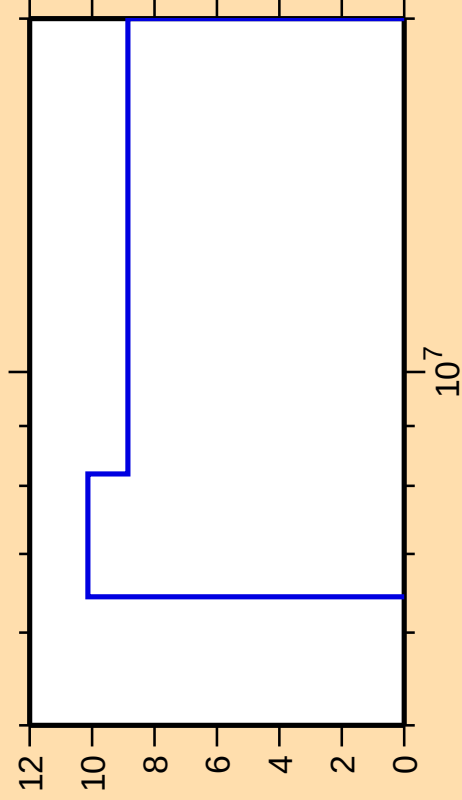
\Delta\sigma/\sigma vs. E for ^{231}\text{Pu}(n,f)
