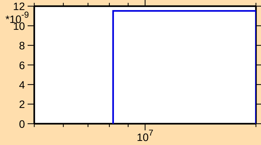
\sigma vs. E for ^{231}\text{Pu}(n,3n)
