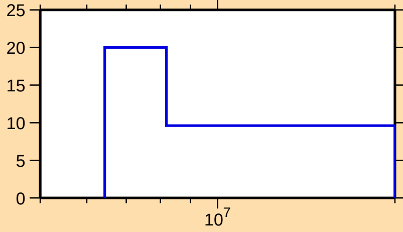
\Delta\sigma/\sigma vs. E for ^{231}\text{Pu}(n,\text{tot.})
