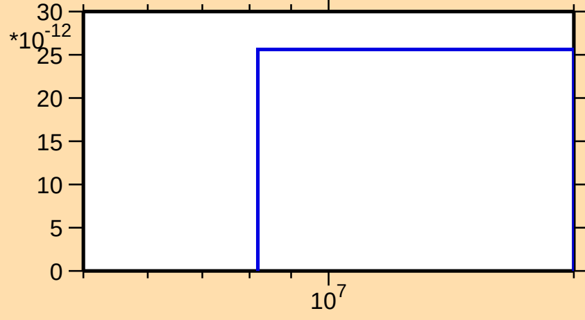
\sigma vs. E for ^{231}\text{Pu}(n,p\alpha)
