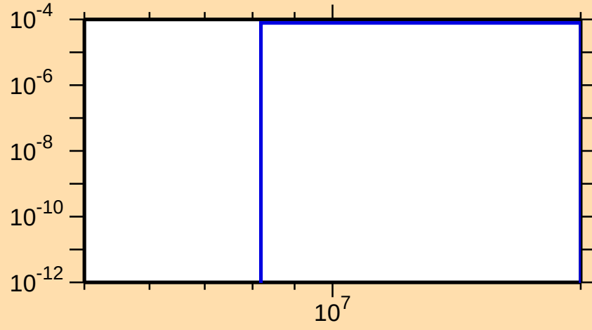
\sigma vs. E for ^{231}\text{Pu}(n,t)
