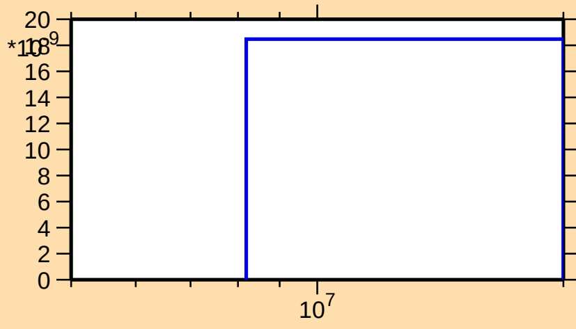
\sigma vs. E for ^{231}\text{Pu}(n,\text{nd})
