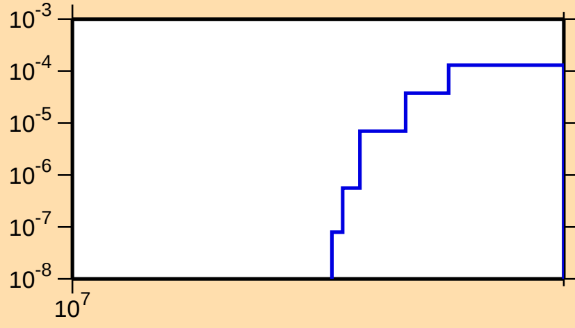
\sigma vs. E for ^{233}\text{Pu}(n,3n)
