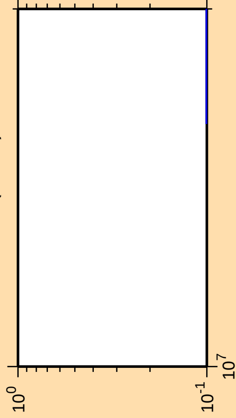
\Delta\sigma/\sigma vs. E for ^{233}\text{Pu}(n,3n\alpha)
