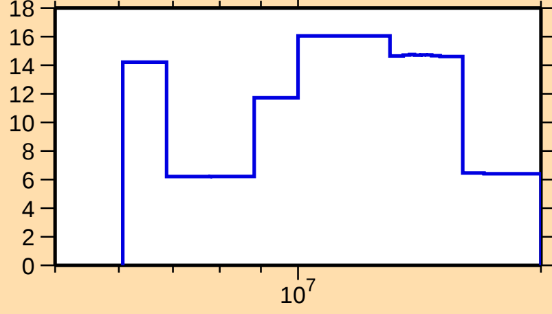
\Delta\sigma/\sigma vs. E for ^{233}\text{Pu}(n,\text{el.})
