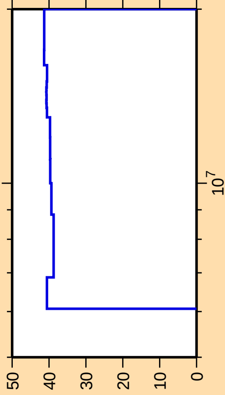
\Delta\sigma/\sigma vs. E for ^{233}\text{Pu}(n,n_1)
