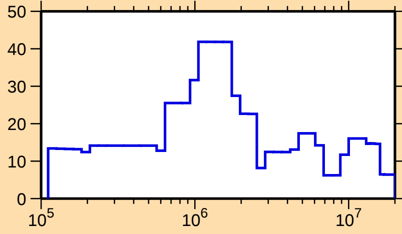
\Delta\sigma/\sigma vs. E for ^{233}\text{Pu}(n,\text{el.})
