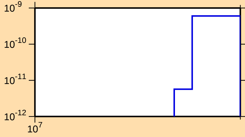
\sigma vs. E for ^{233}\text{Pu}(n,nt)
