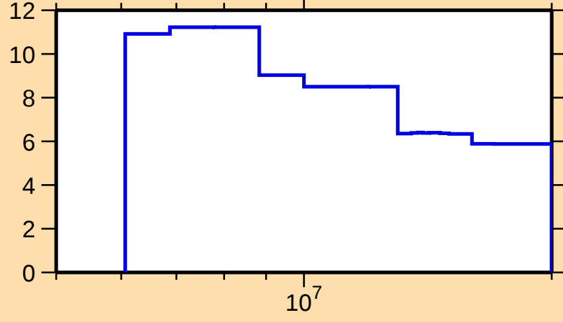
\Delta\sigma/\sigma vs. E for ^{233}\text{Pu}(n,\text{nonel.})
