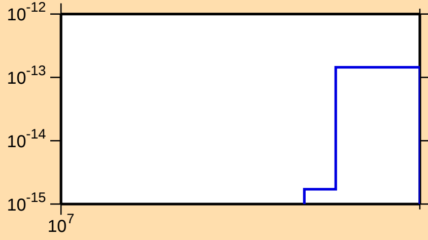
\sigma vs. E for ^{233}\text{Pu}(n,3n\alpha)
