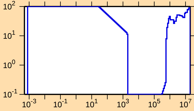
\Delta\sigma/\sigma vs. E for ^{233}\text{Pu}(n,p)
