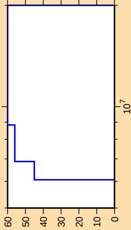
\Delta\sigma/\sigma vs. E for ^{233}\text{Pu}(n,\gamma)
