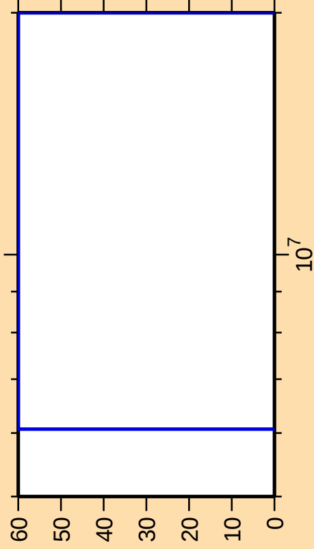
\Delta\sigma/\sigma vs. E for ^{233}\text{Pu}(n,2n)
