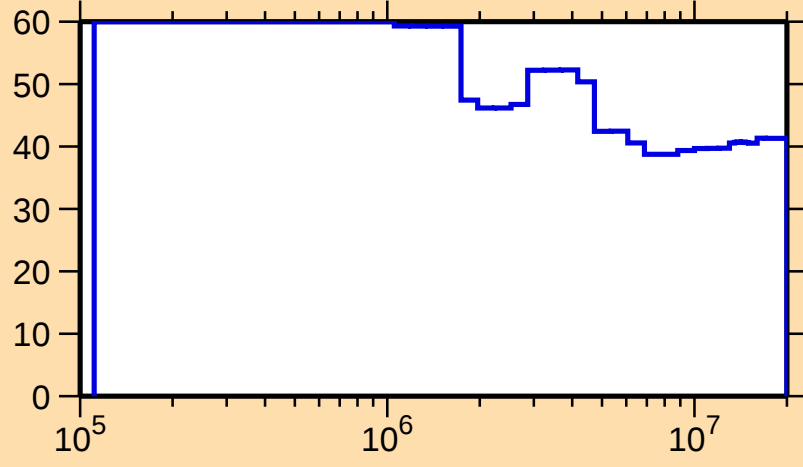
\Delta\sigma/\sigma vs. E for ^{233}\text{Pu}(n,n_1)
