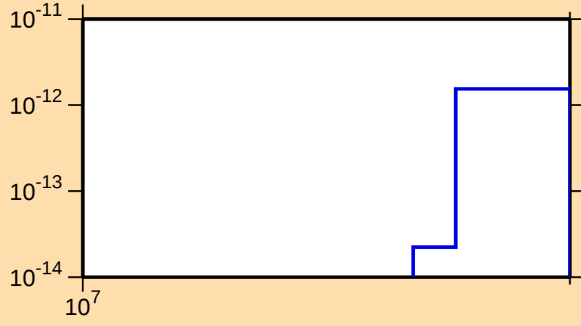
\sigma vs. E for ^{233}\text{Pu} (mt 34)
