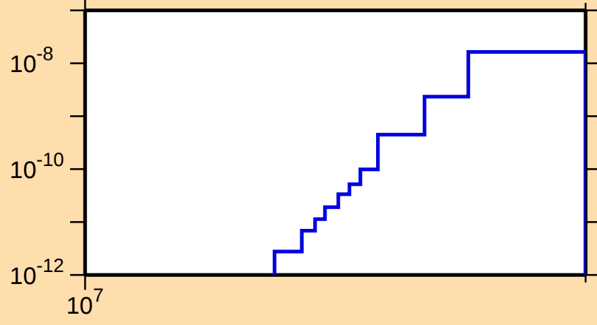
\sigma vs. E for ^{233}\text{Pu}(n,\text{He3})
