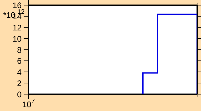
\sigma vs. E for ^{233}\text{Pu}(n,p\alpha)
