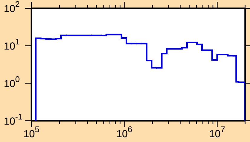
\Delta\sigma/\sigma vs. E for ^{233}\text{Pu}(n,\text{tot.})
