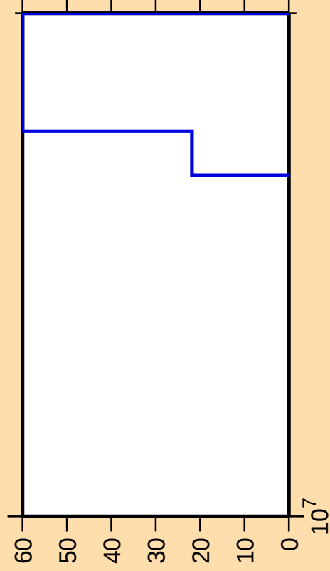
\Delta\sigma/\sigma vs. E for ^{233}\text{Pu}(n,p\alpha)
