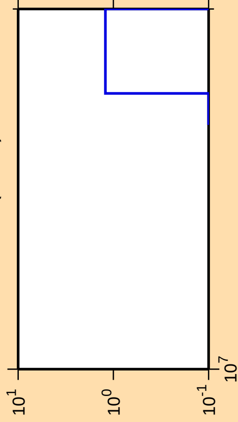
\Delta\sigma/\sigma vs. E for ^{233}\text{Pu} (mt 34)
