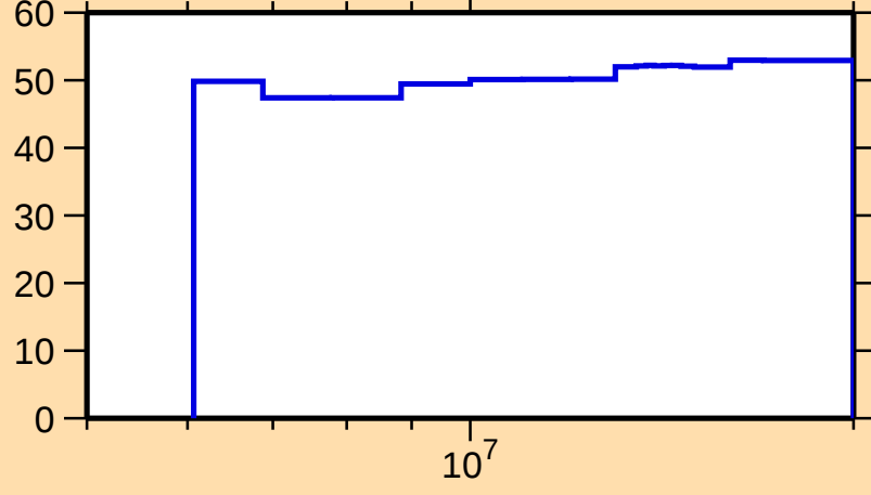
\Delta\sigma/\sigma vs. E for ^{233}\text{Pu}(n,\text{inel.})
