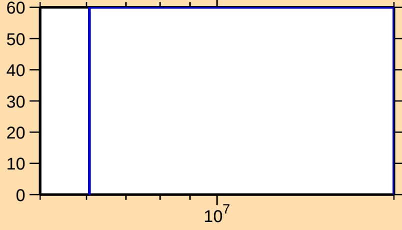
\Delta\sigma/\sigma vs. E for ^{233}\text{Pu}(n,2n)
