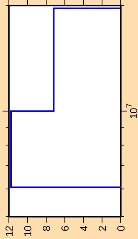
\Delta\sigma/\sigma vs. E for ^{233}\text{Pu}(n,f)
