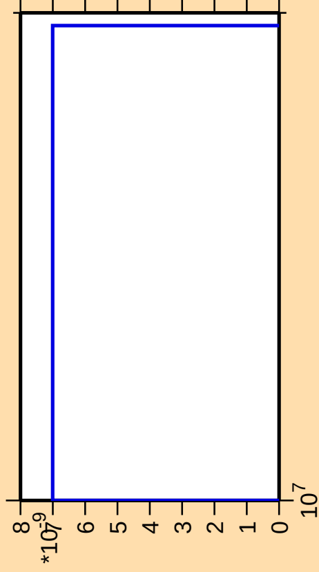
\Delta\sigma/\sigma vs. E for ^{233}\text{Pu} (mt 42)
