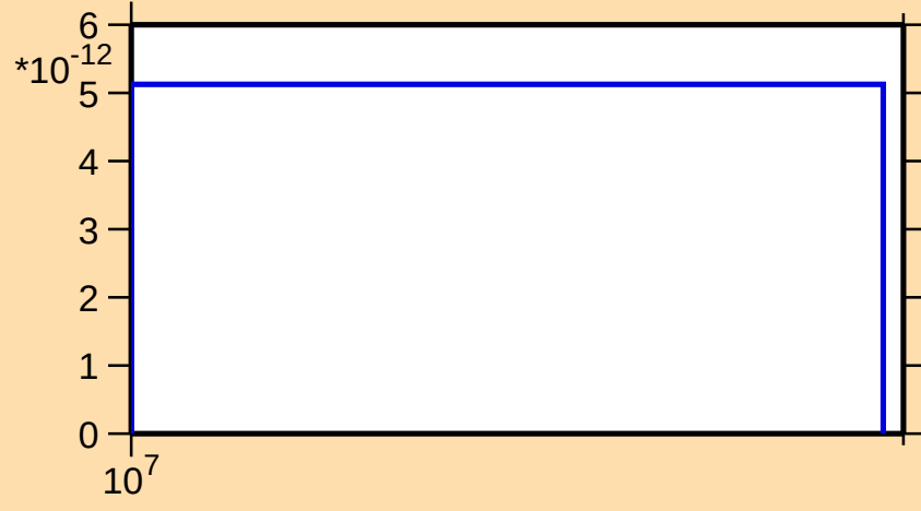
\sigma vs. E for ^{233}\text{Pu}(n,nt)
