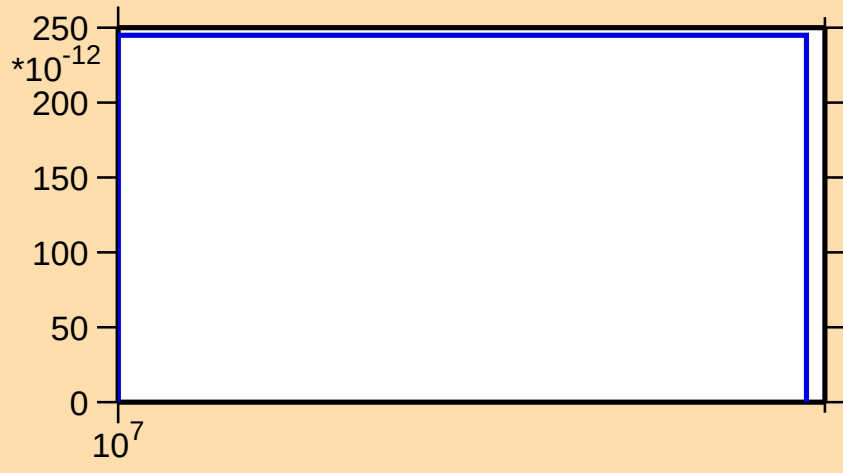
\sigma vs. E for ^{233}\text{Pu}(n,\text{nd})
