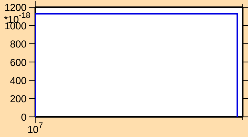
\sigma vs. E for ^{233}\text{Pu}(n,3n\alpha)
