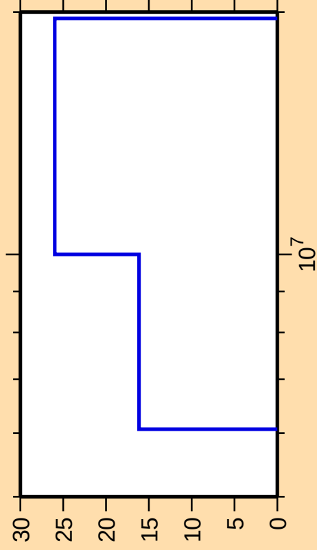
\Delta\sigma/\sigma vs. E for ^{233}\text{Pu}(n,d)
