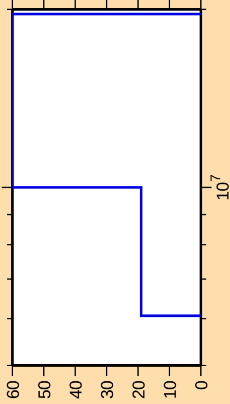
\Delta\sigma/\sigma vs. E for ^{233}\text{Pu}(n,t)
