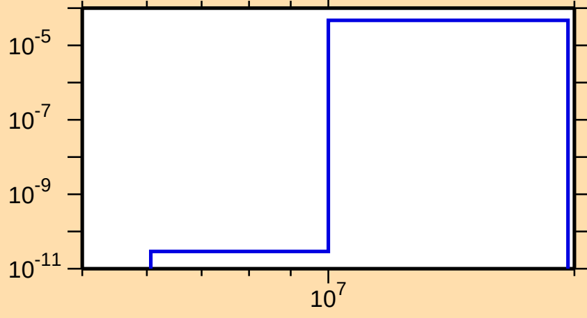
\sigma vs. E for ^{233}\text{Pu}(n,t)
