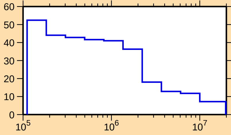
\Delta\sigma/\sigma vs. E for ^{233}\text{Pu}(n,f)
