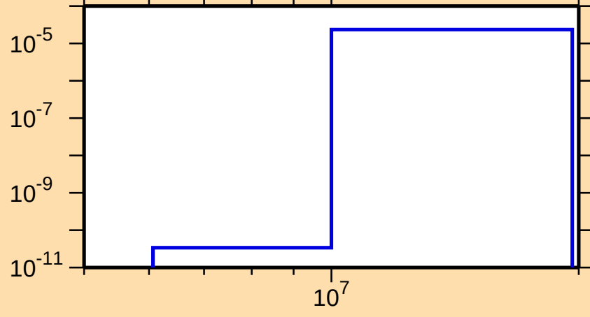
\sigma vs. E for ^{233}\text{Pu}(n,np)
