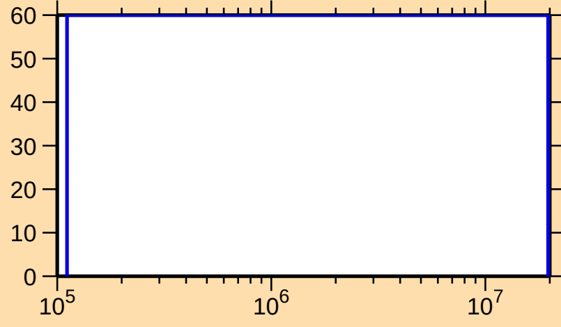
\Delta\sigma/\sigma vs. E for ^{233}\text{Pu}(n,n\text{cont.})
