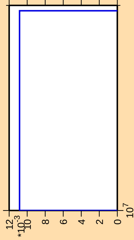
\Delta\sigma/\sigma vs. E for ^{233}\text{Pu}(\text{mt } 34)
