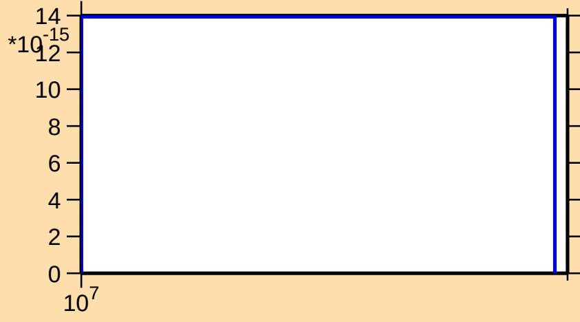
\sigma vs. E for ^{233}\text{Pu}(\text{mt } 34)
