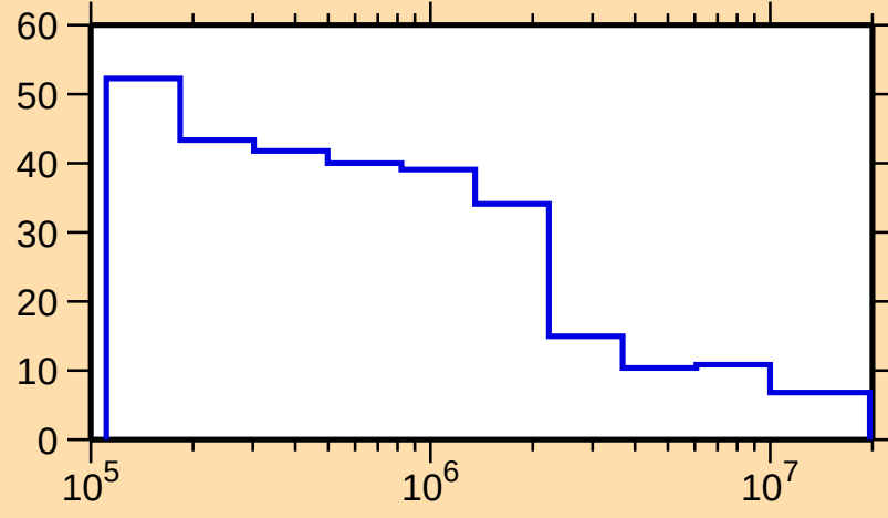
\Delta\sigma/\sigma vs. E for ^{233}\text{Pu}(n,\text{nonel.})
