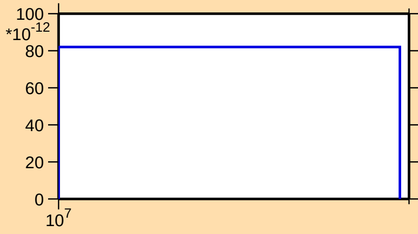
\sigma vs. E for ^{233}\text{Pu}(n,2np)
