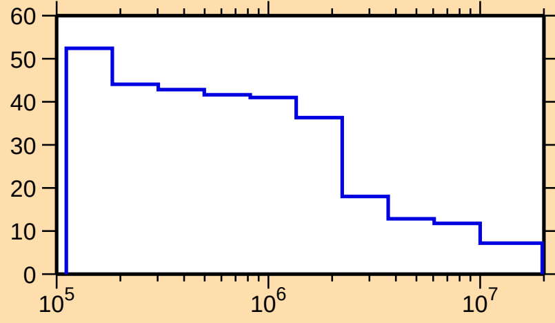
\Delta\sigma/\sigma vs. E for ^{233}\text{Pu}(n,f)
