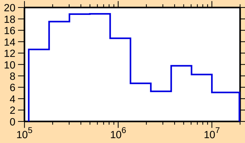
\Delta\sigma/\sigma vs. E for ^{233}\text{Pu}(n,\text{tot.})
