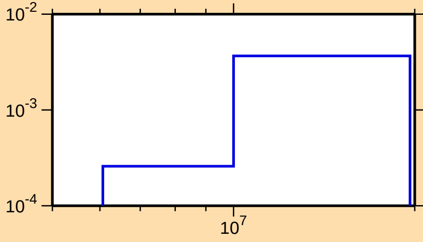
\sigma vs. E for ^{233}\text{Pu}(n,2n)
