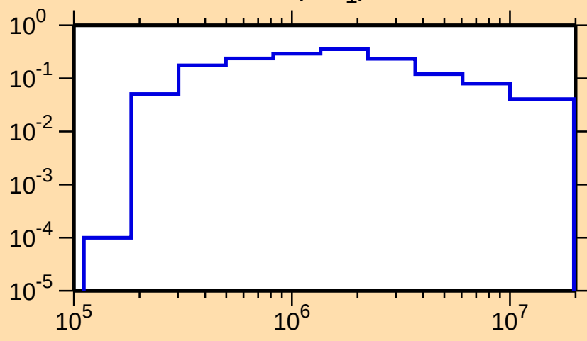
\sigma vs. E for ^{233}\text{Pu}(n,n_1)
