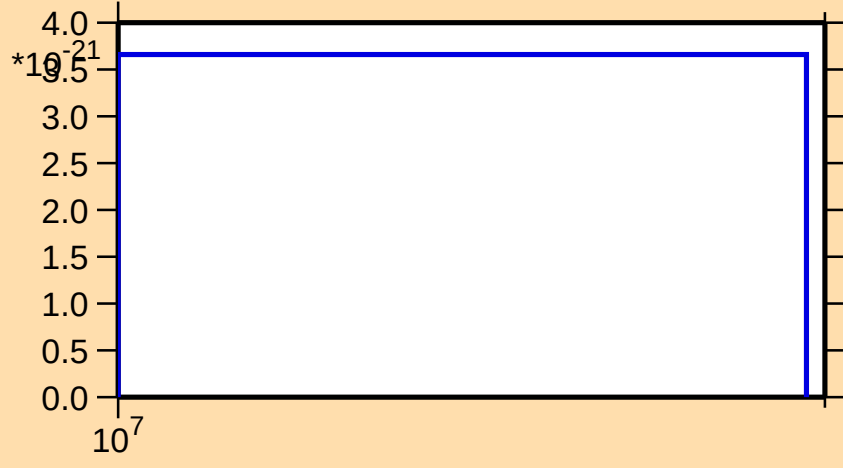
\sigma vs. E for ^{233}\text{Pu} (mt 42)
