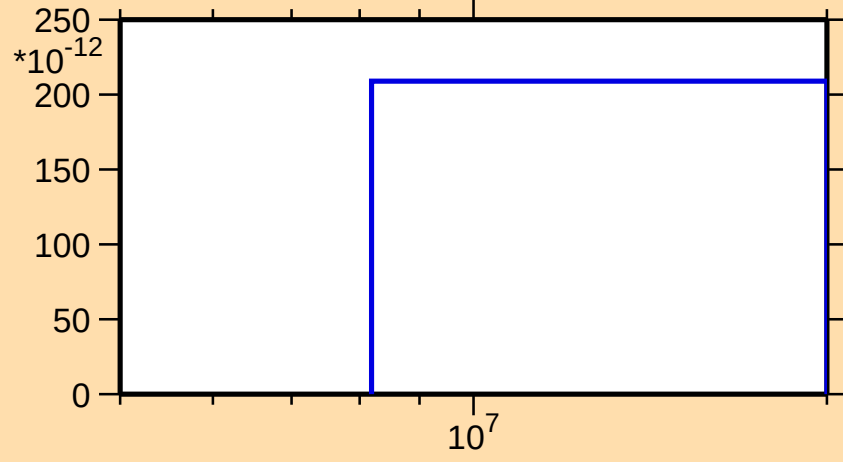
\sigma vs. E for ^{233}\text{Pu}(n,\text{nd})
