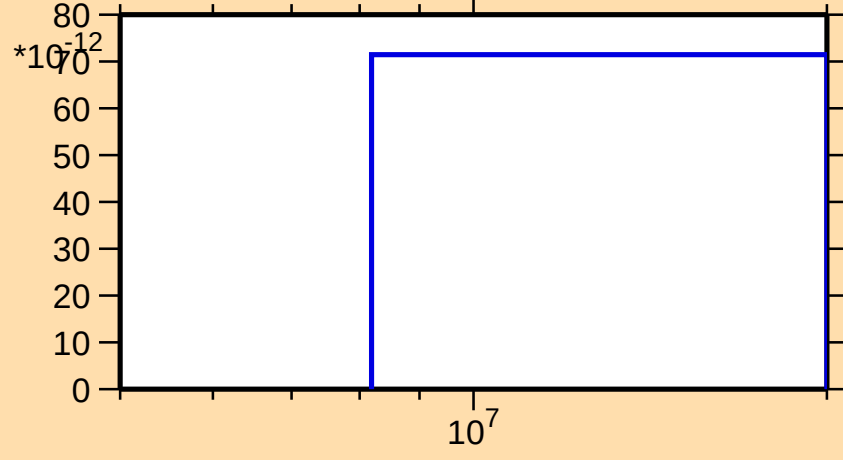
\sigma vs. E for ^{233}\text{Pu}(n,2np)
