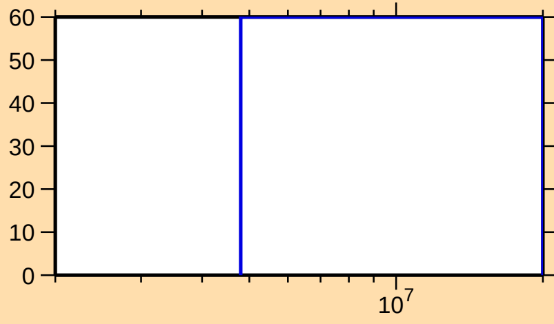
\Delta\sigma/\sigma vs. E for ^{233}\text{Pu}(n,2n)
