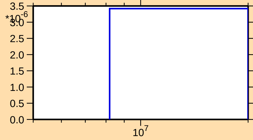
\sigma vs. E for ^{233}\text{Pu}(n,3n)
