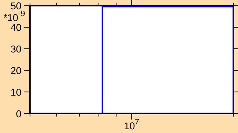
\sigma vs. E for ^{233}\text{Pu}(n,2n\alpha)
