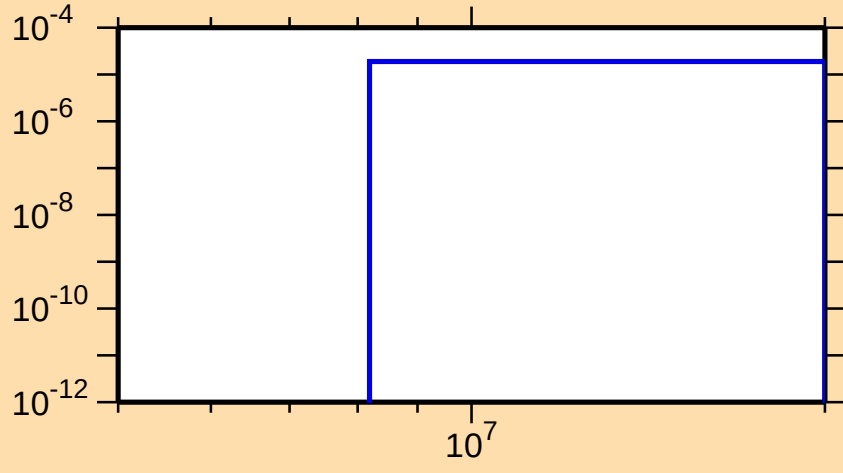
\sigma vs. E for ^{233}\text{Pu}(n,np)
