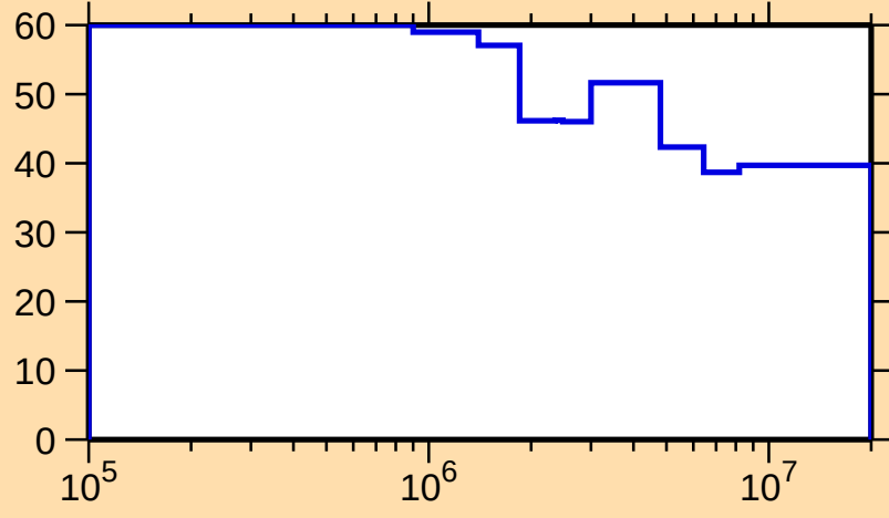
\Delta\sigma/\sigma vs. E for ^{233}\text{Pu}(n,n_1)
