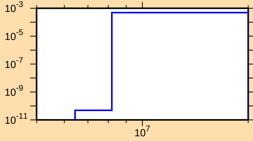
\sigma vs. E for ^{233}\text{Pu}(n,d)
