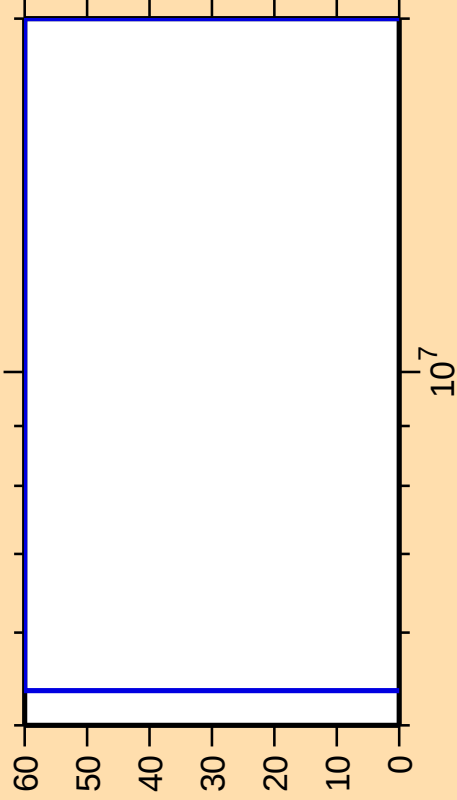
\Delta\sigma/\sigma vs. E for ^{237}\text{Pu}(n,2n)
