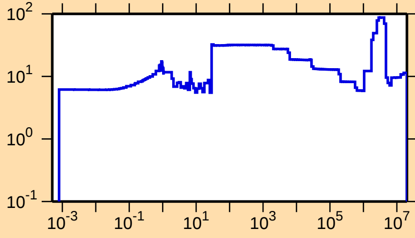
\Delta\sigma/\sigma vs. E for ^{237}\text{Pu}(n,f)
