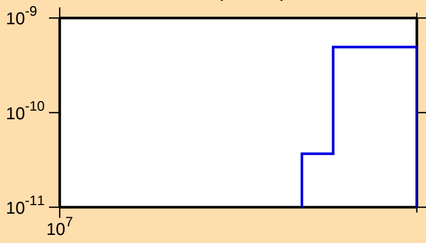
\sigma vs. E for ^{237}\text{Pu}(n,\text{He3})
