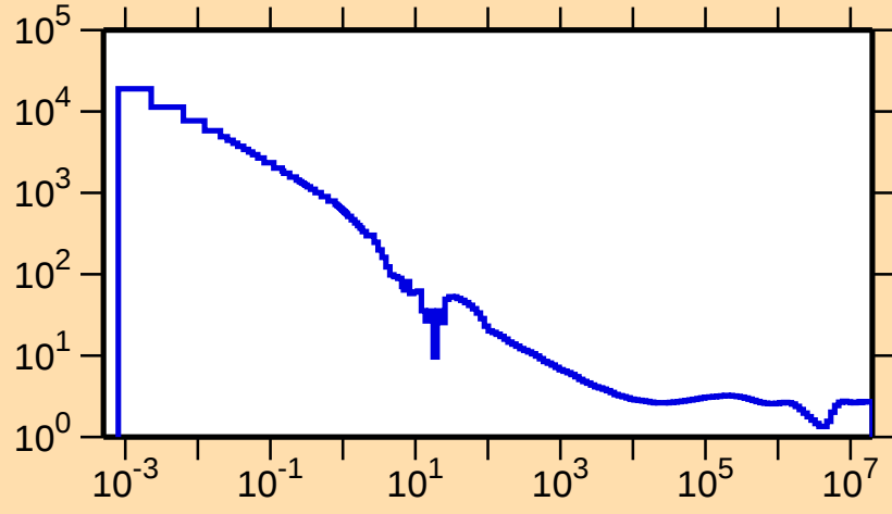
\sigma vs. E for ^{237}\text{Pu}(n,f)
