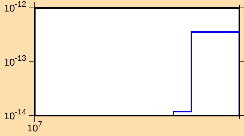
\sigma vs. E for ^{237}\text{Pu}(n,3n\alpha)
