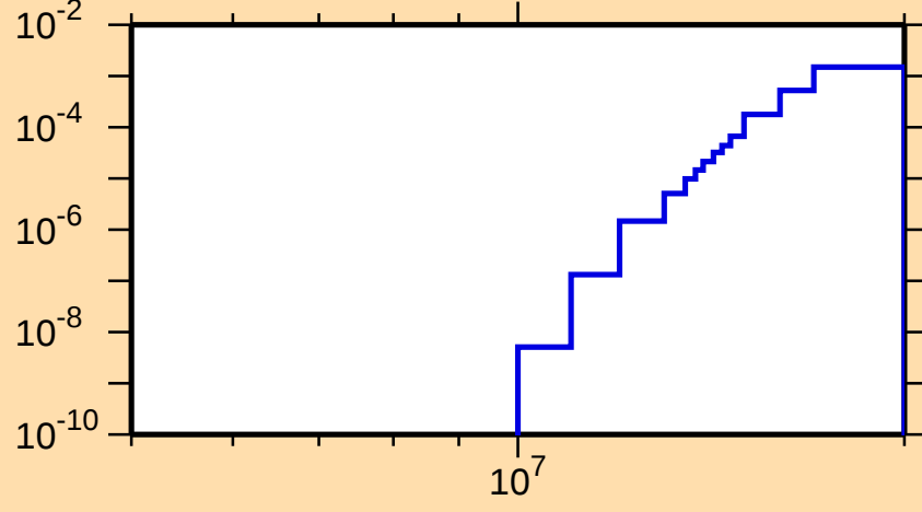
\sigma vs. E for ^{237}\text{Pu}(n,np)
