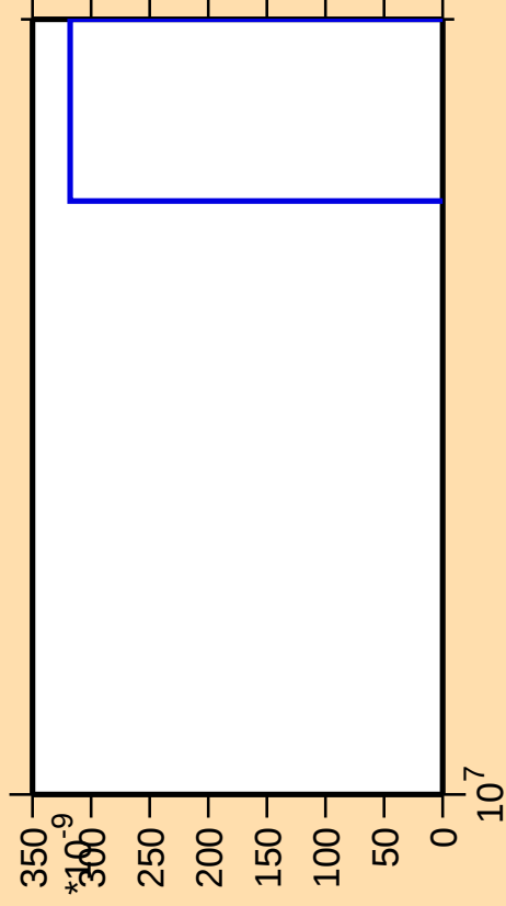
\Delta\sigma/\sigma vs. E for ^{237}\text{Pu} (mt 42)
