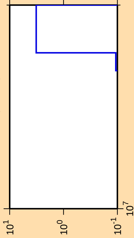
\Delta\sigma/\sigma vs. E for ^{237}\text{Pu}(n,3n\alpha)
