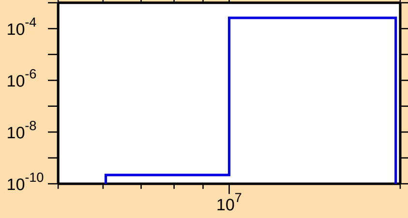
\sigma vs. E for ^{237}\text{Pu}(n,d)
