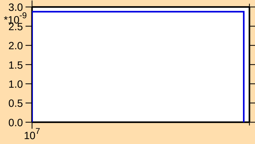
\sigma vs. E for ^{237}\text{Pu}(n,2np)
