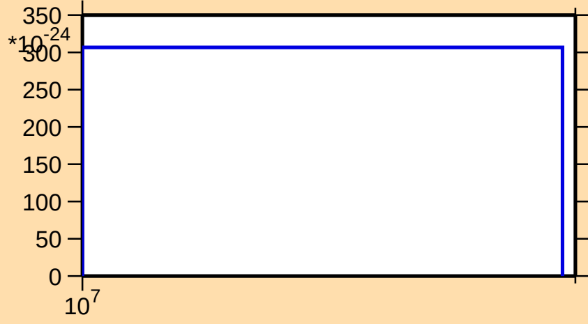
\sigma vs. E for ^{237}\text{Pu} (mt 42)
