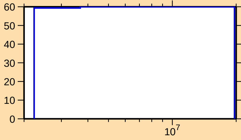
\Delta\sigma/\sigma vs. E for ^{237}\text{Pu}(n,p)
