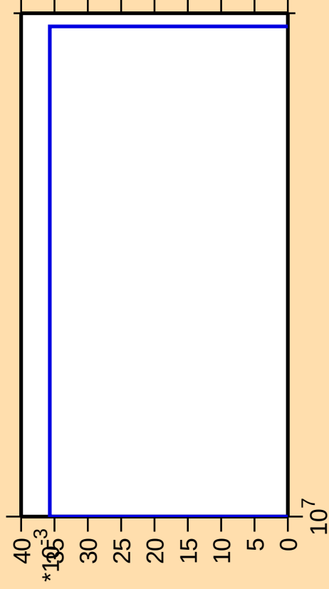
\Delta\sigma/\sigma vs. E for ^{237}\text{Pu}(n,3n\alpha)
