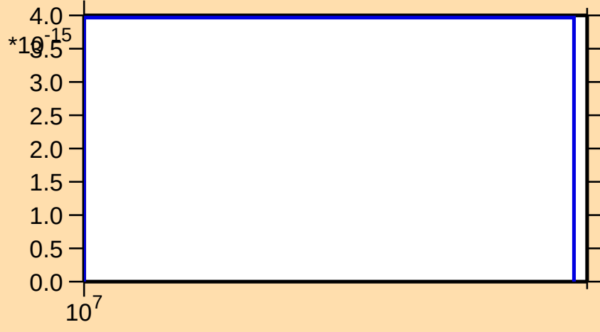
\sigma vs. E for ^{237}\text{Pu}(n,3n\alpha)
