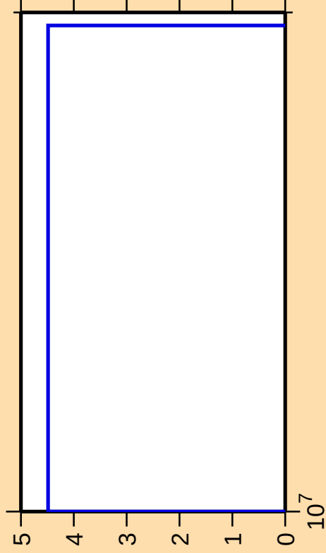
\Delta\sigma/\sigma vs. E for ^{237}\text{Pu}(n,\text{He}3)
