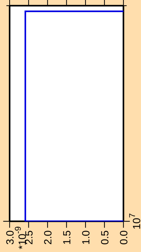
\Delta\sigma/\sigma vs. E for ^{237}\text{Pu} (mt 42)
