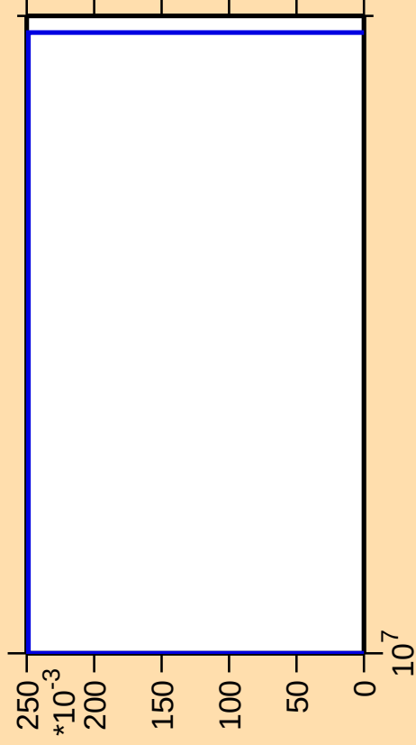
\Delta\sigma/\sigma vs. E for ^{237}\text{Pu}(n,p\alpha)
