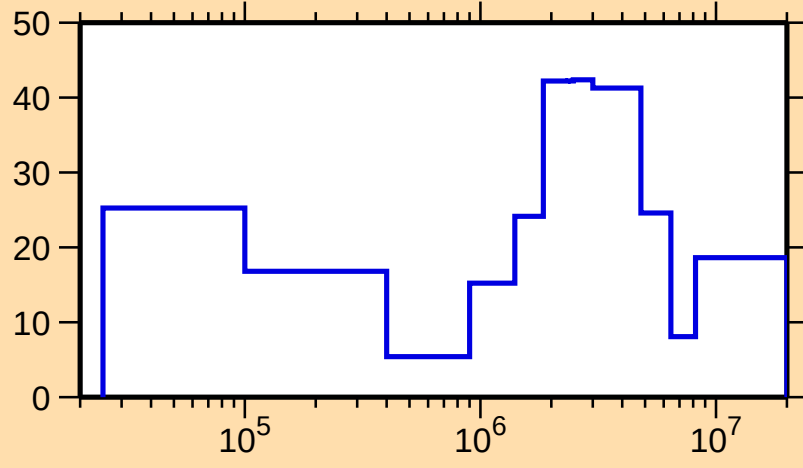
\Delta\sigma/\sigma vs. E for ^{237}\text{Pu}(n,\text{el.})
