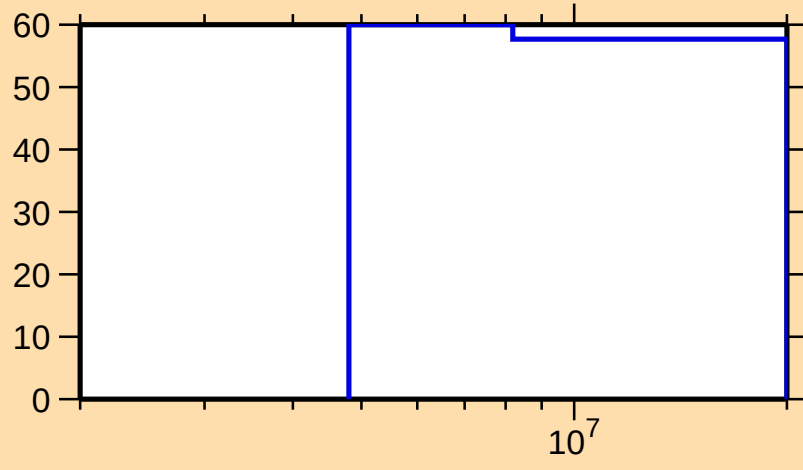
\Delta\sigma/\sigma vs. E for ^{237}\text{Pu}(n,2n)
