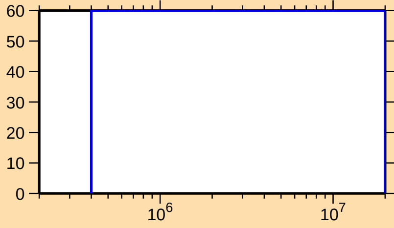
\Delta\sigma/\sigma vs. E for ^{237}\text{Pu}(n,n_1)
