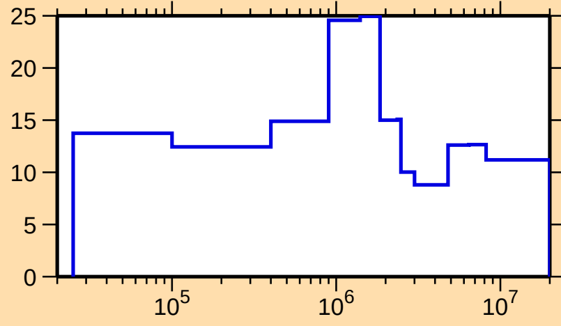
\Delta\sigma/\sigma vs. E for ^{237}\text{Pu}(n,\text{nonel.})
