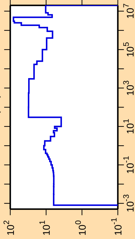
\Delta\sigma/\sigma vs. E for ^{237}\text{Pu}(n,f)
