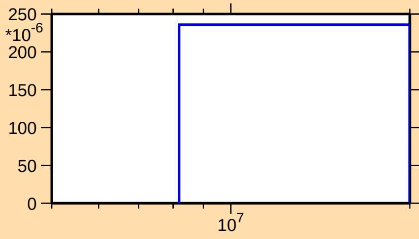
\sigma vs. E for ^{237}\text{Pu}(n,3n)
