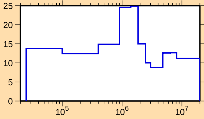
\Delta\sigma/\sigma vs. E for ^{237}\text{Pu}(n,\text{nonel.})
