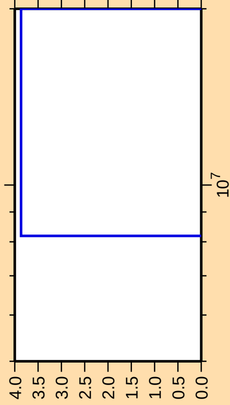
\Delta\sigma/\sigma vs. E for ^{237}\text{Pu}(n,\text{He3})
