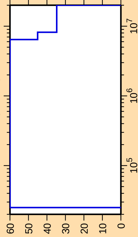
\Delta\sigma/\sigma vs. E for ^{237}\text{Pu}(n,\text{inel.})
