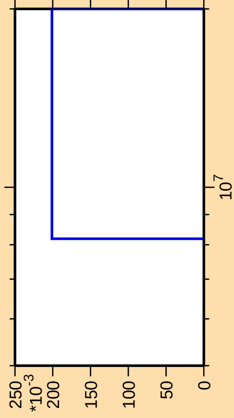
\Delta\sigma/\sigma vs. E for ^{237}\text{Pu}(n,p\alpha)
