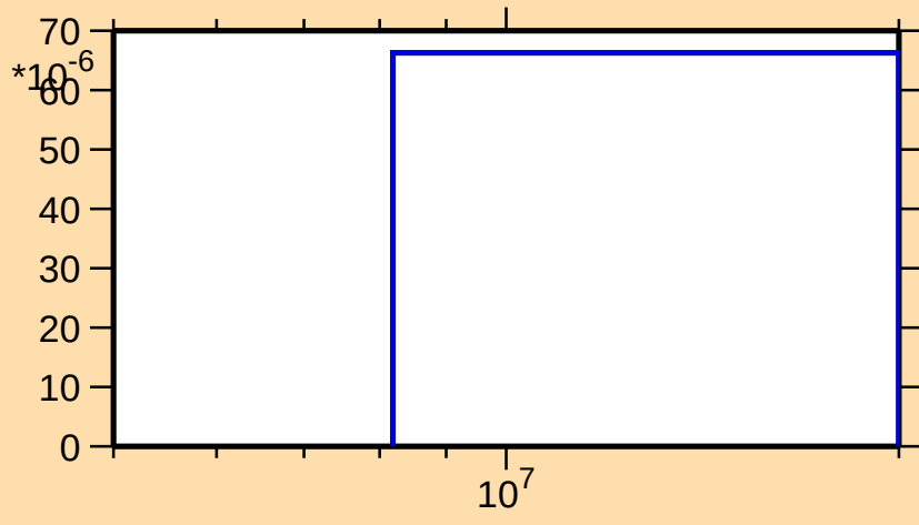
\sigma vs. E for ^{237}\text{Pu}(n,np)
