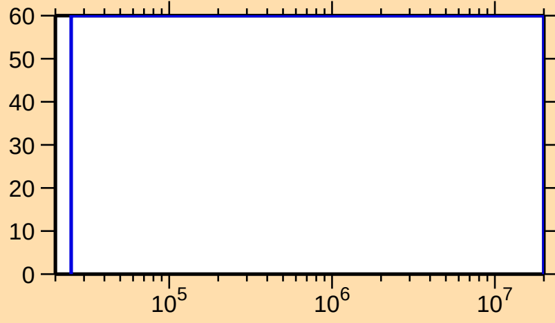
\Delta\sigma/\sigma vs. E for ^{237}\text{Pu}(n,n_1)
