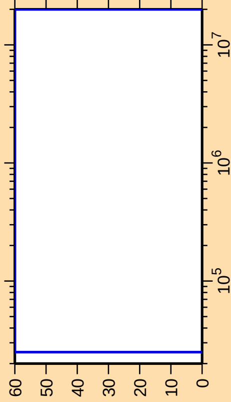
\Delta\sigma/\sigma vs. E for ^{237}\text{Pu}(n,n_1)
