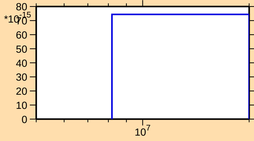
\sigma vs. E for ^{237}\text{Pu}(n,p\alpha)
