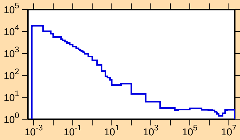
\sigma vs. E for ^{237}\text{Pu}(n,f)
