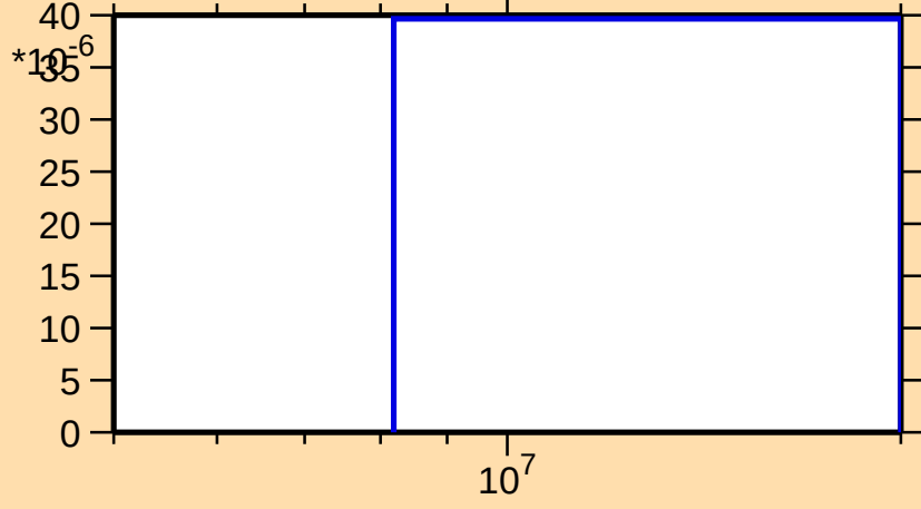
\sigma vs. E for ^{237}\text{Pu}(n,t)
