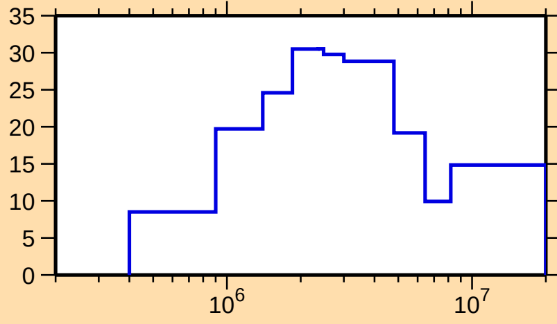
\Delta\sigma/\sigma vs. E for ^{237}\text{Pu}(n,\text{tot.})
