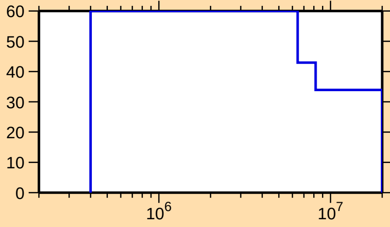
\Delta\sigma/\sigma vs. E for ^{237}\text{Pu}(n,n\text{cont.})
