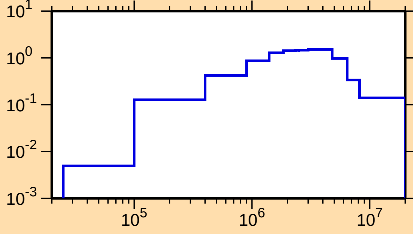
\sigma vs. E for ^{237}\text{Pu}(n,\text{inel.})
