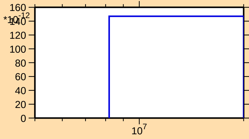
\sigma vs. E for ^{237}\text{Pu}(n,nt)
