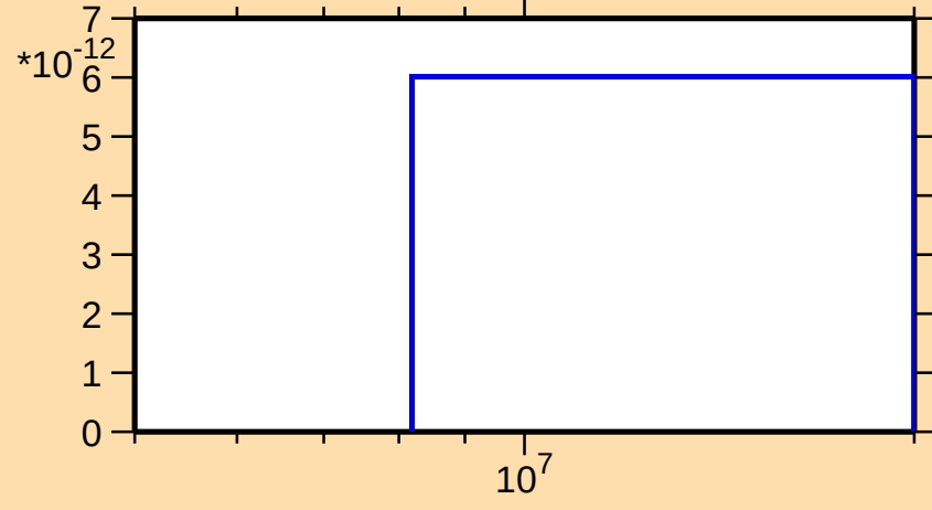
\sigma vs. E for ^{237}\text{Pu}(n,\text{He3})
