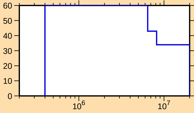
\Delta\sigma/\sigma vs. E for ^{237}\text{Pu}(n,n\text{cont.})
