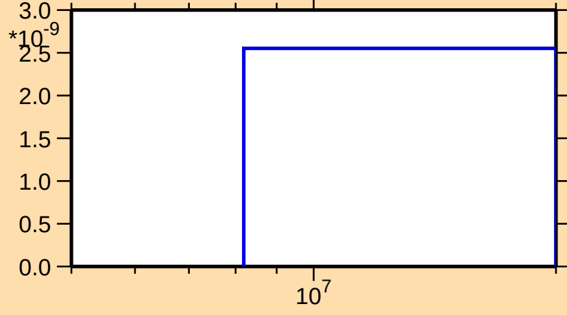
\sigma vs. E for ^{237}\text{Pu}(n,2np)
