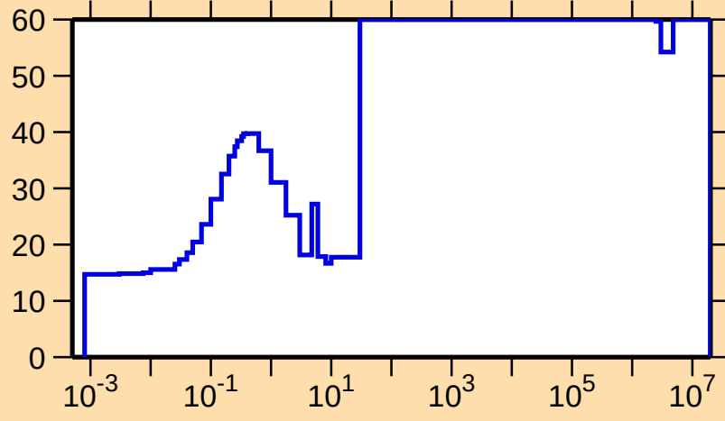
\Delta\sigma/\sigma vs. E for ^{237}\text{Pu}(n,\gamma)
