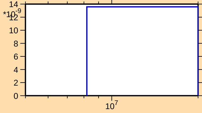
\sigma vs. E for ^{237}\text{Pu}(n,\text{nd})
