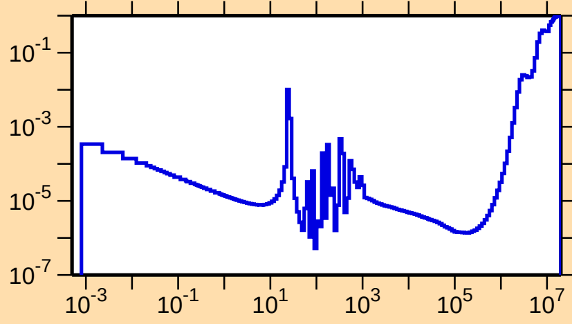
\sigma vs. E for ^{246}\text{Pu}(n,f)
