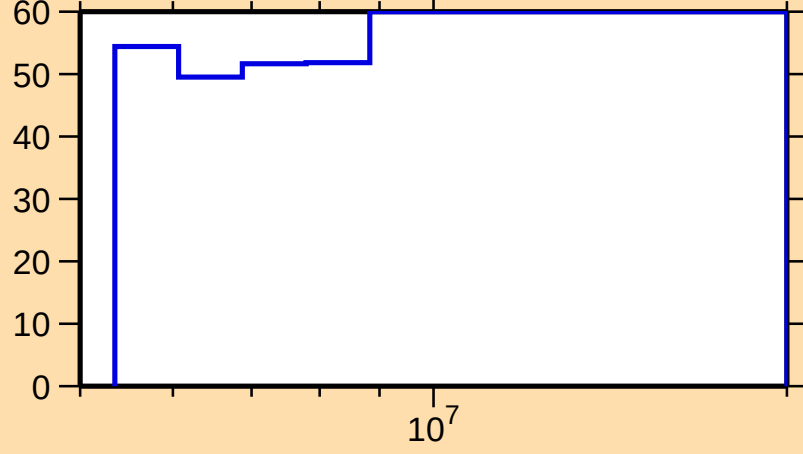
\Delta\sigma/\sigma vs. E for ^{246}\text{Pu}(n,\text{inel.})
