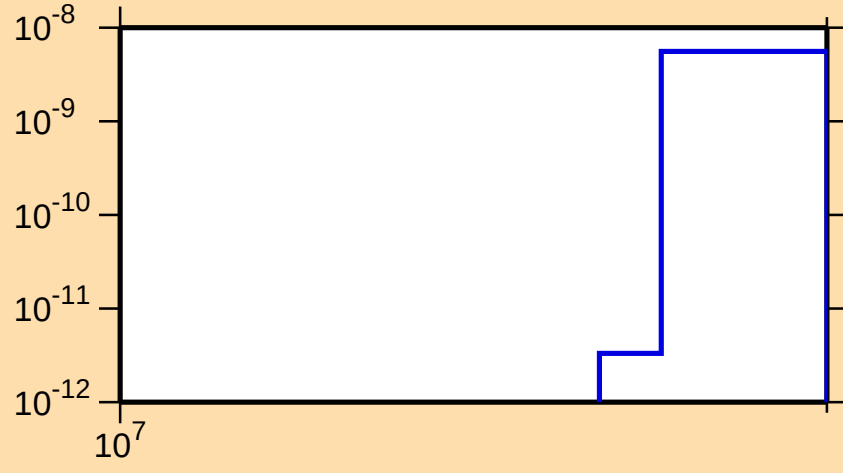
\sigma vs. E for ^{246}\text{Pu}(n,2np)
