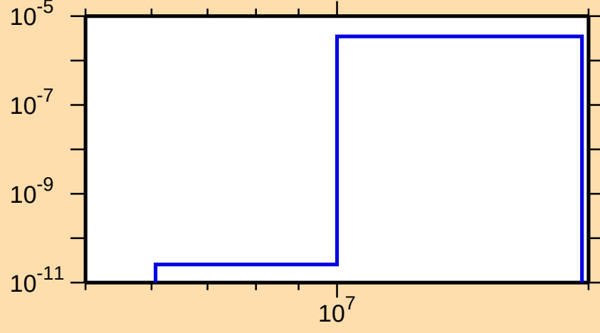
\sigma vs. E for ^{246}\text{Pu}(n,n\alpha)
