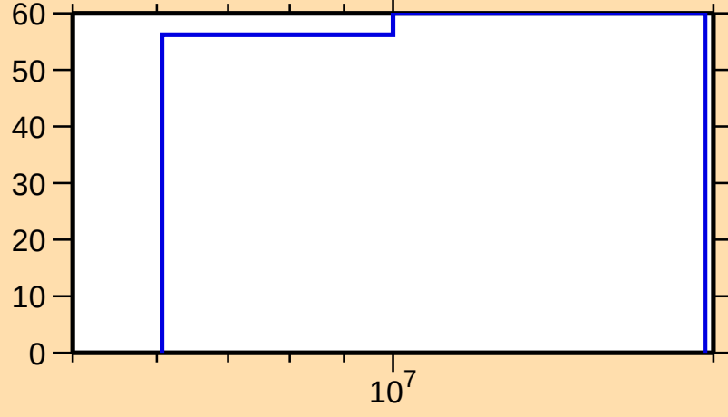
\Delta\sigma/\sigma vs. E for ^{246}\text{Pu}(n,\text{ncont.})
