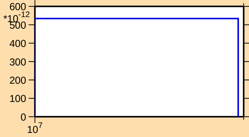
\sigma vs. E for ^{246}\text{Pu}(n,\text{nd})
