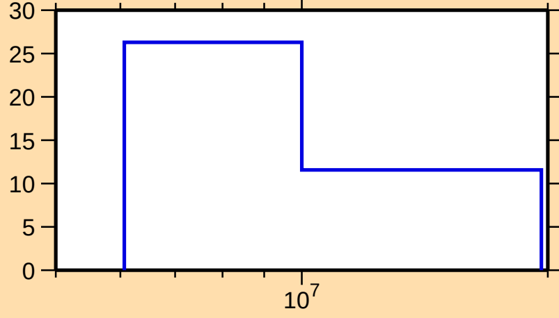
\Delta\sigma/\sigma vs. E for ^{246}\text{Pu}(n,\text{tot.})
