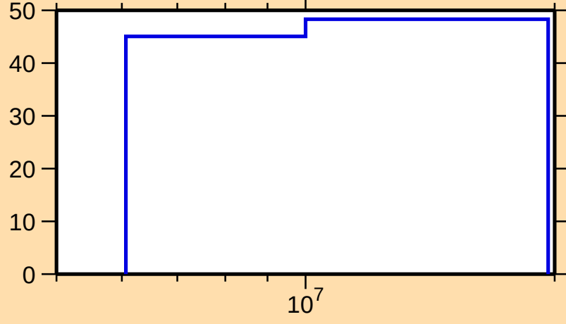
\Delta\sigma/\sigma vs. E for ^{246}\text{Pu}(n,\text{nonel.})
