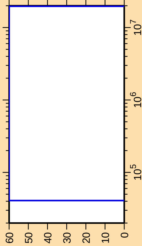
\Delta\sigma/\sigma vs. E for ^{246}\text{Pu}(n,n_1)
