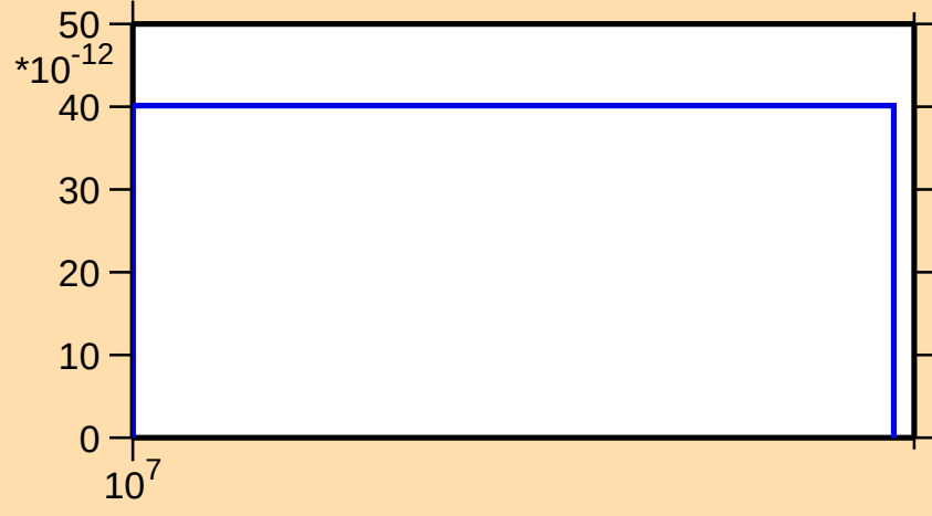
\sigma vs. E for ^{246}\text{Pu}(n,2np)
