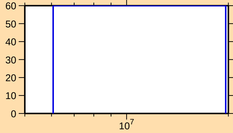
\Delta\sigma/\sigma vs. E for ^{246}\text{Pu}(n,\gamma)
