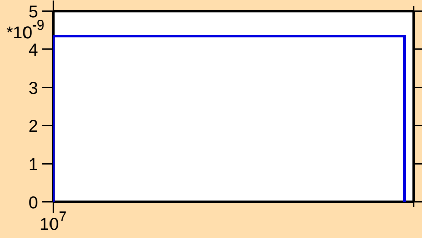
\sigma vs. E for ^{246}\text{Pu}(n,nt)
