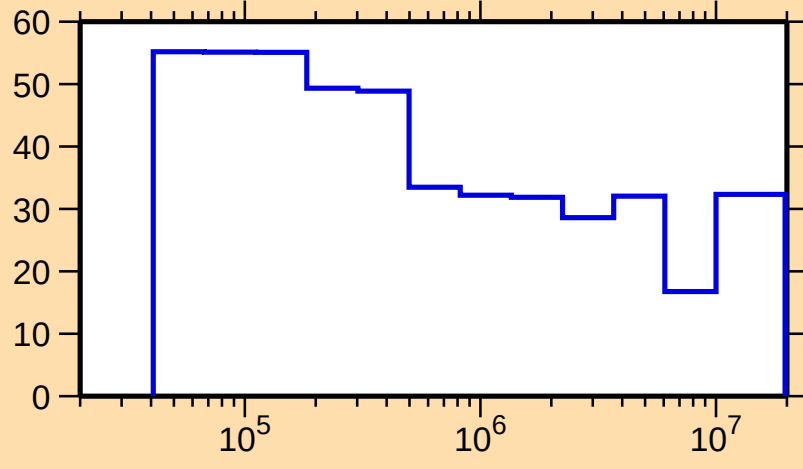
\Delta\sigma/\sigma vs. E for ^{246}\text{Pu}(n,\text{el.})
