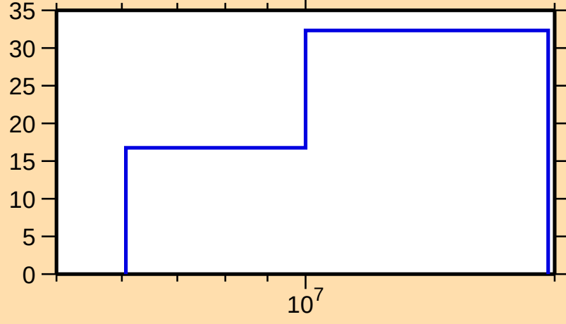
\Delta\sigma/\sigma vs. E for ^{246}\text{Pu}(n,\text{el.})
