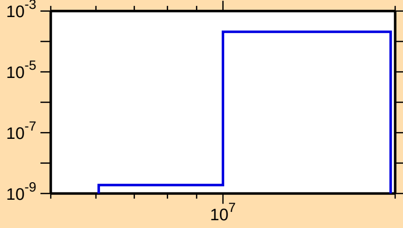
\sigma vs. E for ^{246}\text{Pu}(n,p)
