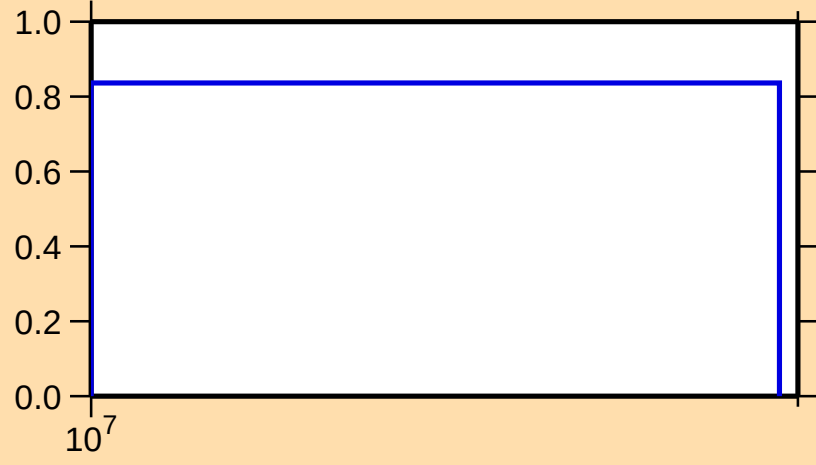
\sigma vs. E for ^{246}\text{Pu}(n,3n)
