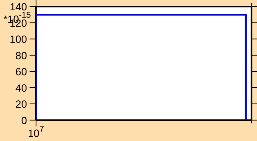
\sigma vs. E for ^{246}\text{Pu}(n,3n\alpha)
