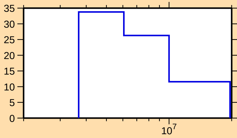
\Delta\sigma/\sigma vs. E for ^{246}\text{Pu}(n,\text{tot.})
