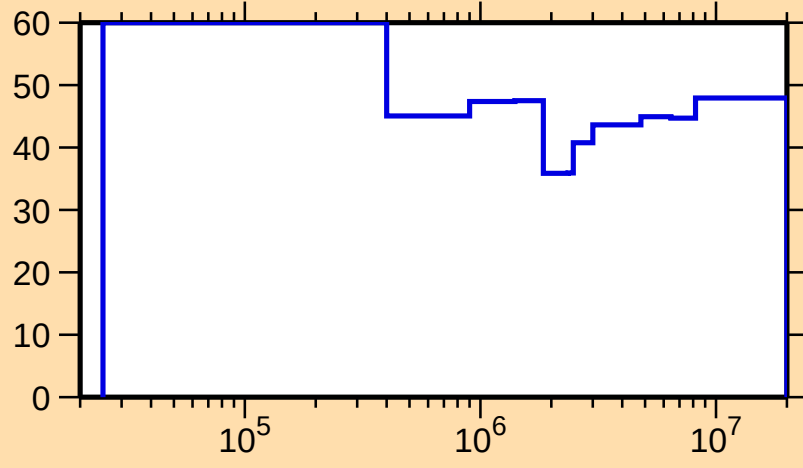
\Delta\sigma/\sigma vs. E for ^{246}\text{Pu}(n,\text{nonel.})
