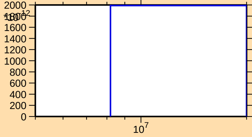
\sigma vs. E for ^{246}\text{Pu}(n,2n\alpha)
