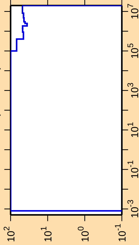
\Delta\sigma/\sigma vs. E for ^{246}\text{Pu}(n,\text{nonel.})
