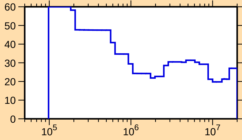
\Delta\sigma/\sigma vs. E for ^{247}\text{Pu}(n,\text{tot.})
