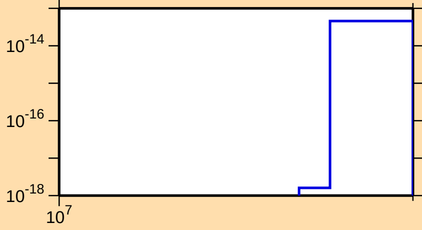
\sigma vs. E for ^{247}\text{Pu}(n,\text{He3})
