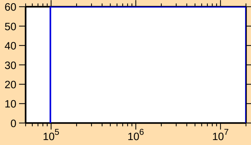
\Delta\sigma/\sigma vs. E for ^{247}\text{Pu}(n,n_1)
