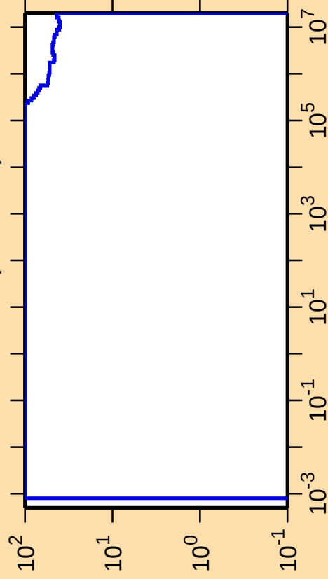
\Delta\sigma/\sigma vs. E for ^{247}\text{Pu}(n,\text{nonel.})
