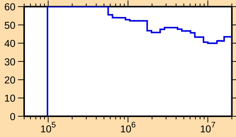
\Delta\sigma/\sigma vs. E for ^{247}\text{Pu}(n,\text{nonel.})
