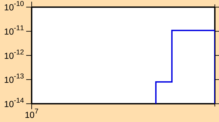
\sigma vs. E for ^{247}\text{Pu}(n,3n\alpha)
