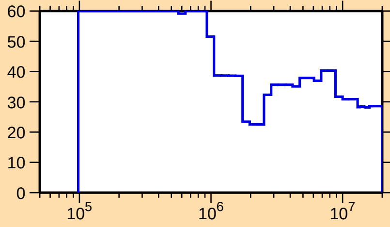
\Delta\sigma/\sigma vs. E for ^{247}\text{Pu}(n,\text{el.})
