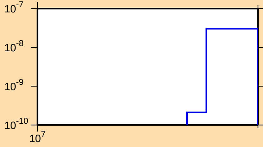
\sigma vs. E for ^{247}\text{Pu}(n,2np)
