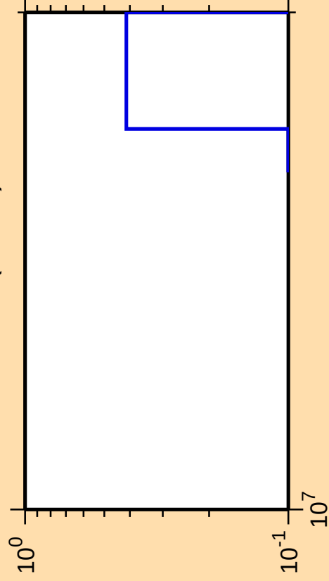
\Delta\sigma/\sigma vs. E for ^{247}\text{Pu}(n,\text{He3})
