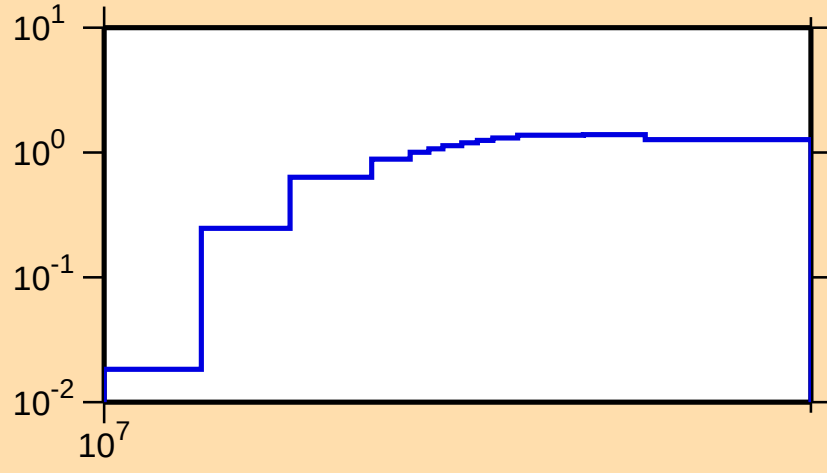
\sigma vs. E for ^{247}\text{Pu}(n,3n)
