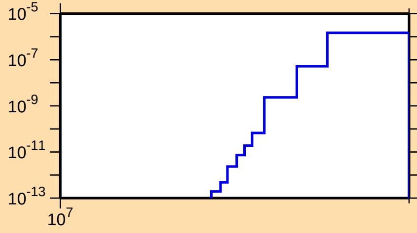
\sigma vs. E for ^{247}\text{Pu}(n,nt)
