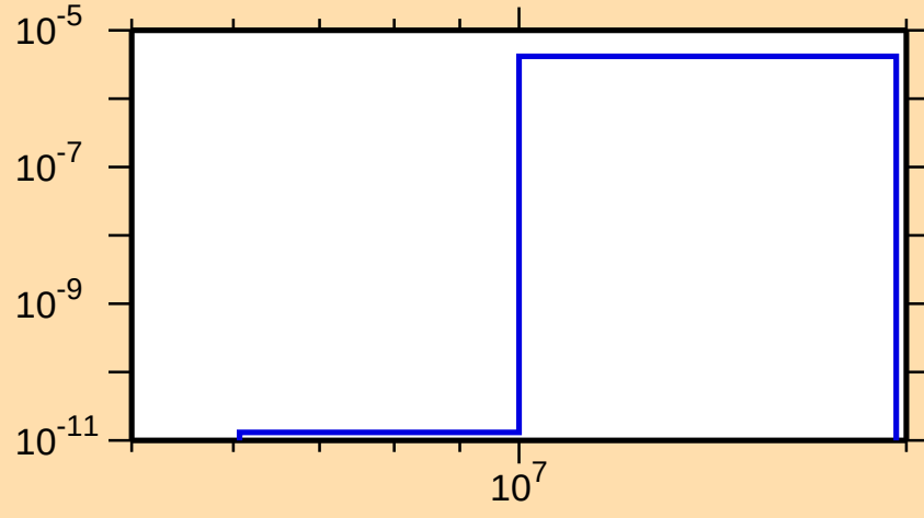
\sigma vs. E for ^{247}\text{Pu}(n,n\alpha)
