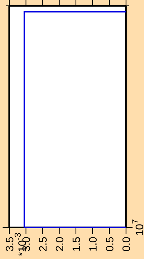
\Delta\sigma/\sigma vs. E for ^{247}\text{Pu}(n,\text{He3})
