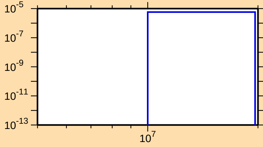
\sigma vs. E for ^{247}\text{Pu}(n,np)
