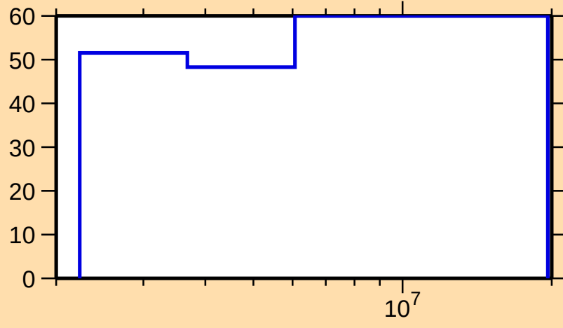
\Delta\sigma/\sigma vs. E for ^{247}\text{Pu}(n,\text{inel.})
