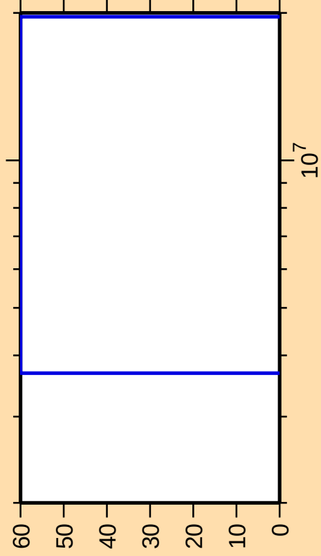
\Delta\sigma/\sigma vs. E for ^{247}\text{Pu}(n,f)
