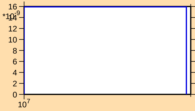
\sigma vs. E for ^{247}\text{Pu}(n,nt)
