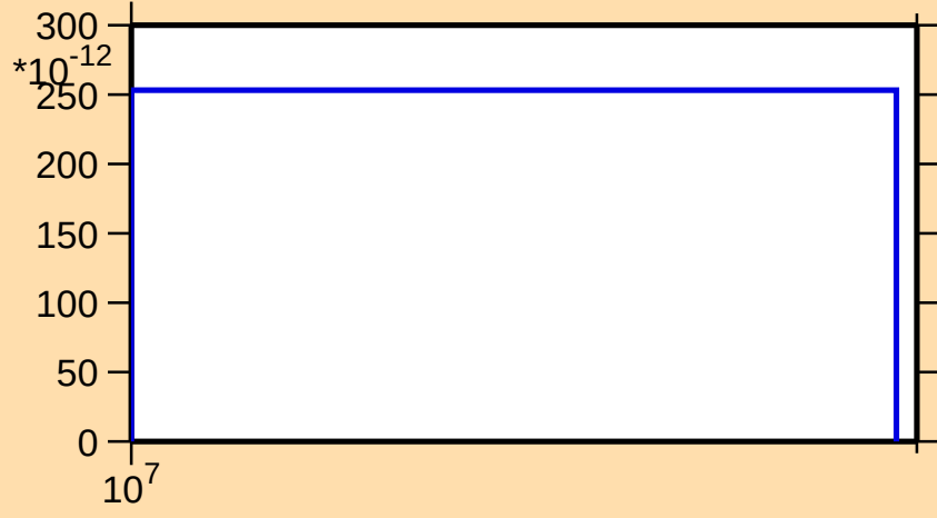
\sigma vs. E for ^{247}\text{Pu}(n,2np)
