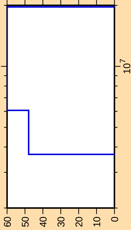
\Delta\sigma/\sigma vs. E for ^{247}\text{Pu}(n,n\text{cont.})
