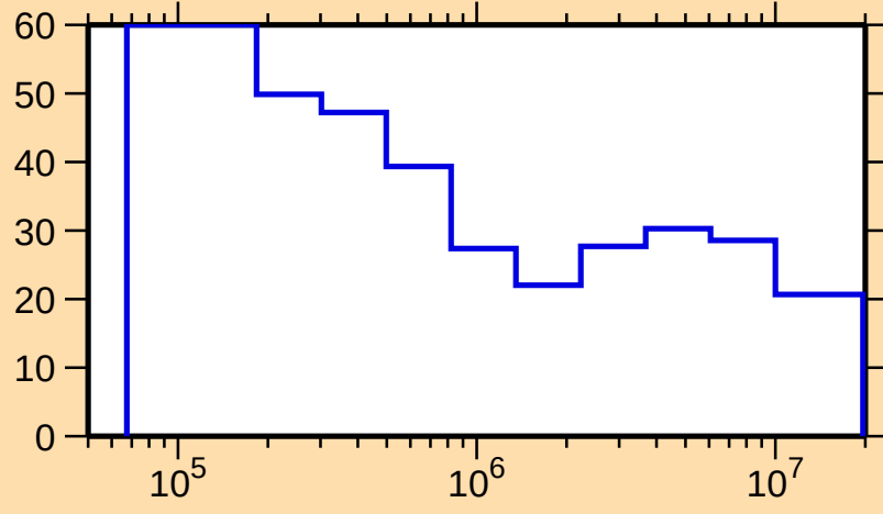
\Delta\sigma/\sigma vs. E for ^{247}\text{Pu}(n,\text{tot.})
