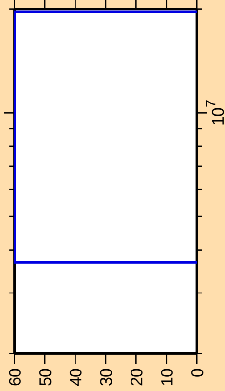
\Delta\sigma/\sigma vs. E for ^{247}\text{Pu}(n,\gamma)
