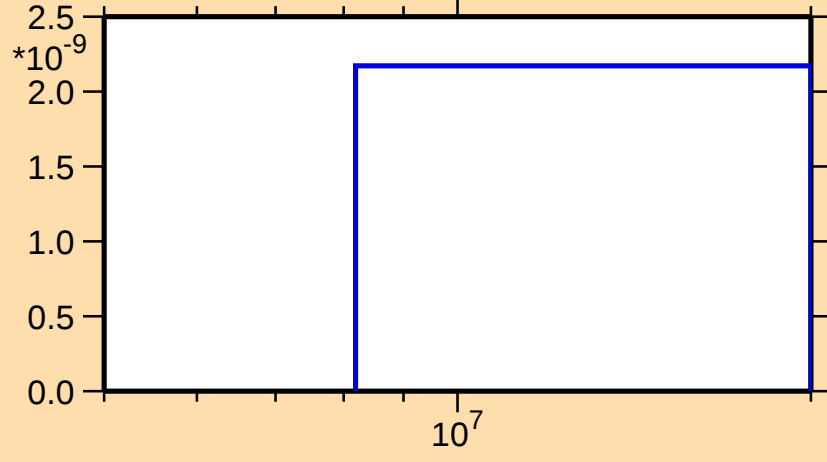
\sigma vs. E for ^{247}\text{Pu}(n,\text{nd})
