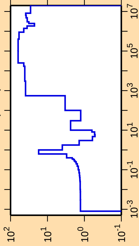
\Delta\sigma/\sigma vs. E for ^{247}\text{Pu}(n,\text{el.})
