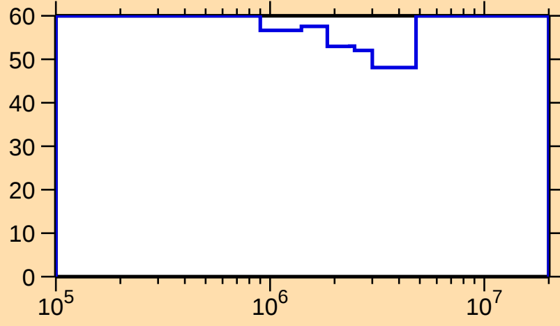
\Delta\sigma/\sigma vs. E for ^{247}\text{Pu}(n,n\text{cont.})
