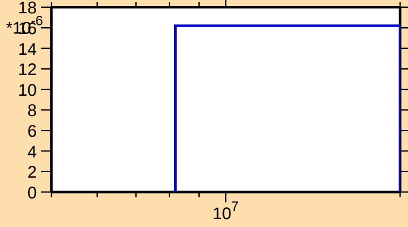
\sigma vs. E for ^{247}\text{Pu}(n,d)
