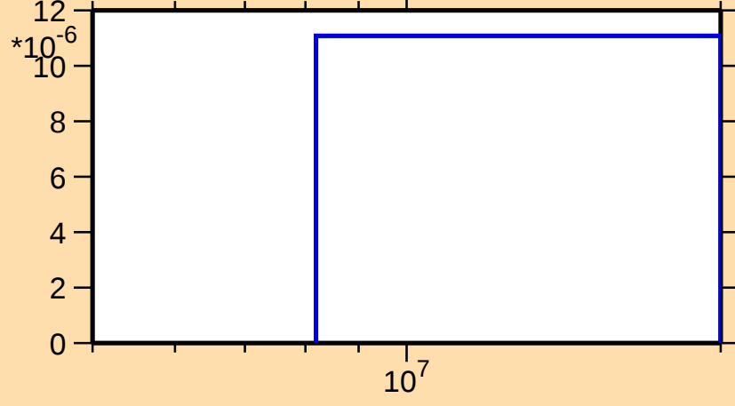
\sigma vs. E for ^{247}\text{Pu}(n,t)
