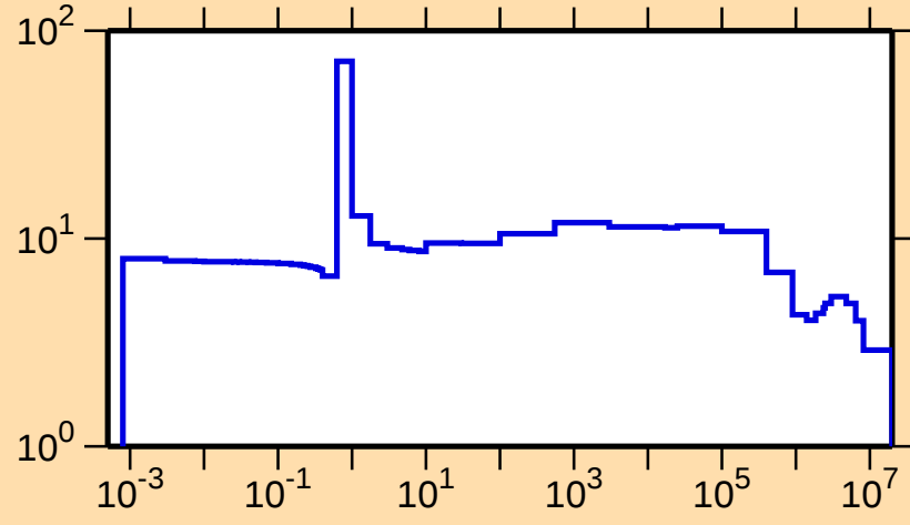
\sigma vs. E for ^{247}\text{Pu}(n,\text{el.})
