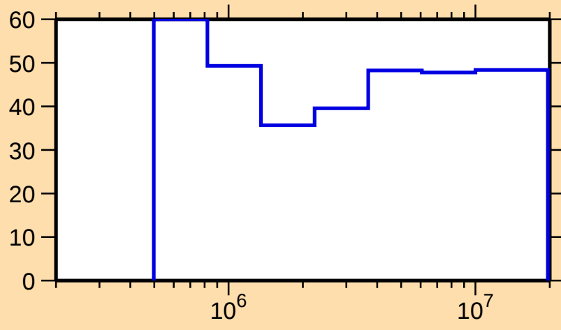
\Delta\sigma/\sigma vs. E for ^{207}\text{Ra}(n,n_1)
