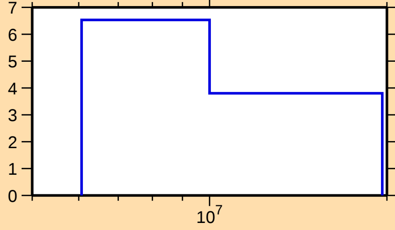
\Delta\sigma/\sigma vs. E for ^{207}\text{Ra}(n,\text{nonel.})
