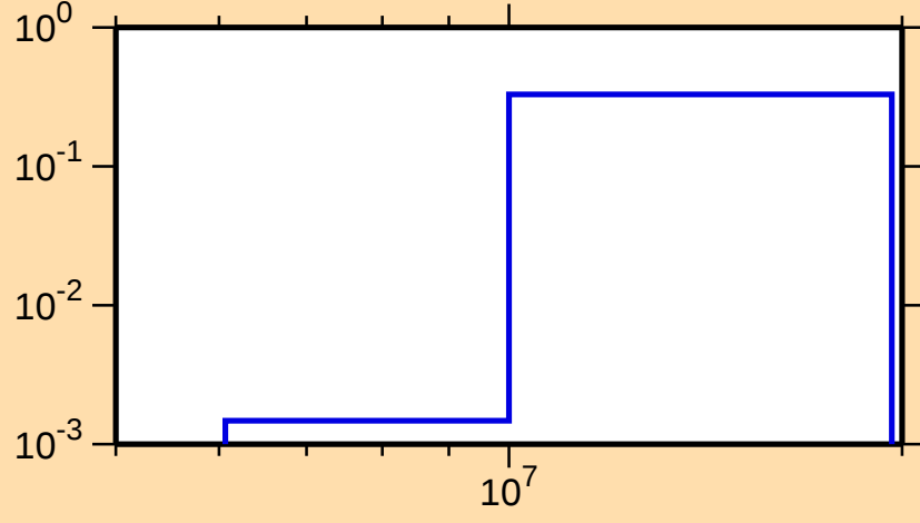
\sigma vs. E for ^{207}\text{Ra}(n,2n)
