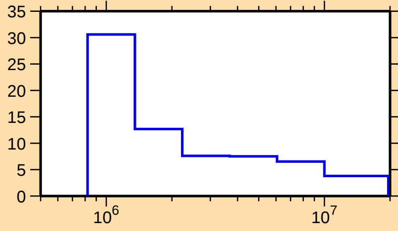
\Delta\sigma/\sigma vs. E for ^{207}\text{Ra}(n,n\text{nonel.})
