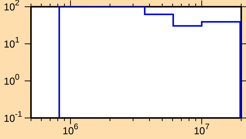
\Delta\sigma/\sigma vs. E for ^{207}\text{Ra}(n,n\text{cont.})
