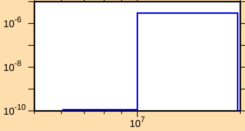
\sigma vs. E for ^{207}\text{Ra}(n,\text{He3})
