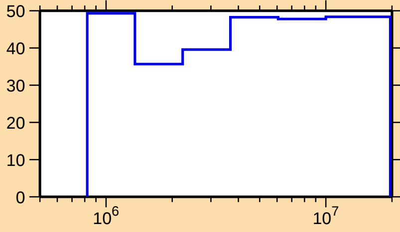
\Delta\sigma/\sigma vs. E for ^{207}\text{Ra}(n,n_1)
