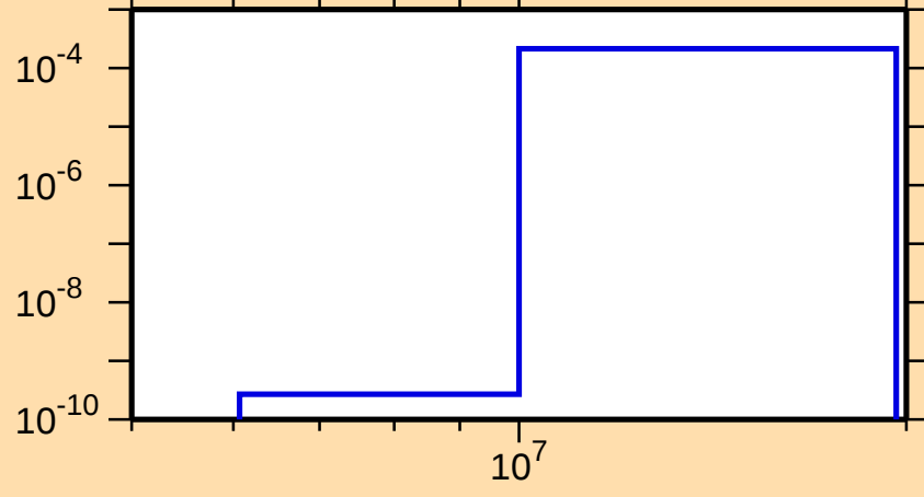
\sigma vs. E for ^{207}\text{Ra}(n,t)
