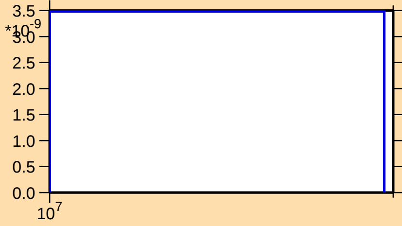
\sigma vs. E for ^{207}\text{Ra}(n,\text{pt})
