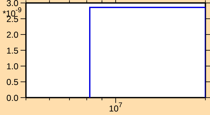
\sigma vs. E for ^{207}\text{Ra}(n,\text{pt})
