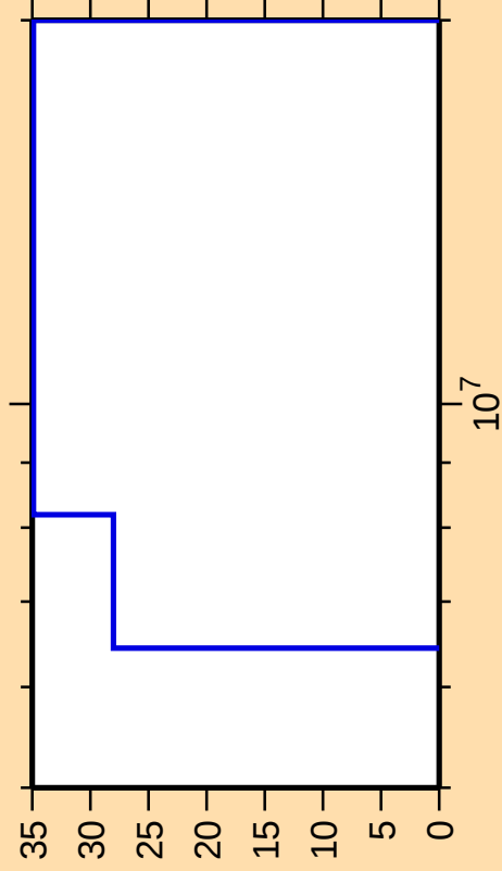
\Delta\sigma/\sigma vs. E for ^{207}\text{Ra}(n,n\text{cont.})
