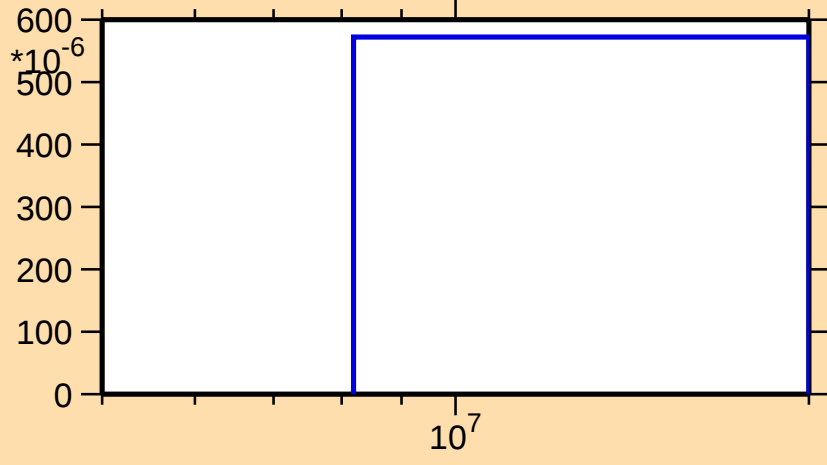
\sigma vs. E for ^{207}\text{Ra}(n,2n\alpha)
