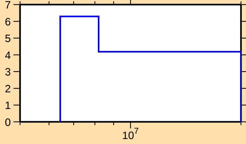
\Delta\sigma/\sigma vs. E for ^{207}\text{Ra}(n,\text{nonel.})
