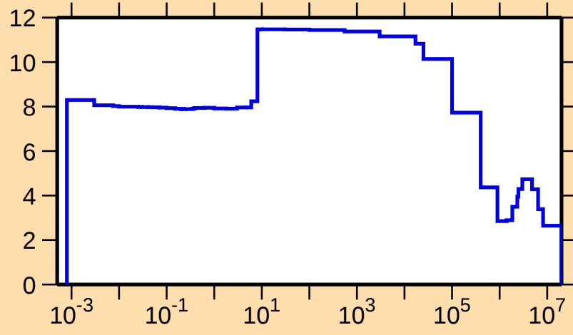
\sigma vs. E for ^{207}\text{Ra}(n,\text{el.})
