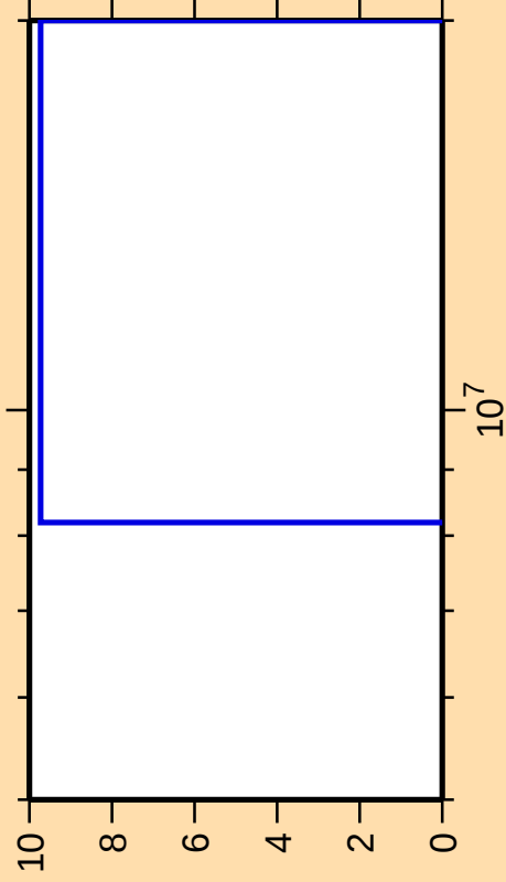
\Delta\sigma/\sigma vs. E for ^{207}\text{Ra}(n,nt)
