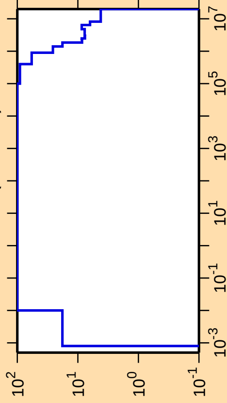
\Delta\sigma/\sigma vs. E for ^{207}\text{Ra}(n,\text{nonel.})
