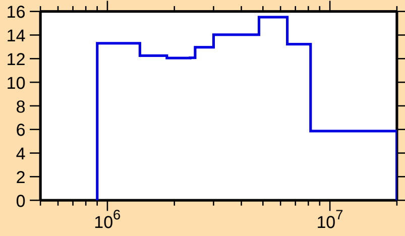
\Delta\sigma/\sigma vs. E for ^{207}\text{Ra}(n,\text{el.})
