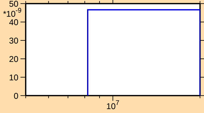
\sigma vs. E for ^{207}\text{Ra}(n,\text{pd})
