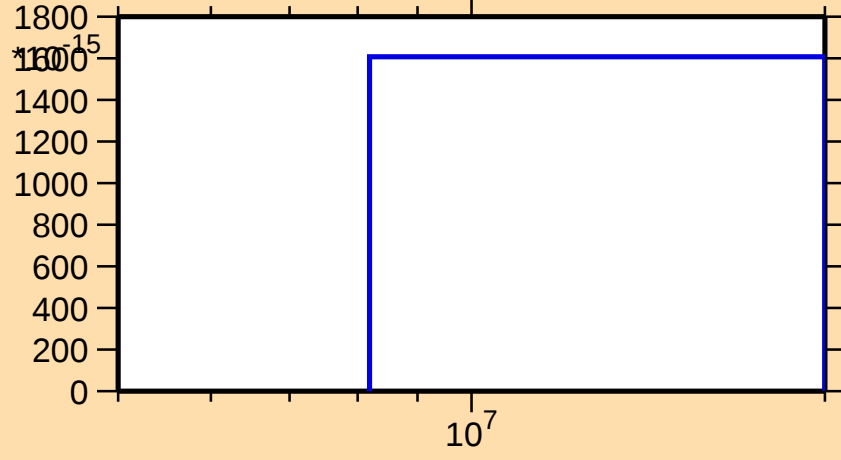
\sigma vs. E for ^{207}\text{Ra}(n,nt)
