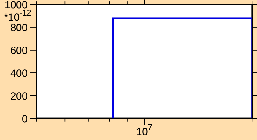
\sigma vs. E for ^{207}\text{Ra}(\text{mt117})
