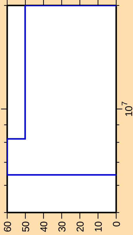
\Delta\sigma/\sigma vs. E for ^{207}\text{Ra}(n,p)
