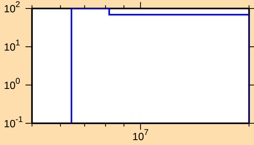
\Delta\sigma/\sigma vs. E for ^{207}\text{Ra}(n,2n)
