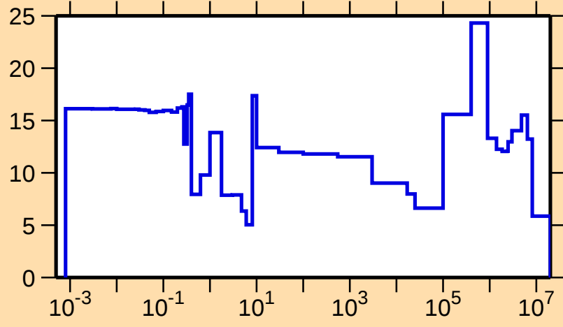
\Delta\sigma/\sigma vs. E for ^{207}\text{Ra}(n,\text{el.})
