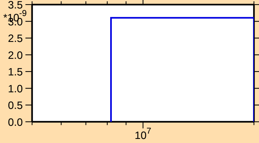
\sigma vs. E for ^{207}\text{Ra}(n,3n\alpha)
