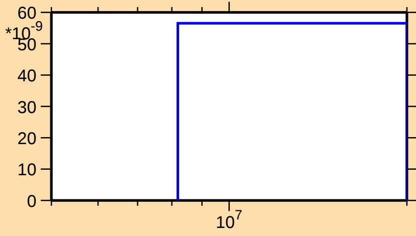
\sigma vs. E for ^{207}\text{Ra}(n,3n)
