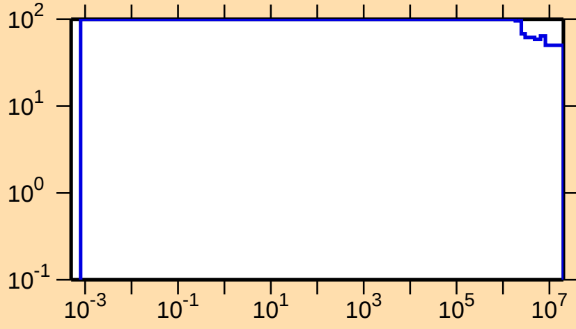
\Delta\sigma/\sigma vs. E for ^{207}\text{Ra}(n,p)
