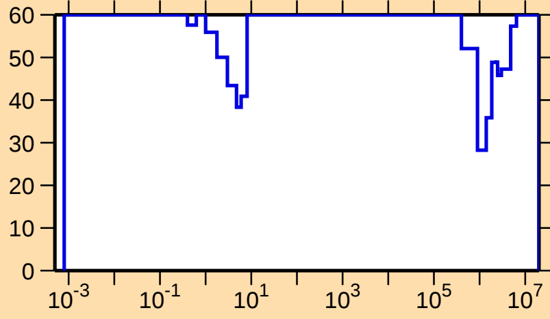
\Delta\sigma/\sigma vs. E for ^{207}\text{Ra}(n,\gamma)
