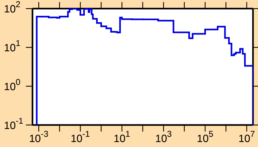
\Delta\sigma/\sigma vs. E for ^{207}\text{Ra}(n,\text{tot.})
