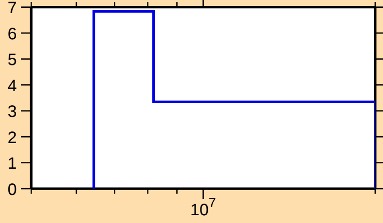
\Delta\sigma/\sigma vs. E for ^{207}\text{Ra}(n,\text{tot.})
