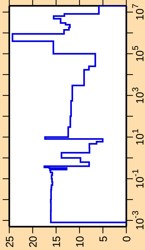
\Delta\sigma/\sigma vs. E for ^{207}\text{Ra}(n,\text{el.})
