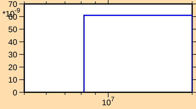
\sigma vs. E for ^{207}\text{Ra}(n,\text{nd})
