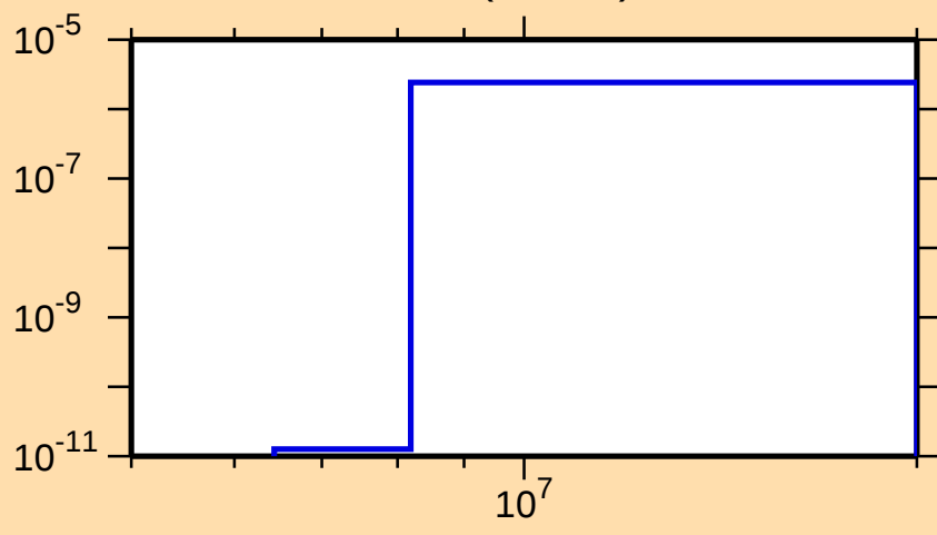
\sigma vs. E for ^{207}\text{Ra}(n,\text{He}3)
