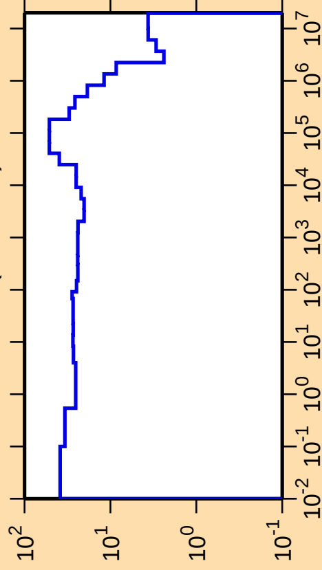
\Delta\sigma/\sigma vs. E for ^{78}\text{Rb}(n,\text{nonel.})
