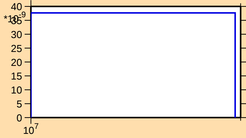
\sigma vs. E for ^{78}\text{Rb}(\text{mt } 45)
