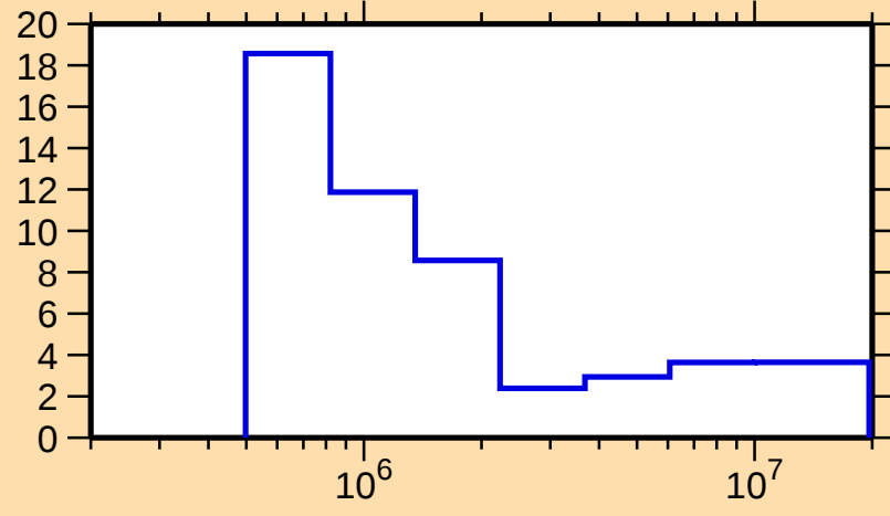
\Delta\sigma/\sigma vs. E for ^{78}\text{Rb}(n,n\text{nonel.})
