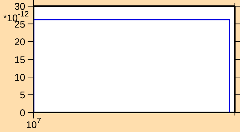
\sigma vs. E for ^{78}\text{Rb}(\text{mt } 34)
