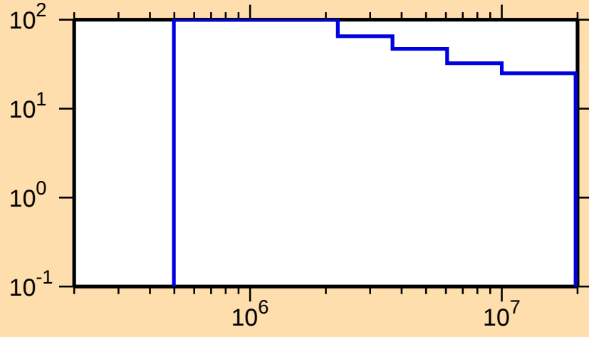
\Delta\sigma/\sigma vs. E for ^{78}\text{Rb}(n,n\text{cont.})
