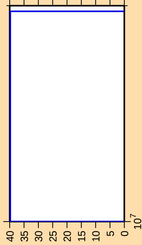
\Delta\sigma/\sigma vs. E for ^{78}\text{Rb}(\text{mt } 45)
