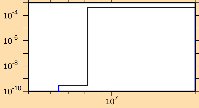
\sigma vs. E for ^{78}\text{Rb}(n,t)
