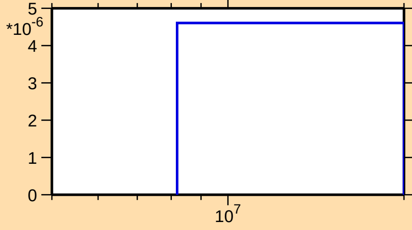
\sigma vs. E for ^{78}\text{Rb}(n,\text{pd})
