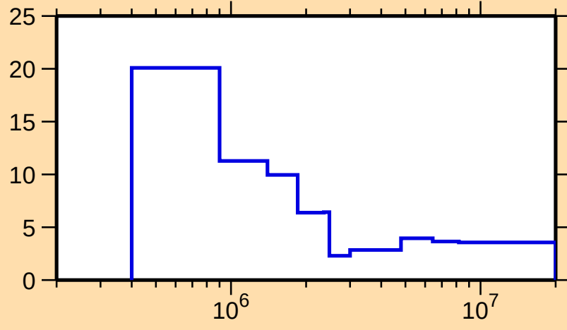
\Delta\sigma/\sigma vs. E for ^{78}\text{Rb}(n,n\text{nonel.})
