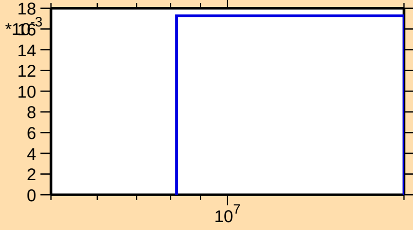
\sigma vs. E for ^{78}\text{Rb}(n,2n)
