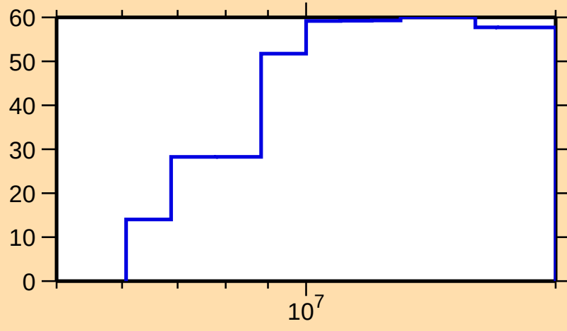
\Delta\sigma/\sigma vs. E for ^{88}\text{Rb}(n,\text{inel.})
