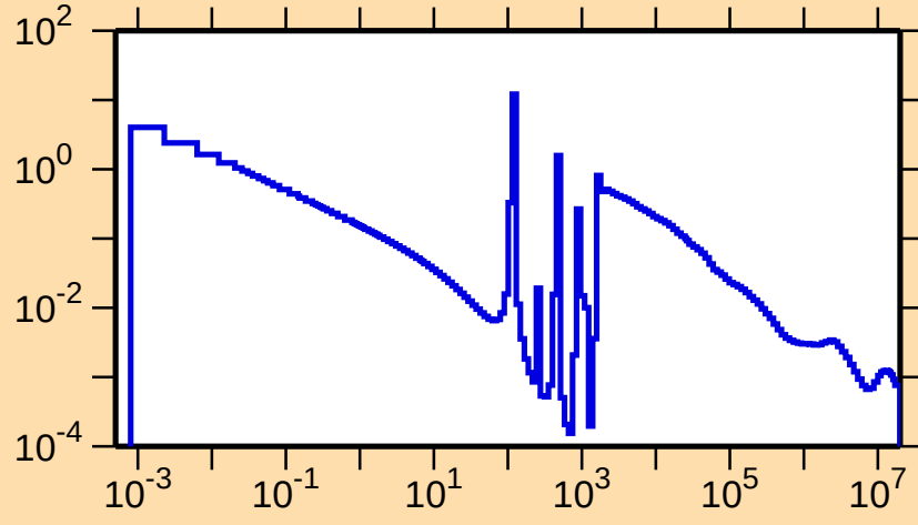
\sigma vs. E for ^{88}\text{Rb}(n,\gamma)
