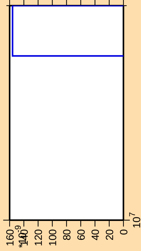
\Delta\sigma/\sigma vs. E for ^{88}\text{Rb} (mt 34)
