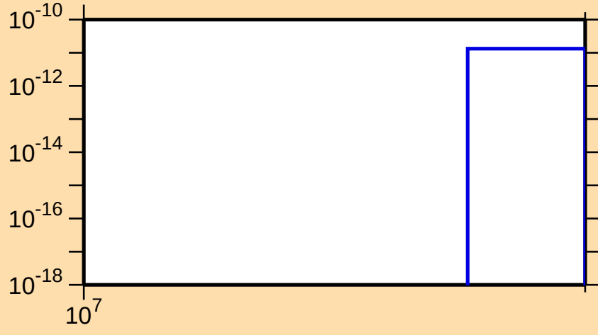
\sigma vs. E for ^{88}\text{Rb}(n,2n\alpha)
