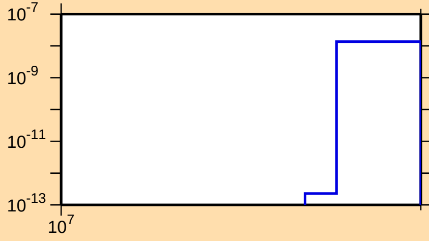
\sigma vs. E for ^{88}\text{Rb}(n,nt)
