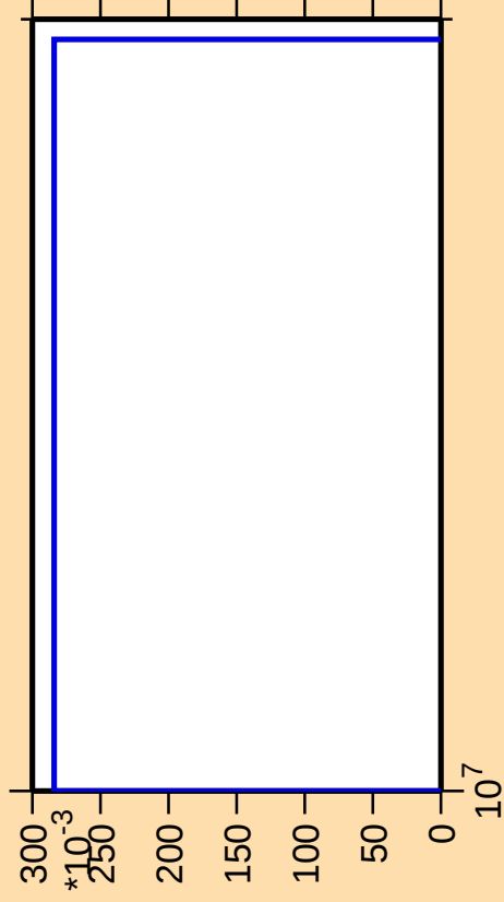
\Delta\sigma/\sigma vs. E for ^{88}\text{Rb}(n,2n\alpha)
