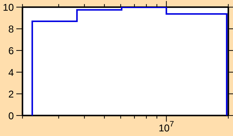
\Delta\sigma/\sigma vs. E for ^{88}\text{Rb}(n,n\text{nonel.})
