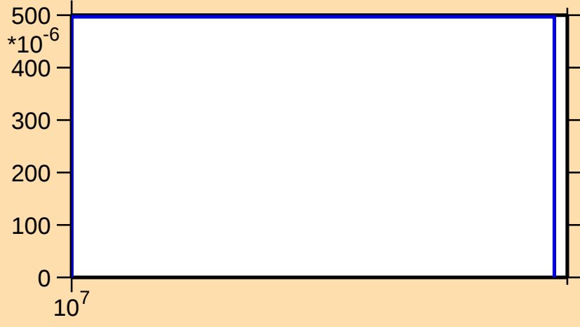
\sigma vs. E for ^{88}\text{Rb}(n,3n)
