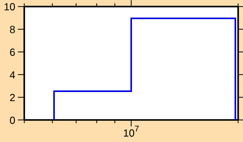
\Delta\sigma/\sigma vs. E for ^{88}\text{Rb}(n,\text{tot.})
