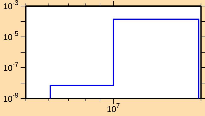
\sigma vs. E for ^{88}\text{Rb}(n,t)
