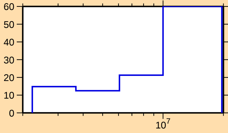
\Delta\sigma/\sigma vs. E for ^{88}\text{Rb}(n,n\text{cont.})
