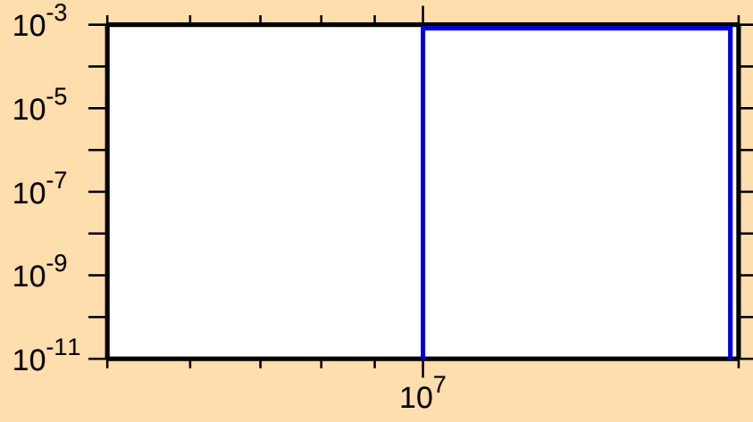
\sigma vs. E for ^{88}\text{Rb}(n,np)
