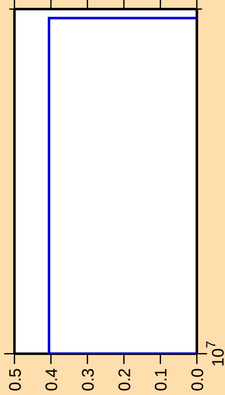
\Delta\sigma/\sigma vs. E for ^{88}\text{Rb}(n,p\alpha)
