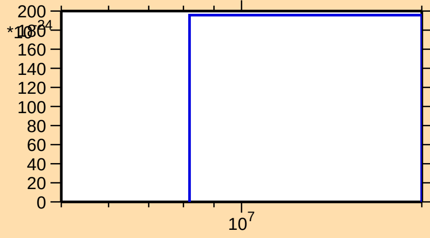
\sigma vs. E for ^{88}\text{Rb}(\text{mt } 34)
