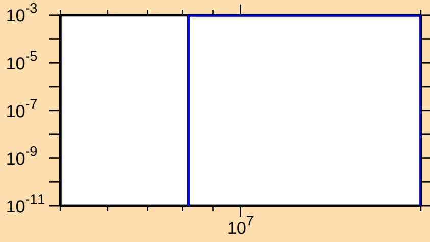
\sigma vs. E for ^{88}\text{Rb}(n,d)
