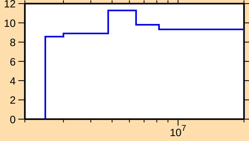
\Delta\sigma/\sigma vs. E for ^{88}\text{Rb}(n,\text{nonel.})
