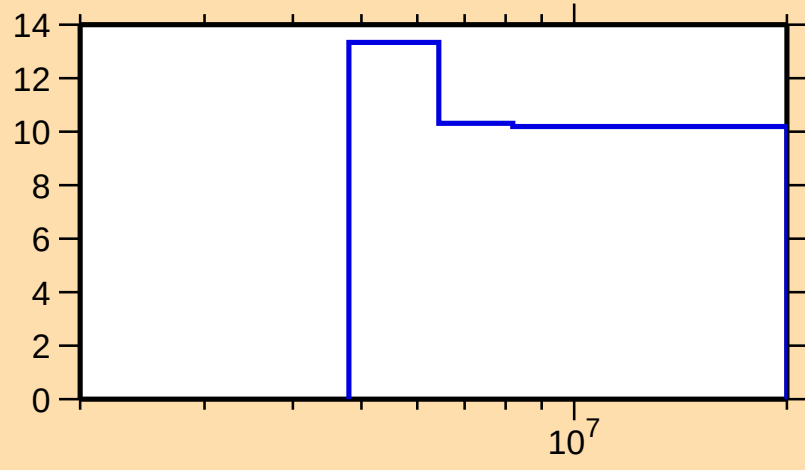
\Delta\sigma/\sigma vs. E for ^{88}\text{Rb}(n,\text{el.})
