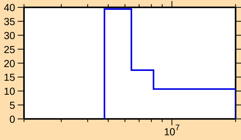
\Delta\sigma/\sigma vs. E for ^{88}\text{Rb}(n,2n)
