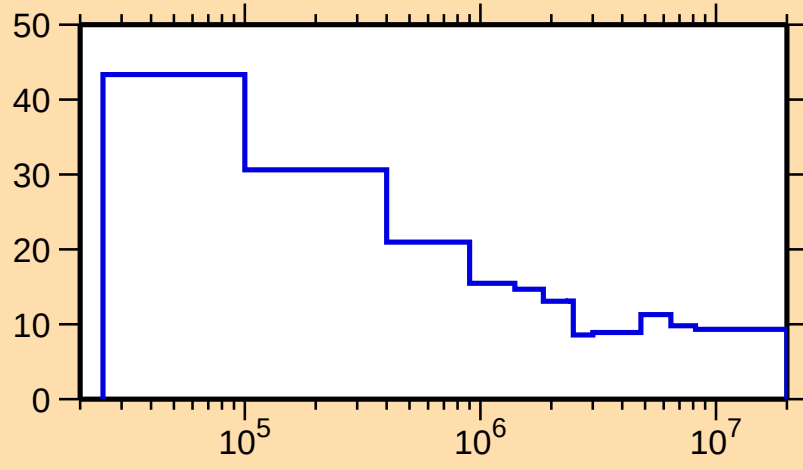
\Delta\sigma/\sigma vs. E for ^{88}\text{Rb}(n,\text{nonel.})
