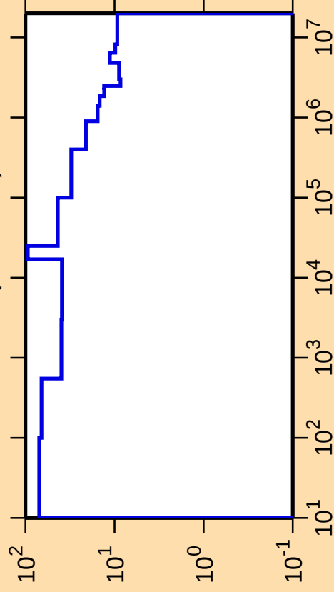
\Delta\sigma/\sigma vs. E for ^{88}\text{Rb}(n,\text{nonel.})
