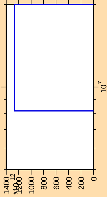
\Delta\sigma/\sigma vs. E for ^{88}\text{Rb}(\text{mt } 34)
