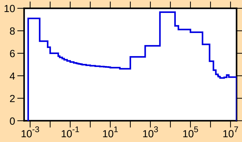
\sigma vs. E for ^{88}\text{Rb}(n,\text{tot.})
