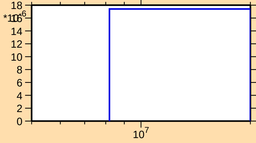
\sigma vs. E for ^{88}\text{Rb}(n,n\alpha)
