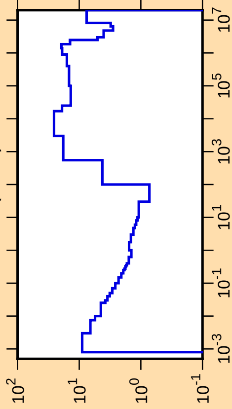
\Delta\sigma/\sigma vs. E for ^{88}\text{Rb}(n,\text{tot.})
