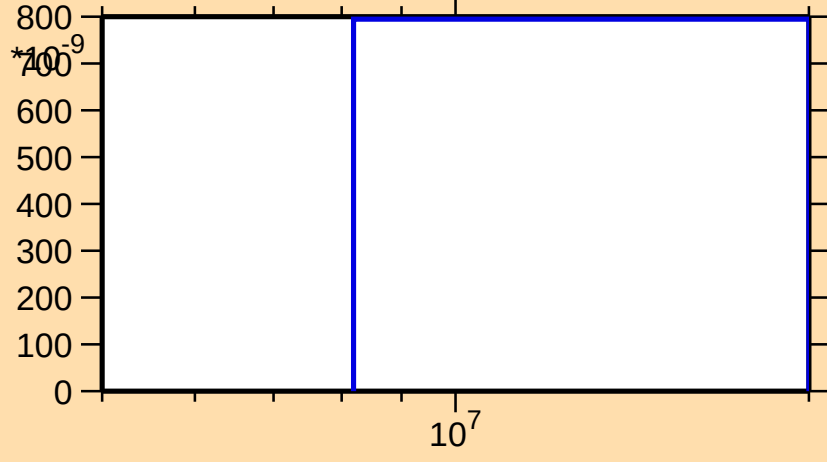
\sigma vs. E for ^{88}\text{Rb}(n,\text{nd})
