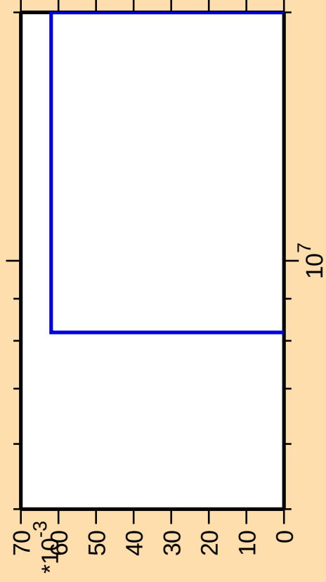
\Delta\sigma/\sigma vs. E for ^{88}\text{Rb}(n,\text{He}3)
