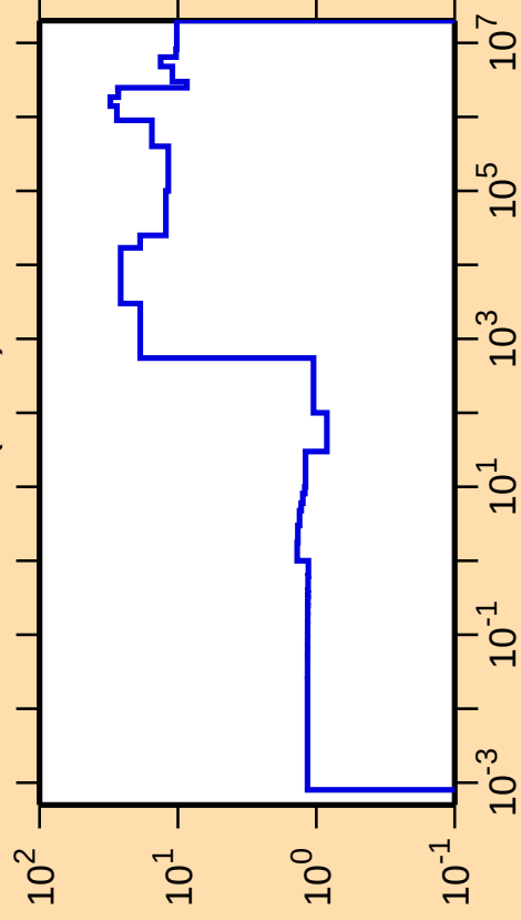
\Delta\sigma/\sigma vs. E for ^{88}\text{Rb}(n,\text{el.})
