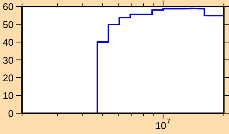
\Delta\sigma/\sigma vs. E for ^{92}\text{Rb}(n,n_1)
