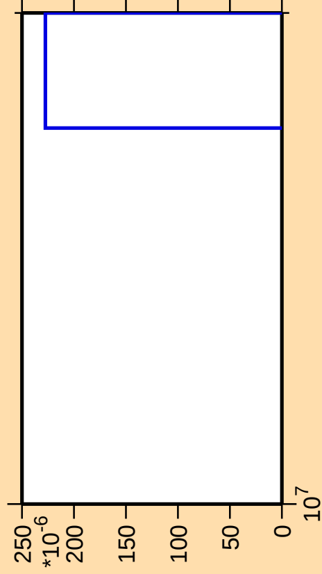
\Delta\sigma/\sigma vs. E for ^{92}\text{Rb}(\text{mt 11})
