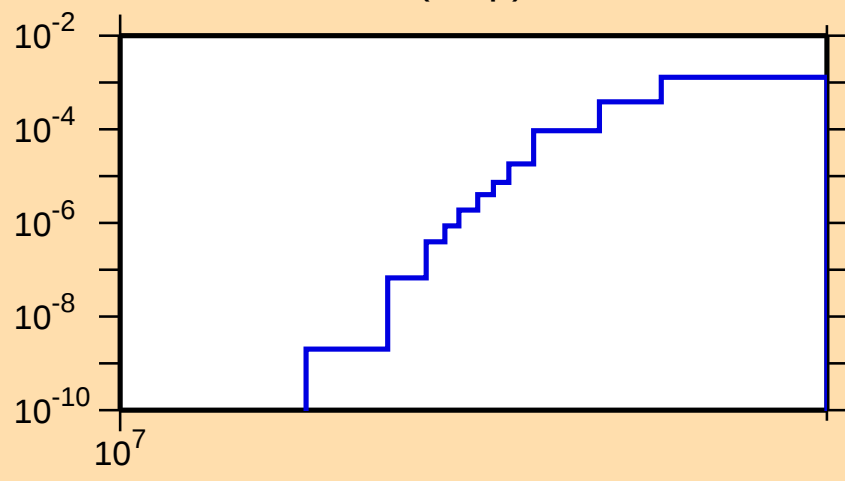
\sigma vs. E for ^{92}\text{Rb}(n,np)
