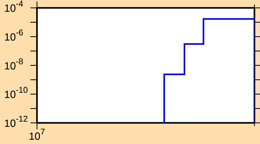
\sigma vs. E for ^{92}\text{Rb}(n,nt)
