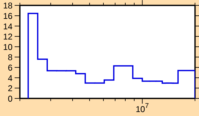
\Delta\sigma/\sigma vs. E for ^{92}\text{Rb}(n,n\text{nonel.})
