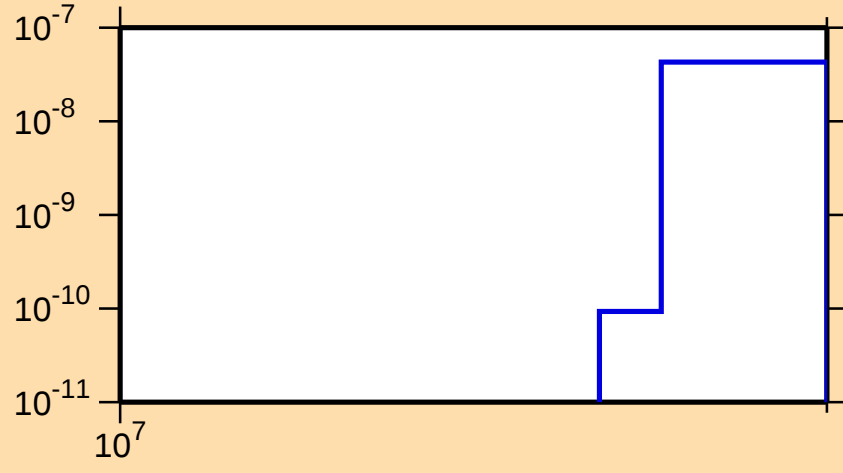
\sigma vs. E for ^{92}\text{Rb}(n,2n\alpha)
