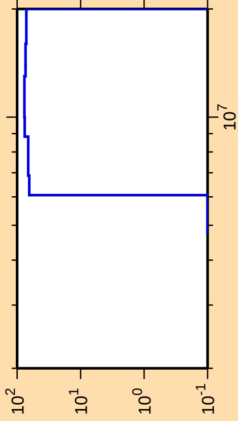
\Delta\sigma/\sigma vs. E for ^{92}\text{Rb}(n,p)
