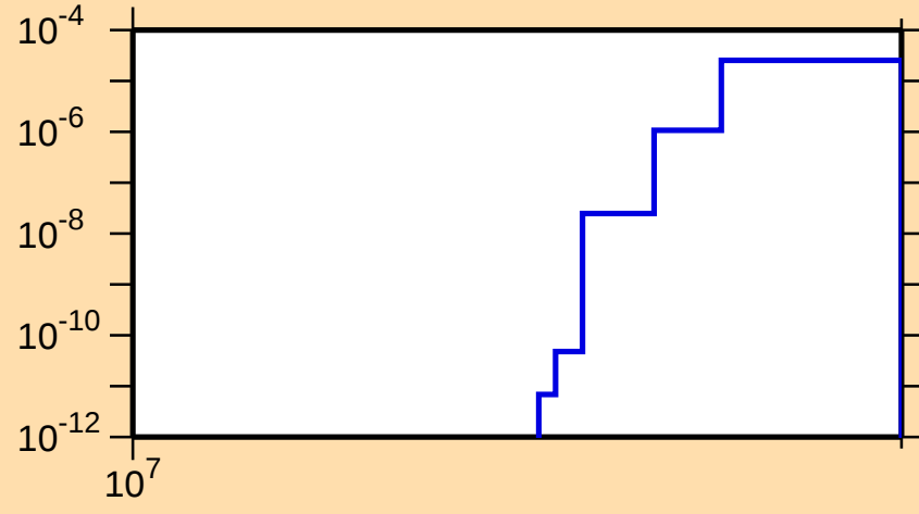
\sigma vs. E for ^{92}\text{Rb}(n,\text{nd})
