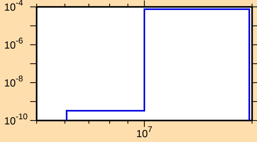
\sigma vs. E for ^{92}\text{Rb}(n,t)
