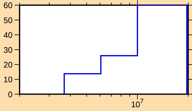
\Delta\sigma/\sigma vs. E for ^{92}\text{Rb}(n,n\text{cont.})
