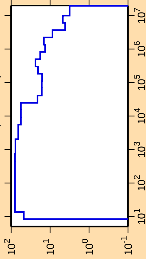
\Delta\sigma/\sigma vs. E for ^{92}\text{Rb}(n,\text{nonel.})
