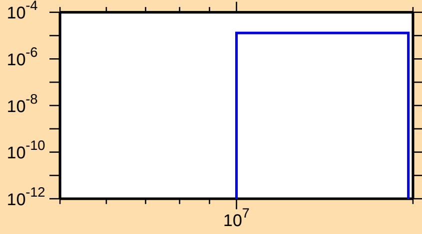
\sigma vs. E for ^{92}\text{Rb}(n,n\alpha)
