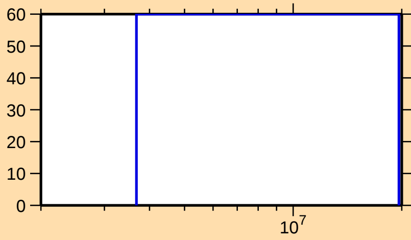
\Delta\sigma/\sigma vs. E for ^{92}\text{Rb}(n,\gamma)
