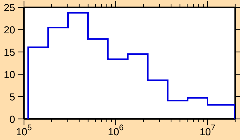
\Delta\sigma/\sigma vs. E for ^{92}\text{Rb}(n,\text{nonel.})
