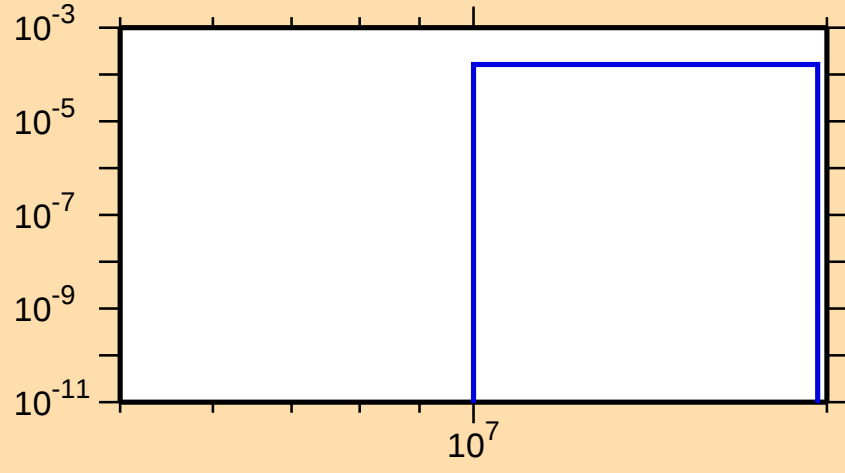
\sigma vs. E for ^{92}\text{Rb}(n,d)
