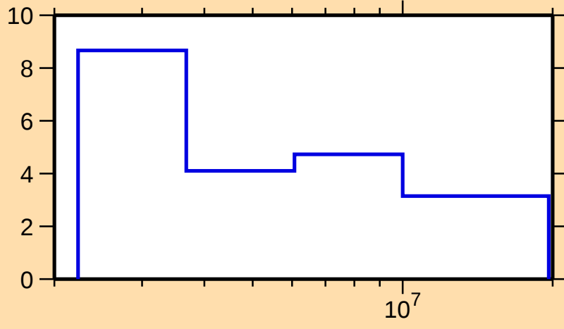
\Delta\sigma/\sigma vs. E for ^{92}\text{Rb}(n,n\text{oncl.})
