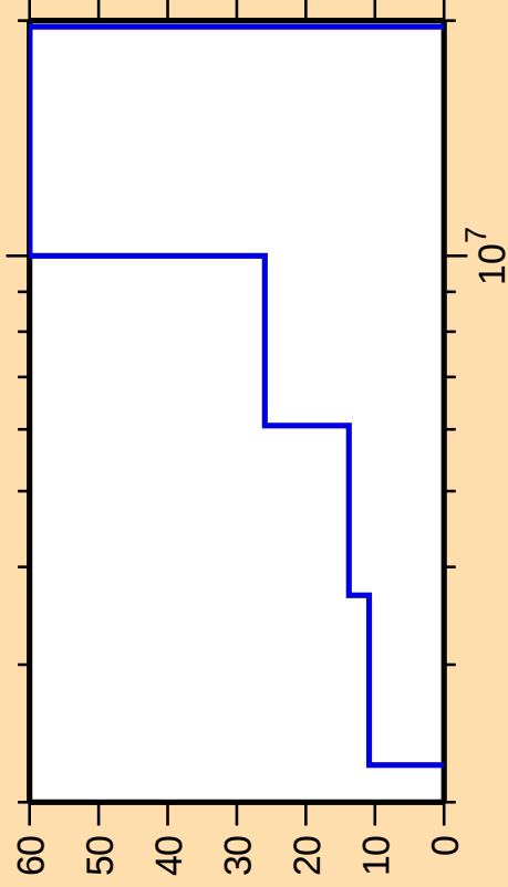
\Delta\sigma/\sigma vs. E for ^{92}\text{Rb}(n,\text{ncont.})
