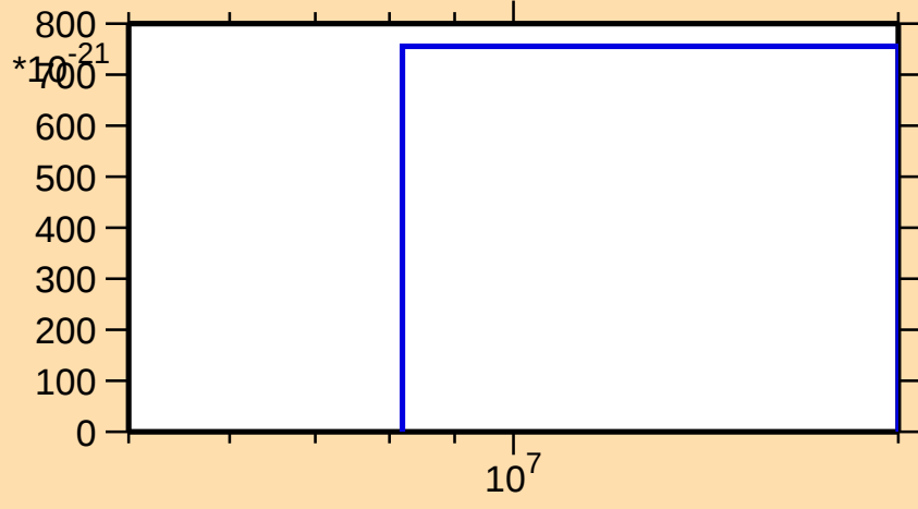
\sigma vs. E for ^{92}\text{Rb}(\text{mt 11})
