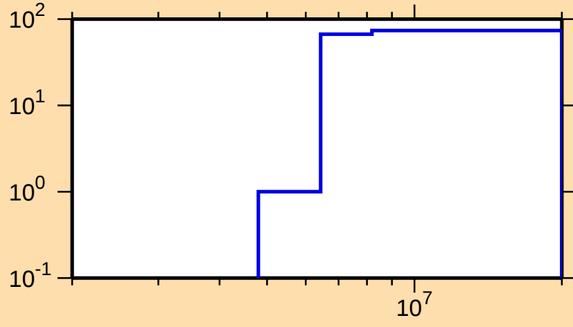
\Delta\sigma/\sigma vs. E for ^{92}\text{Rb}(n,p)
