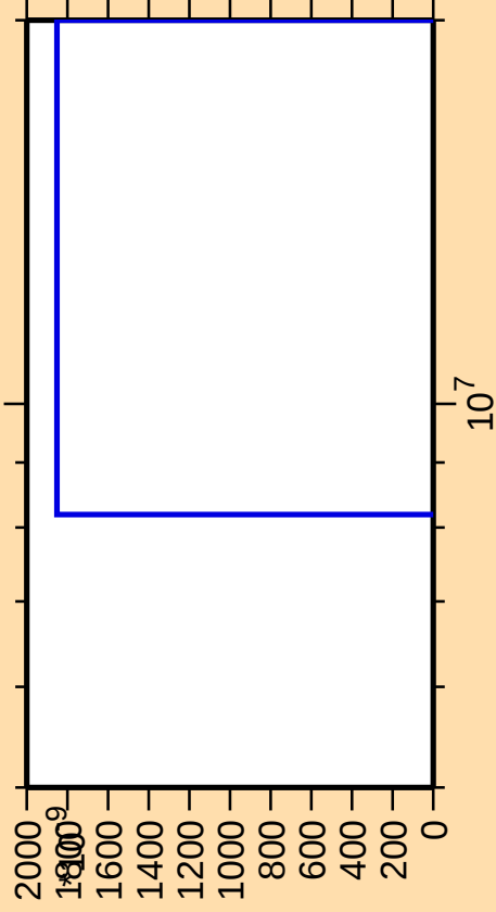
\Delta\sigma/\sigma vs. E for ^{92}\text{Rb}(\text{mt 11})
