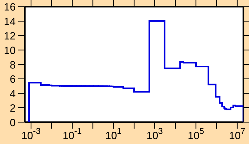
\sigma vs. E for ^{92}\text{Rb}(n,\text{el.})
