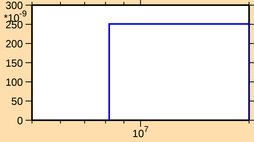
\sigma vs. E for ^{92}\text{Rb}(n,nd)
