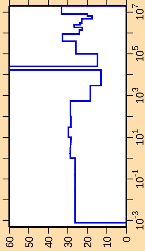
\Delta\sigma/\sigma vs. E for ^{92}\text{Rb}(n,\text{el.})
