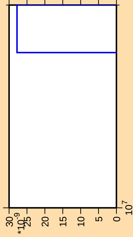
\Delta\sigma/\sigma vs. E for ^{93}\text{Rb}(\text{mt 11})
