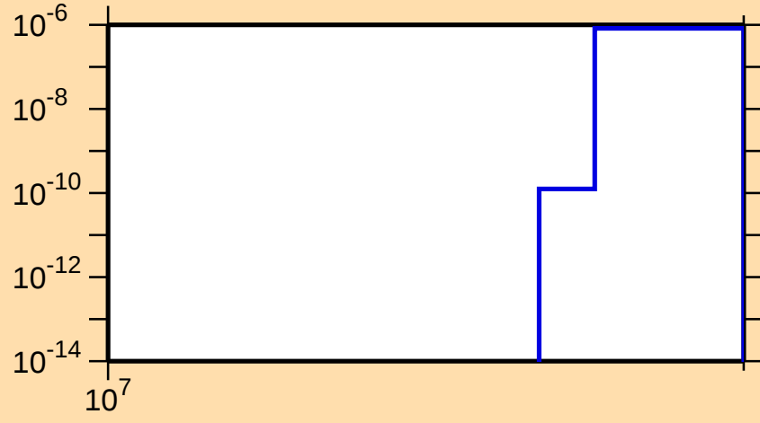
\sigma vs. E for ^{93}\text{Rb}(n,\text{nd})
