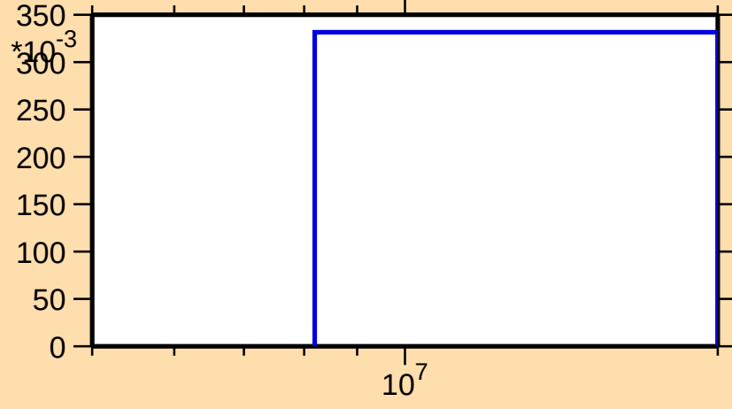
\sigma vs. E for ^{93}\text{Rb}(n,3n)
