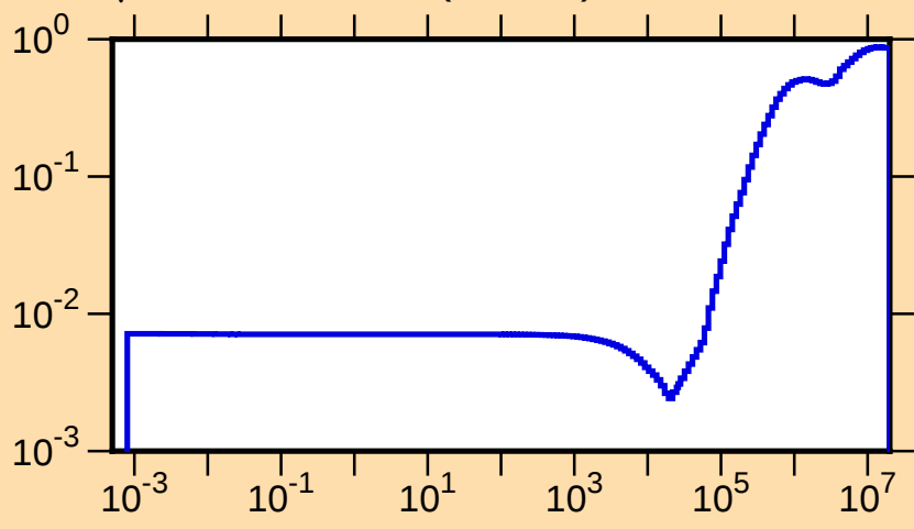
\mu vs. E for ^{94}\text{Rb}(\text{mt251})
