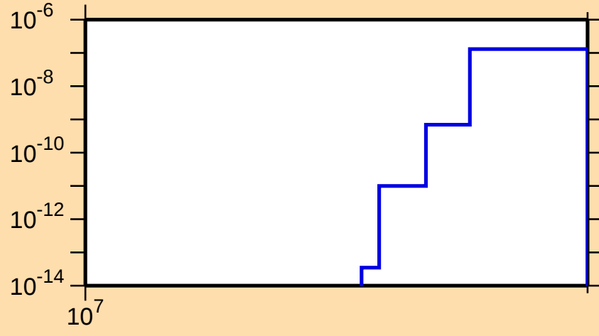
\sigma vs. E for ^{94}\text{Rb}(n,2n\alpha)
