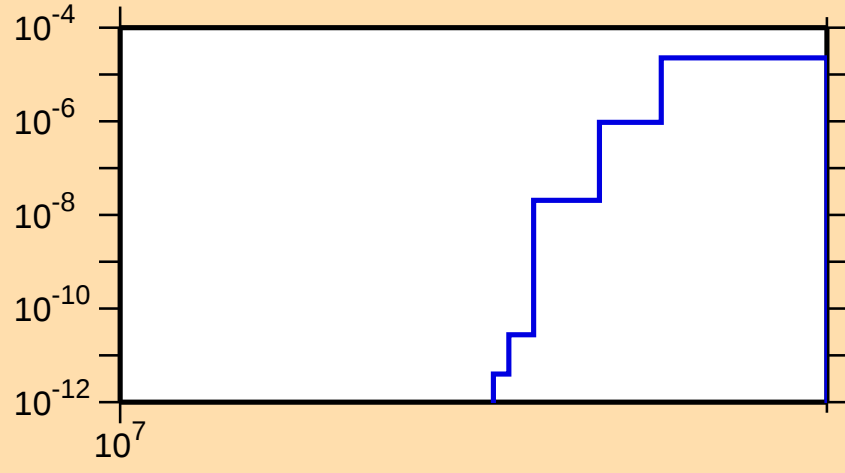
\sigma vs. E for ^{94}\text{Rb}(n,\text{nd})
