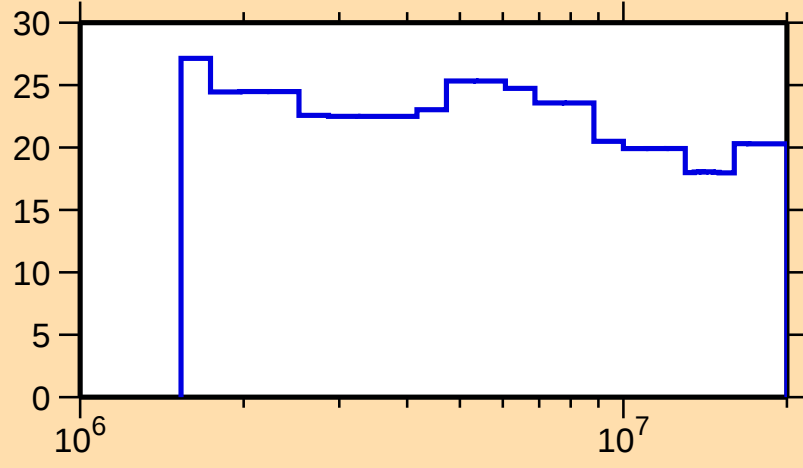
\Delta\sigma/\sigma vs. E for ^{94}\text{Rb}(n,n\text{nonel.})
