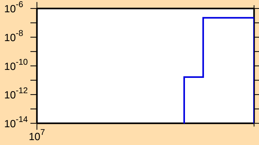
\sigma vs. E for ^{94}\text{Rb}(n,2np)
