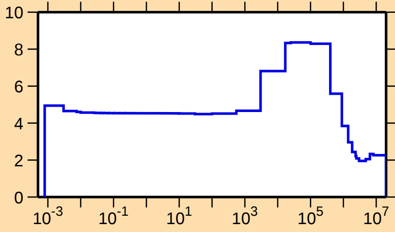
\sigma vs. E for ^{94}\text{Rb}(n,\text{el.})
