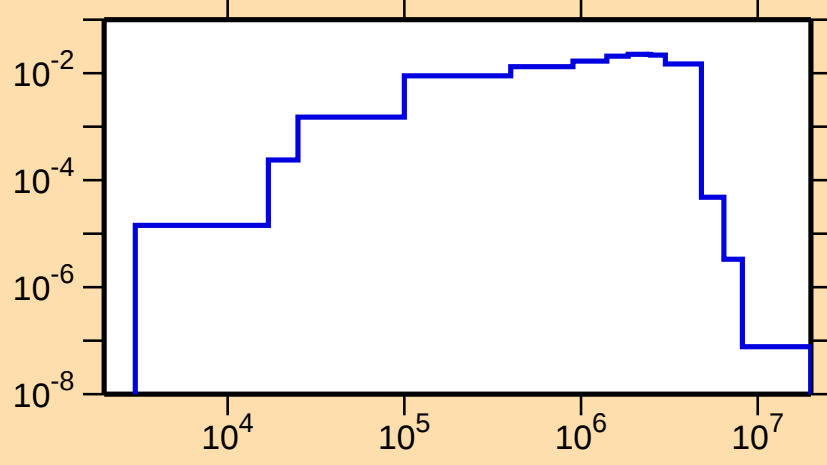
\sigma vs. E for ^{94}\text{Rb}(n,n_1)
