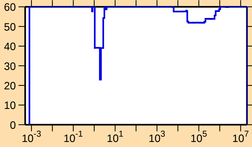
\Delta\sigma/\sigma vs. E for ^{167}\text{Re}(n,\gamma)
