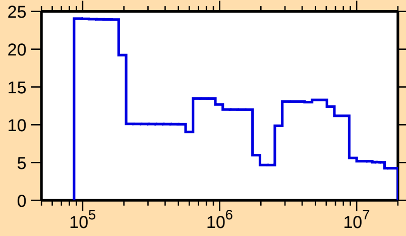
\Delta\sigma/\sigma vs. E for ^{167}\text{Re}(n,\text{tot.})
