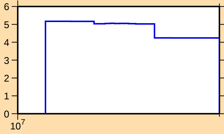
\Delta\sigma/\sigma vs. E for ^{167}\text{Re}(n,\text{tot.})
