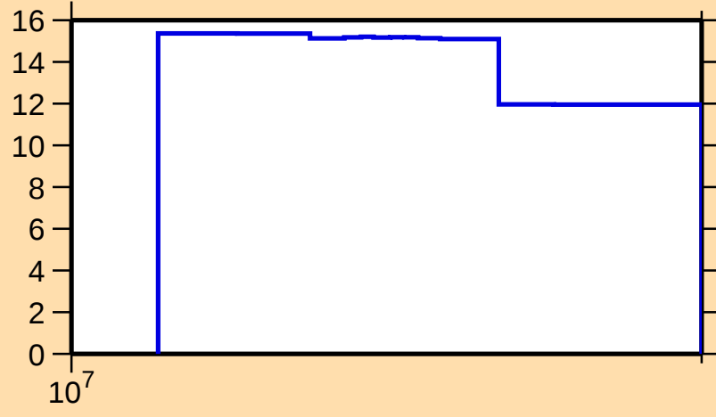
\Delta\sigma/\sigma vs. E for ^{167}\text{Re}(n,\text{el.})
