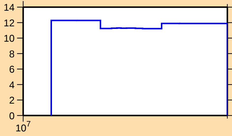
\Delta\sigma/\sigma vs. E for ^{167}\text{Re}(n,\text{nonel.})
