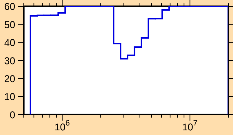
\Delta\sigma/\sigma vs. E for ^{167}\text{Re}(n,n_1)
