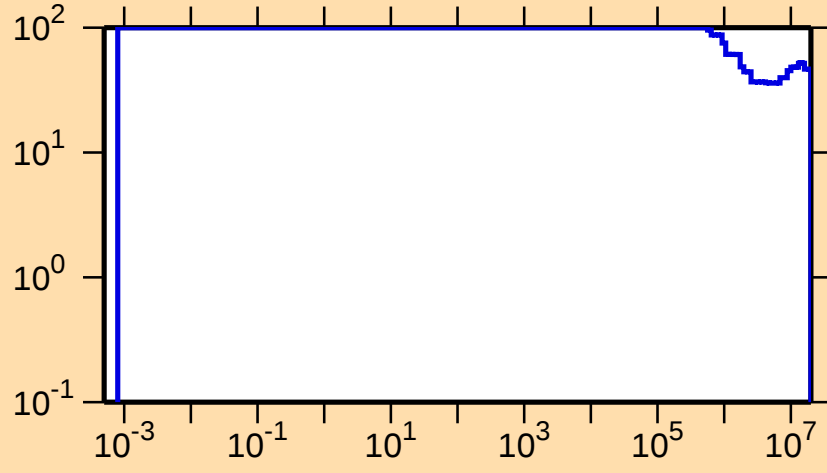
\Delta\sigma/\sigma vs. E for ^{167}\text{Re}(n,p)
