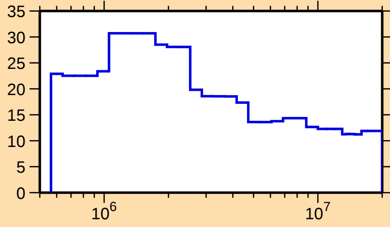
\Delta\sigma/\sigma vs. E for ^{167}\text{Re}(n,\text{nonel.})
