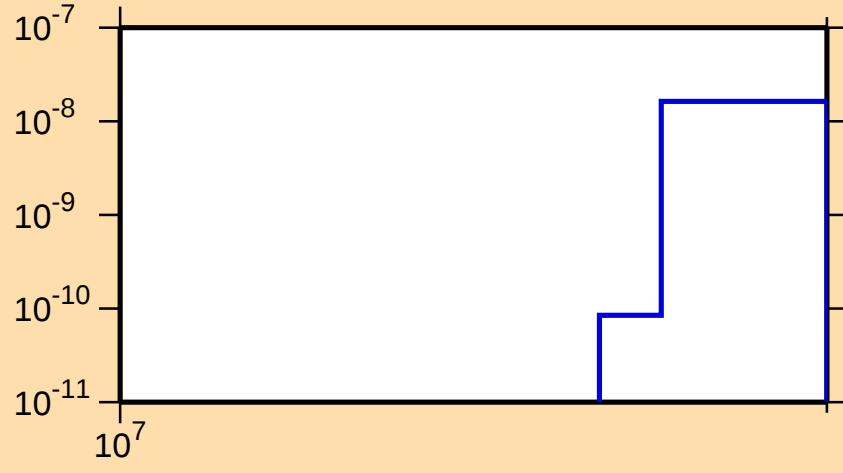
\sigma vs. E for ^{167}\text{Re}(n,nt)
