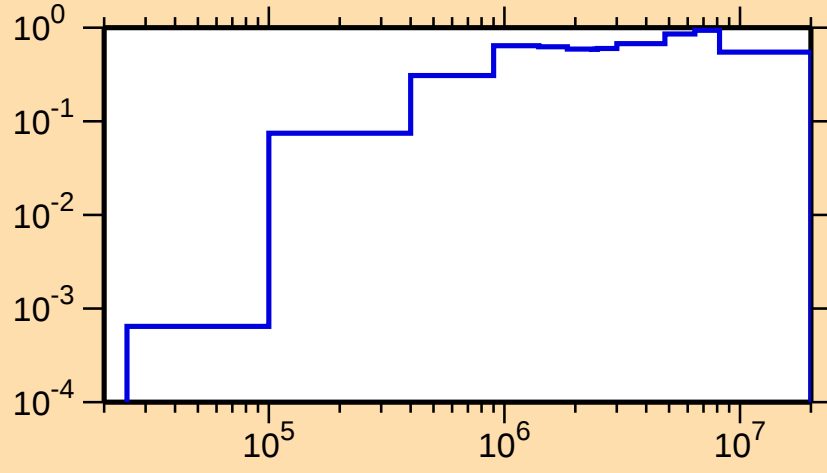
\sigma vs. E for ^{167}\text{Re}(n,\text{inel.})
