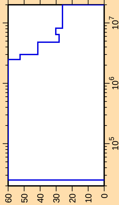
\Delta\sigma/\sigma vs. E for ^{167}\text{Re}(n,\text{inel.})
