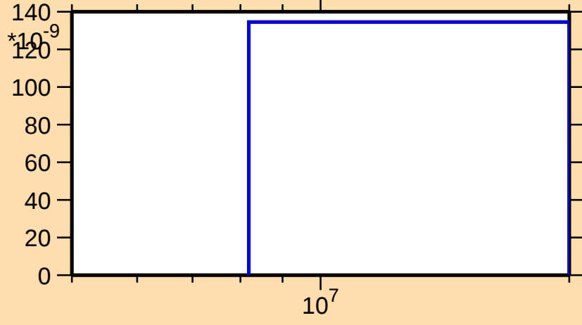
\sigma vs. E for ^{167}\text{Re}(n,\text{nd})
