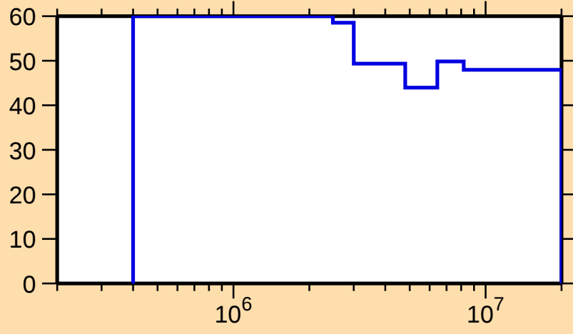
\Delta\sigma/\sigma vs. E for ^{167}\text{Re}(n,n\text{cont.})
