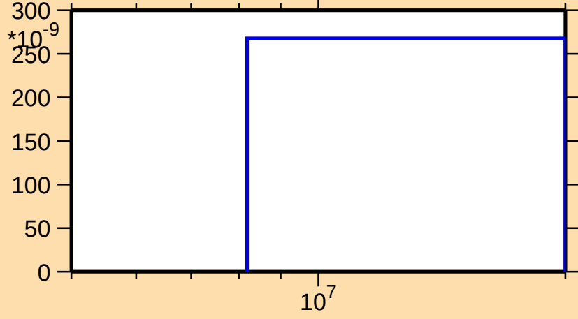
\sigma vs. E for ^{167}\text{Re}(n,2n\alpha)
