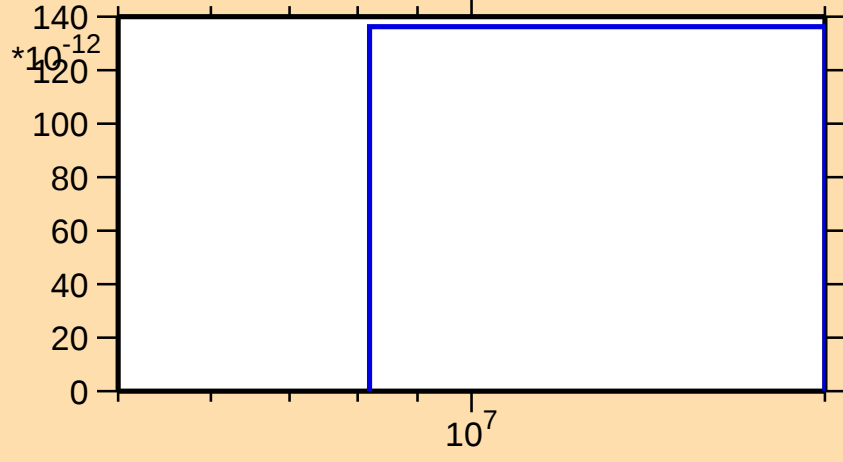
\sigma vs. E for ^{167}\text{Re}(n,nt)
