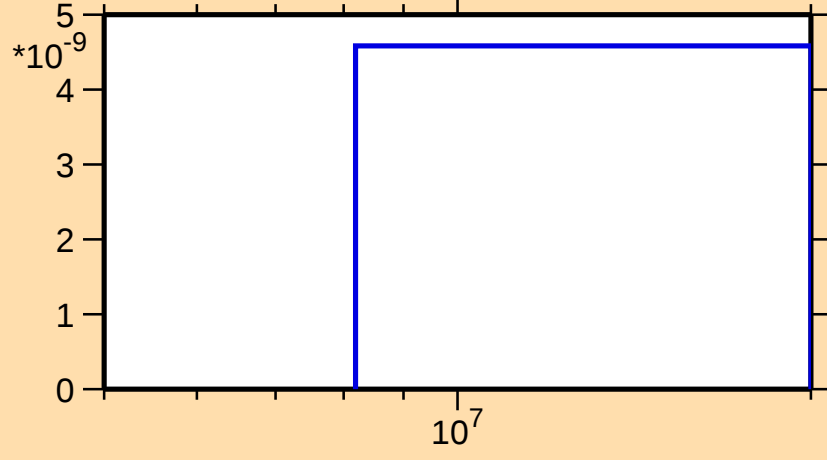
\sigma vs. E for ^{167}\text{Re}(n,\text{pt})
