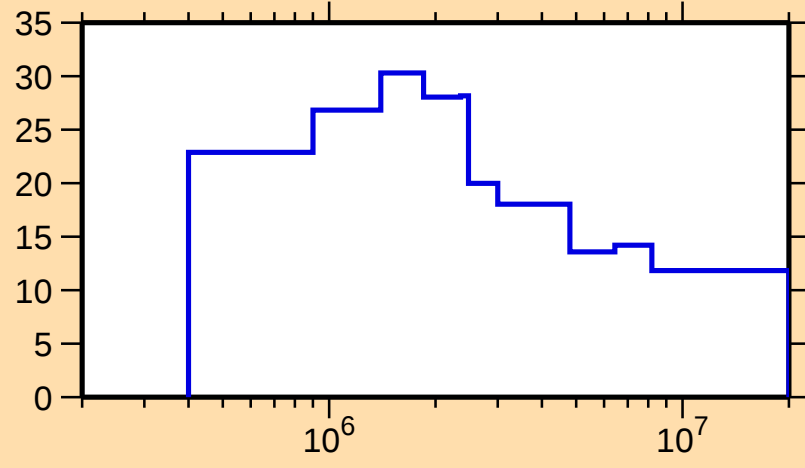
\Delta\sigma/\sigma vs. E for ^{167}\text{Re}(n,n\text{onel.})
