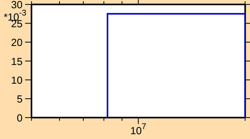
\sigma vs. E for ^{167}\text{Re}(n,2n)
