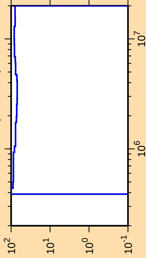
\Delta\sigma/\sigma vs. E for ^{168}\text{Re}(n,n_{\text{cont}})
