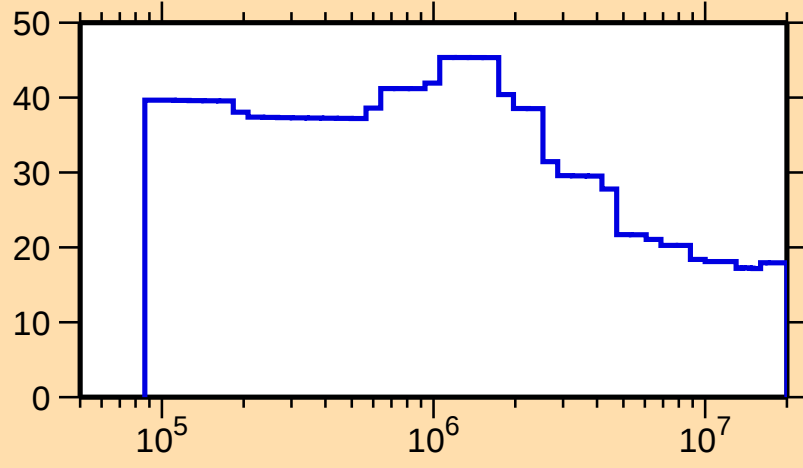
\Delta\sigma/\sigma vs. E for ^{168}\text{Re}(n,\text{nonel.})
