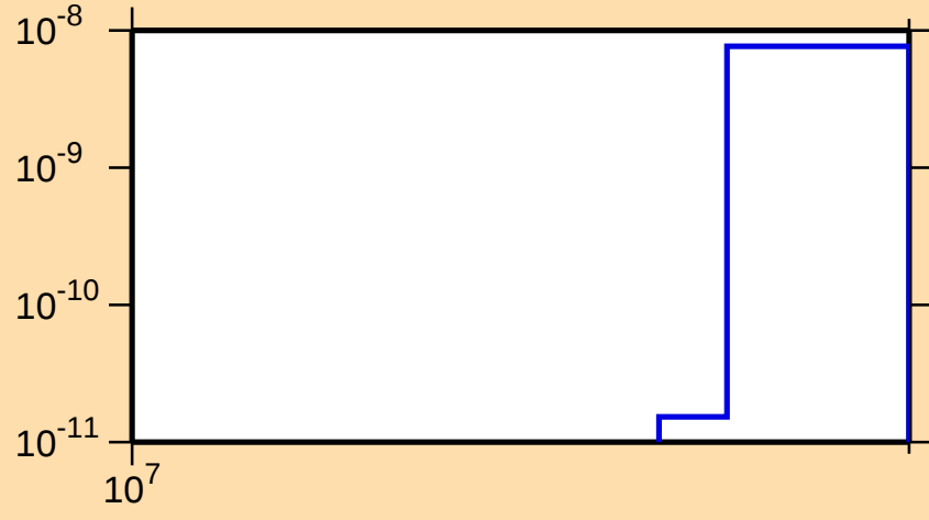
\sigma vs. E for ^{168}\text{Re}(n,nt)
