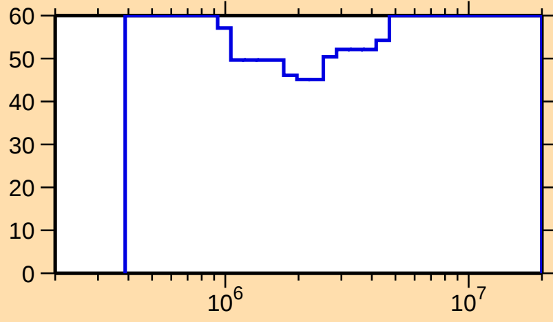
\Delta\sigma/\sigma vs. E for ^{168}\text{Re}(n,\text{inel.})
