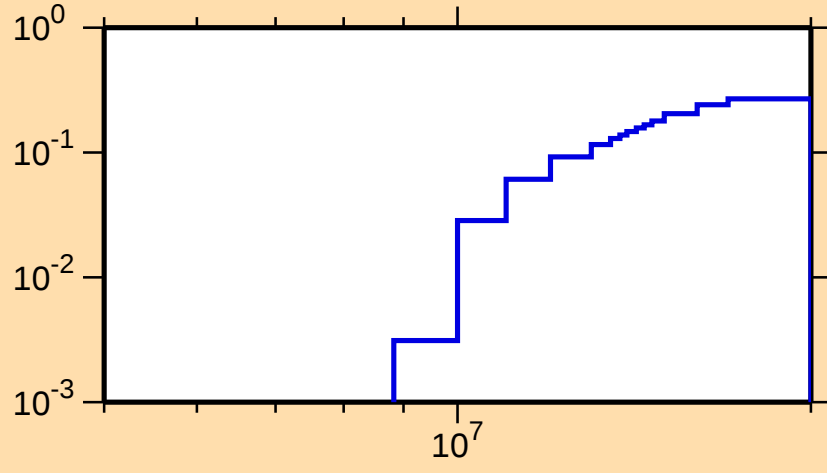
\sigma vs. E for ^{168}\text{Re}(n,2n)
