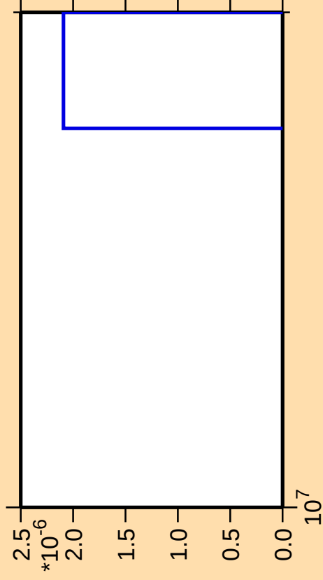
\Delta\sigma/\sigma vs. E for ^{168}\text{Re}(\text{mt 11})
