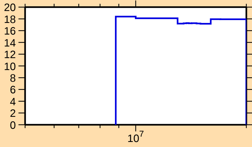
\Delta\sigma/\sigma vs. E for ^{168}\text{Re}(n,\text{nonel.})
