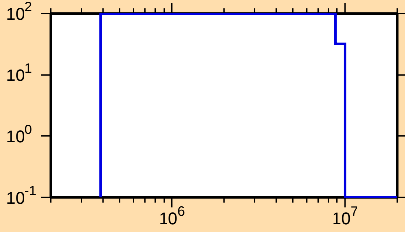
\Delta\sigma/\sigma vs. E for ^{168}\text{Re}(n,n_1)
