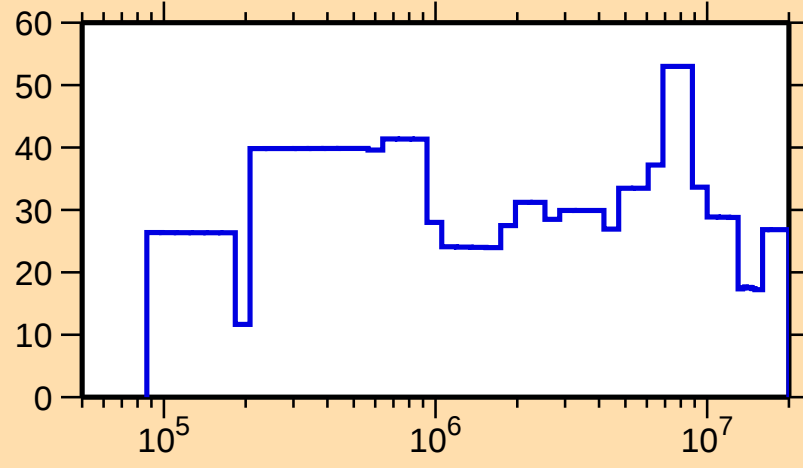
\Delta\sigma/\sigma vs. E for ^{168}\text{Re}(n,\text{el.})
