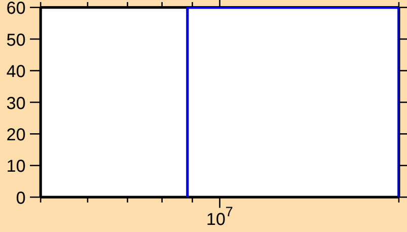
\Delta\sigma/\sigma vs. E for ^{168}\text{Re}(n,\text{inel.})
