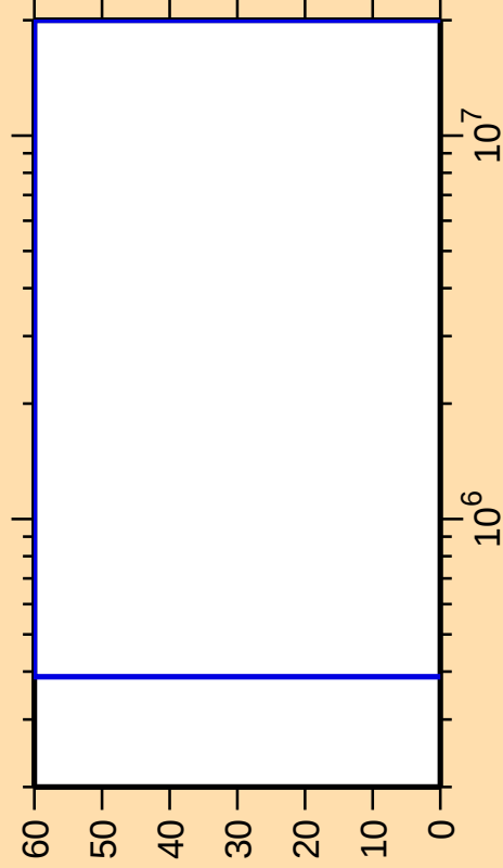
\Delta\sigma/\sigma vs. E for ^{168}\text{Re}(n,p)
