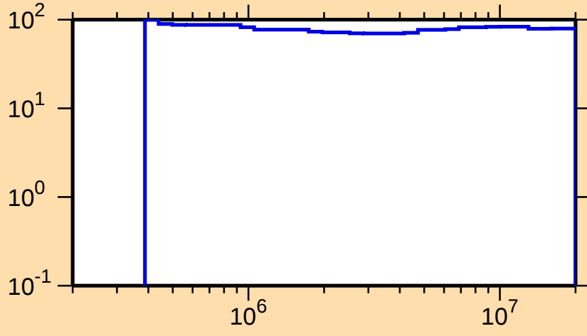
\Delta\sigma/\sigma vs. E for ^{168}\text{Re}(n,n\text{cont.})
