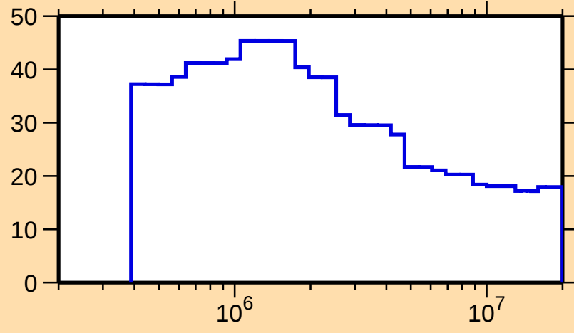
\Delta\sigma/\sigma vs. E for ^{168}\text{Re}(n,n\text{onel.})
