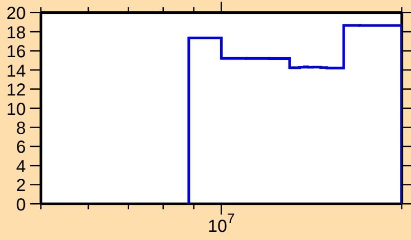
\Delta\sigma/\sigma vs. E for ^{168}\text{Re}(n,\text{tot.})
