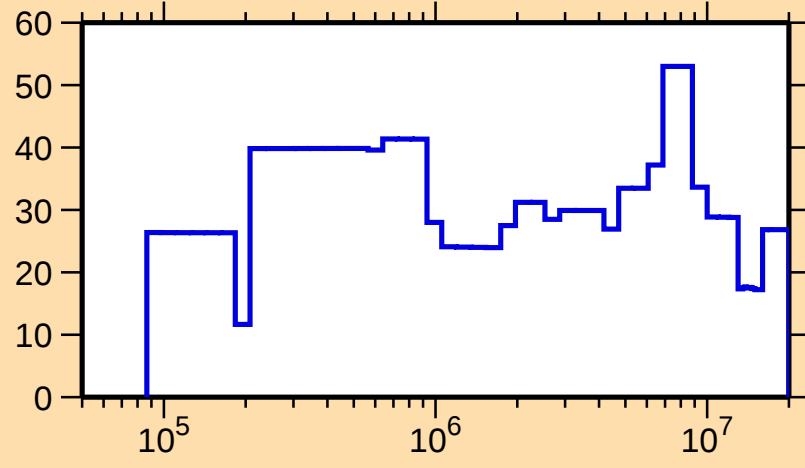
\Delta\sigma/\sigma vs. E for ^{168}\text{Re}(n,\text{el.})
