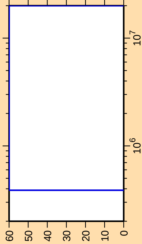
\Delta\sigma/\sigma vs. E for ^{168}\text{Re}(n,\alpha)
