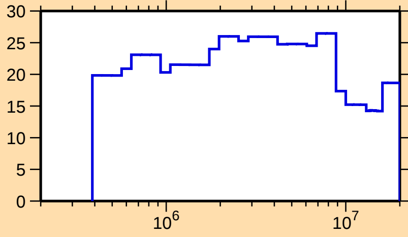
\Delta\sigma/\sigma vs. E for ^{168}\text{Re}(n,\text{tot.})
