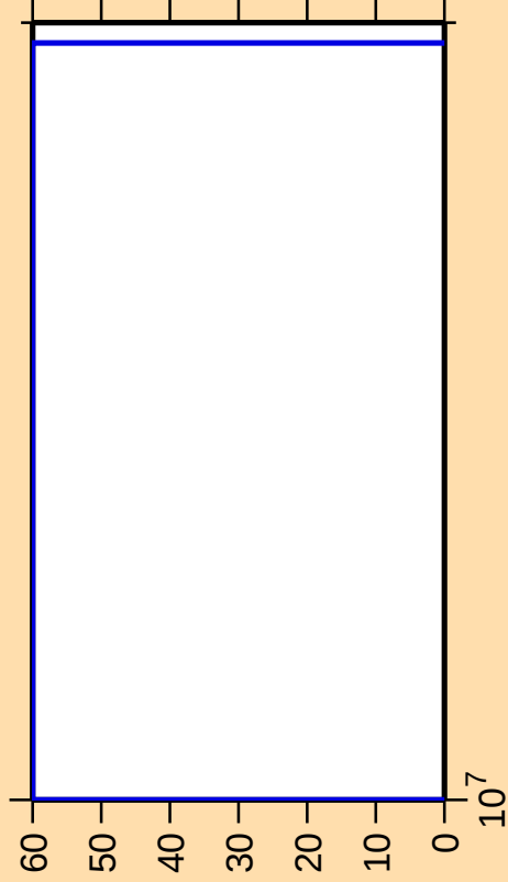
\Delta\sigma/\sigma vs. E for ^{168}\text{Re}(\text{mt } 34)
