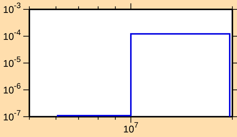
\sigma vs. E for ^{168}\text{Re}(n,2n\alpha)
