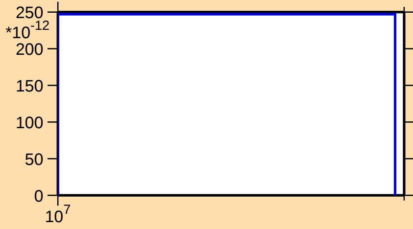
\sigma vs. E for ^{168}\text{Re}(\text{mt } 34)
