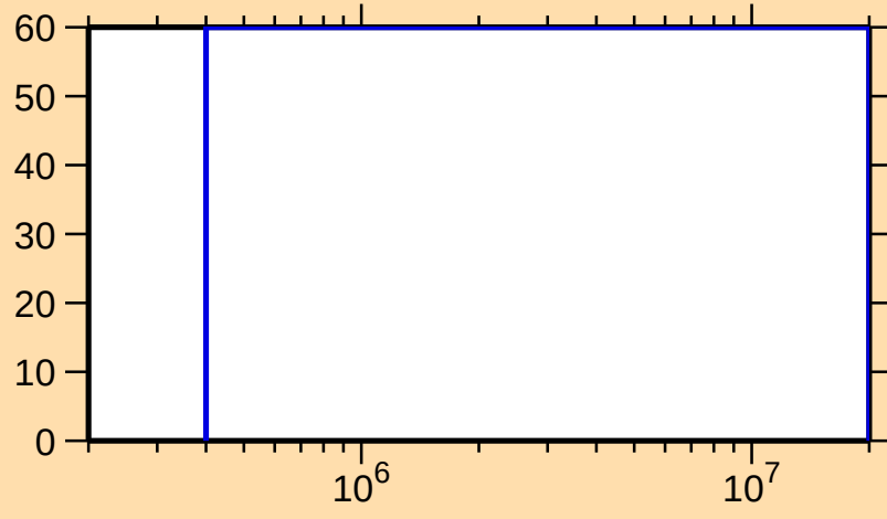
\Delta\sigma/\sigma vs. E for ^{168}\text{Re}(n,n\text{cont.})
