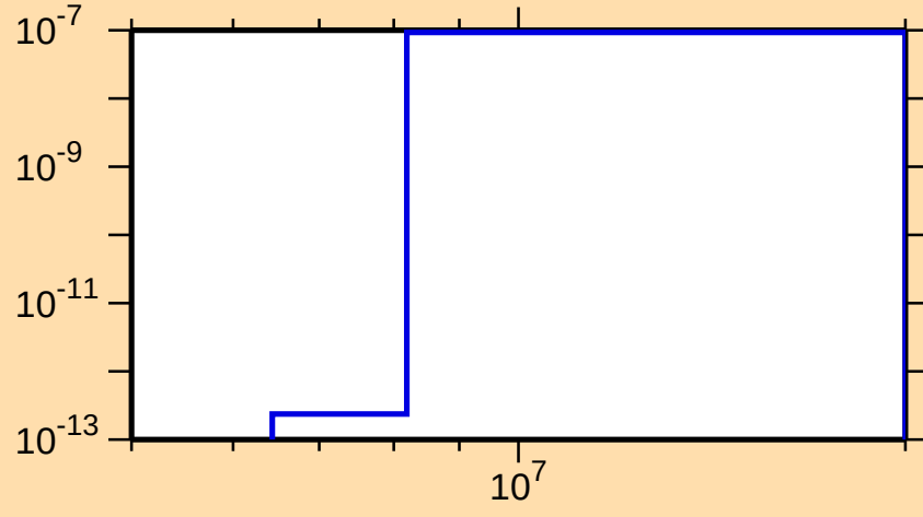
\sigma vs. E for ^{168}\text{Re}(\text{mt117})
