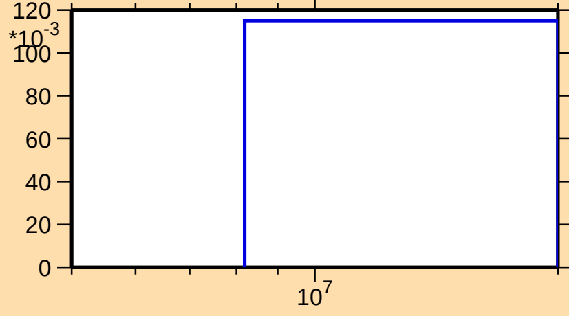
\sigma vs. E for ^{168}\text{Re}(n,2n)
