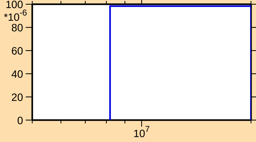
\sigma vs. E for ^{168}\text{Re}(n,2n\alpha)
