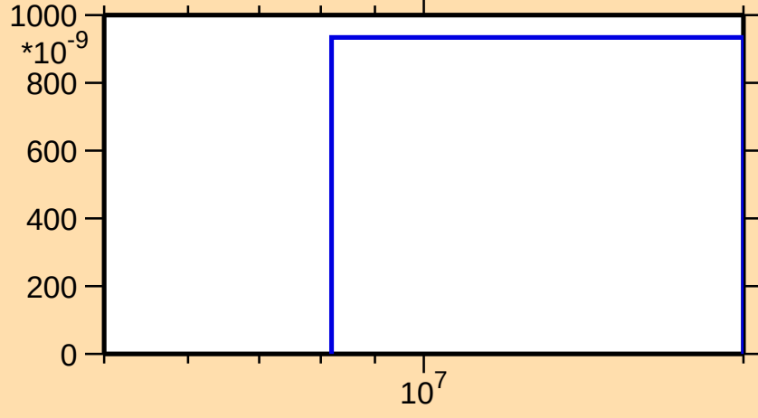
\sigma vs. E for ^{168}\text{Re}(n,\text{pd})
