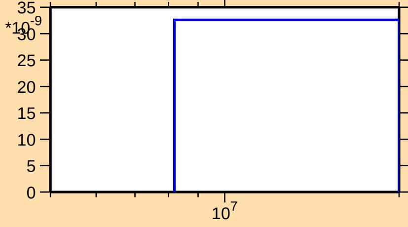
\sigma vs. E for ^{168}\text{Re}(n,\text{pt})
