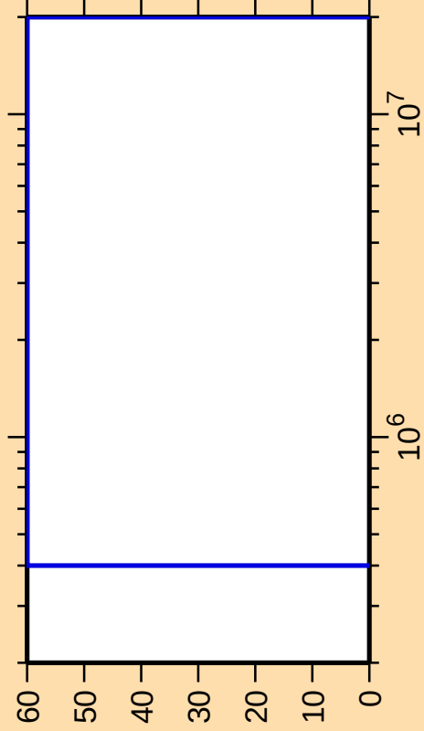
\Delta\sigma/\sigma vs. E for ^{168}\text{Re}(n,\gamma)
