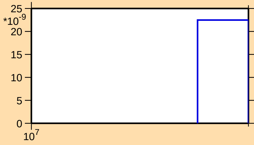
\sigma vs. E for ^{169}\text{Re}(n,3n)
