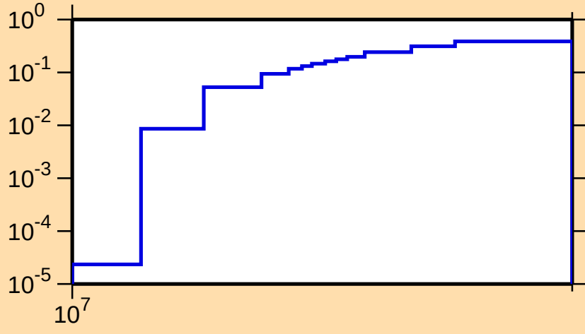
\sigma vs. E for ^{169}\text{Re}(n,2n)
