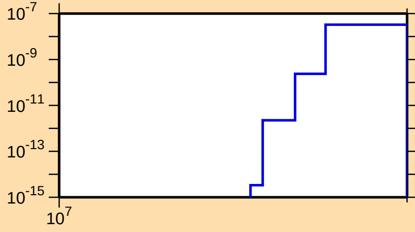
\sigma vs. E for ^{169}\text{Re}(n,nt)
