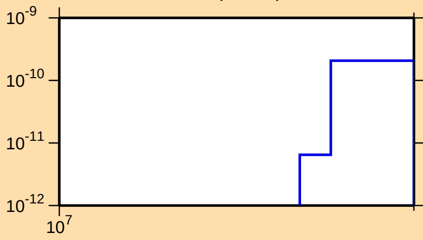
\sigma vs. E for ^{169}\text{Re}(\text{mt 34})
