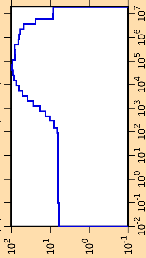
\Delta\mu/\mu vs. E for ^{169}\text{Re}(\text{mt251})
