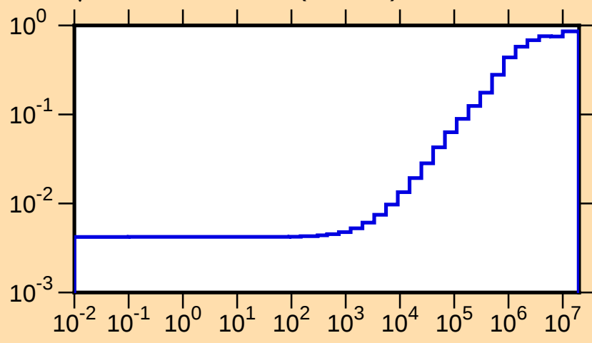
\mu vs. E for ^{169}\text{Re}(\text{mt251})
