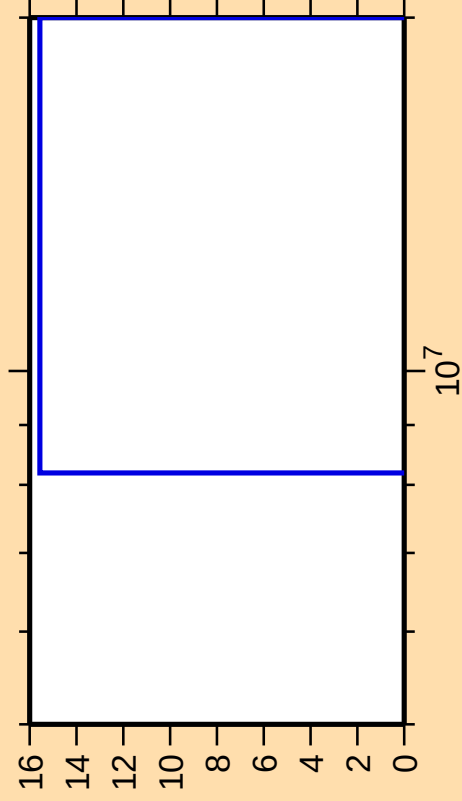
\Delta\sigma/\sigma vs. E for ^{169}\text{Re}(\text{mt 34})
