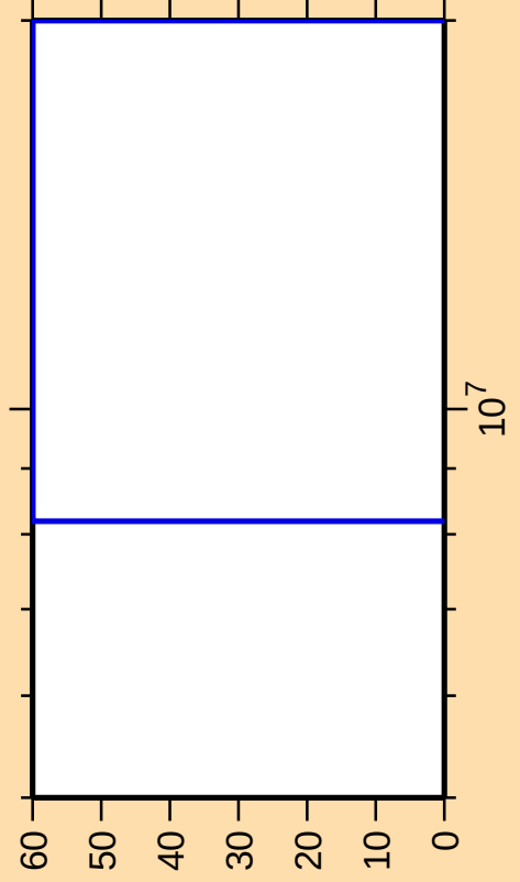
\Delta\sigma/\sigma vs. E for ^{169}\text{Re}(n,n\text{cont.})
