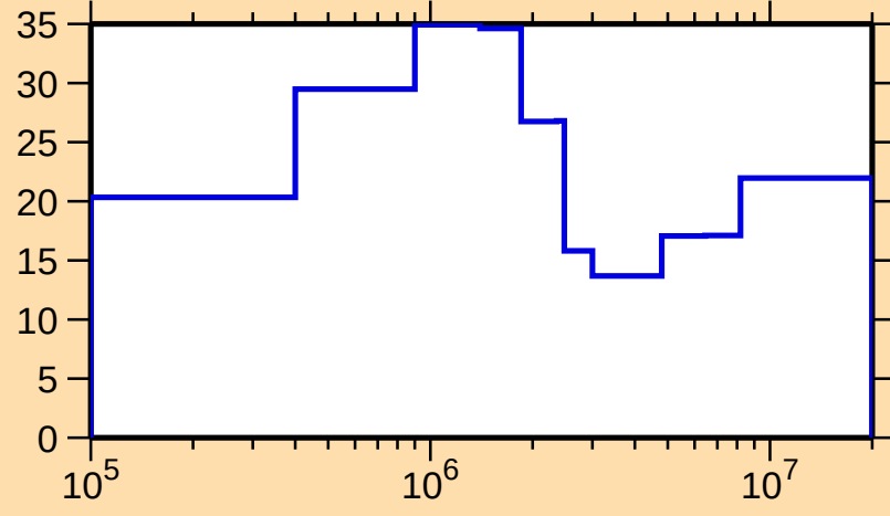
\Delta\sigma/\sigma vs. E for ^{169}\text{Re}(n,\text{tot.})
