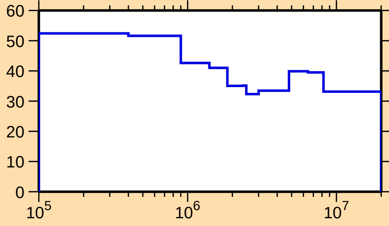
\Delta\sigma/\sigma vs. E for ^{169}\text{Re}(n,\text{nonel.})
