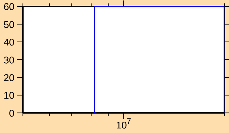
\Delta\sigma/\sigma vs. E for ^{169}\text{Re}(n,2n)
