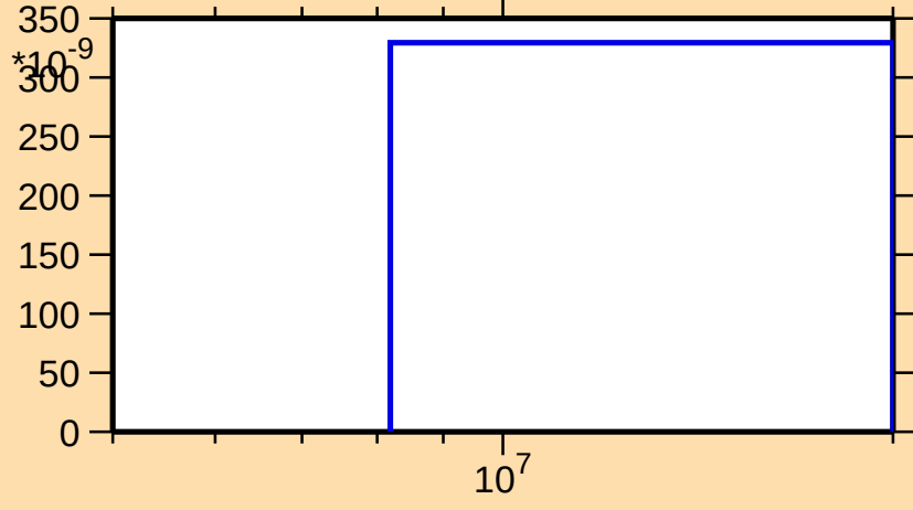
\sigma vs. E for ^{169}\text{Re}(n,\text{pd})
