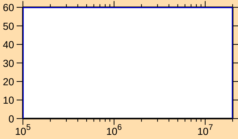
\Delta\sigma/\sigma vs. E for ^{169}\text{Re}(n,n\text{cont.})
