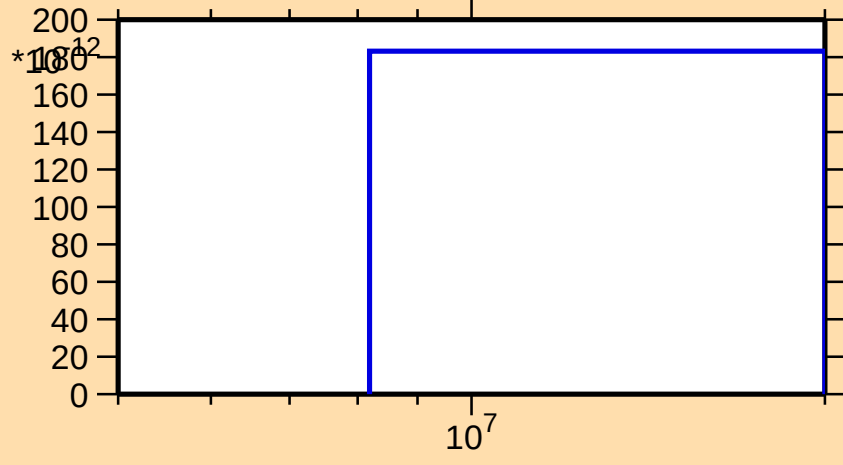
\sigma vs. E for ^{169}\text{Re}(n,3n)
