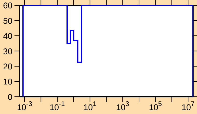
\Delta\sigma/\sigma vs. E for ^{169}\text{Re}(n,\gamma)
