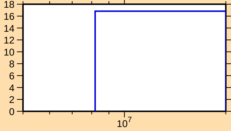
\Delta\sigma/\sigma vs. E for ^{169}\text{Re}(n,\text{el.})
