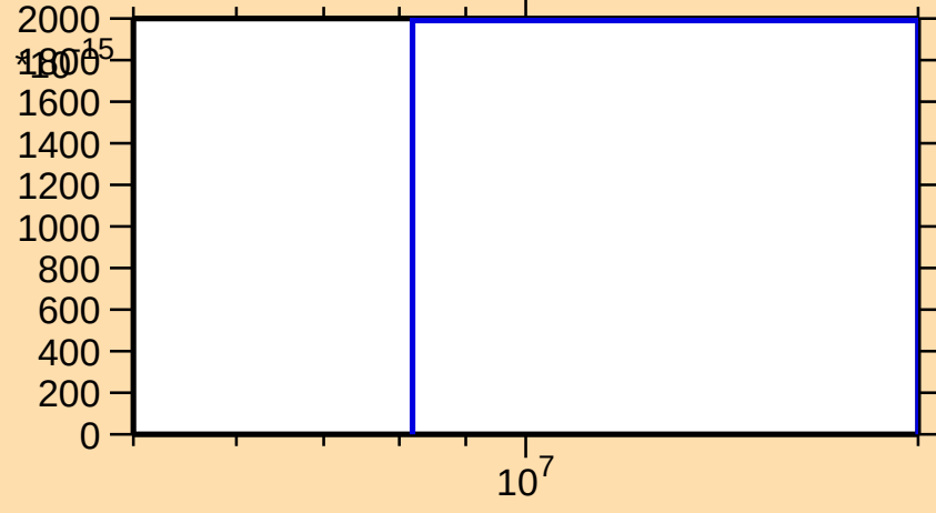
\sigma vs. E for ^{169}\text{Re}(\text{mt 34})
