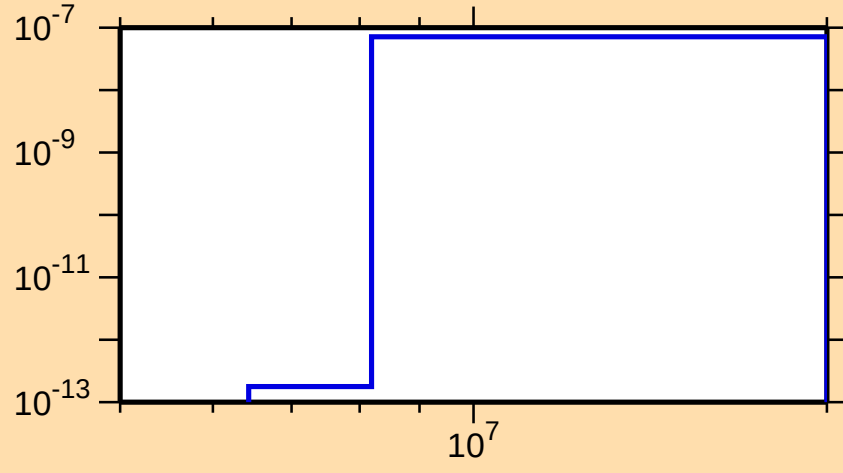
\sigma vs. E for ^{169}\text{Re}(\text{mt117})
