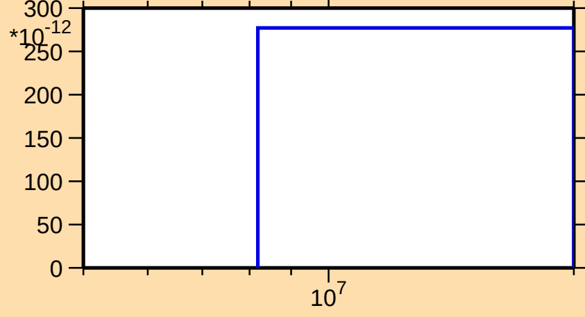
\sigma vs. E for ^{169}\text{Re}(n,nt)
