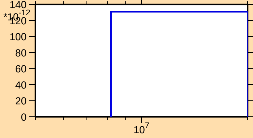
\sigma vs. E for ^{169}\text{Re}(n,\text{pt})
