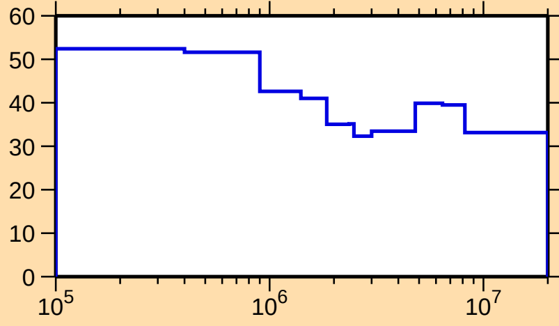
\Delta\sigma/\sigma vs. E for ^{169}\text{Re}(n,\text{nonel.})
