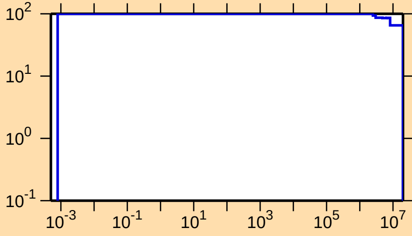
\Delta\sigma/\sigma vs. E for ^{169}\text{Re}(n,p)
