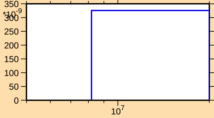
\sigma vs. E for ^{169}\text{Re}(n,2n\alpha)
