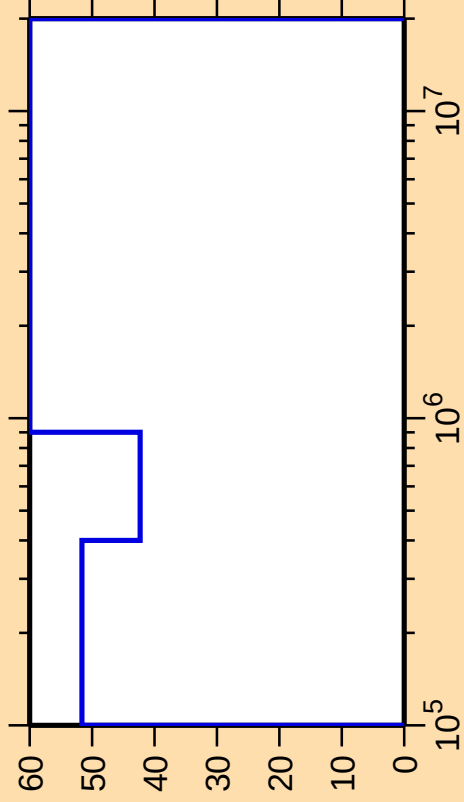
\Delta\sigma/\sigma vs. E for ^{169}\text{Re}(n,\text{inel.})
