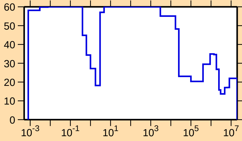
\Delta\sigma/\sigma vs. E for ^{169}\text{Re}(n,\text{tot.})
