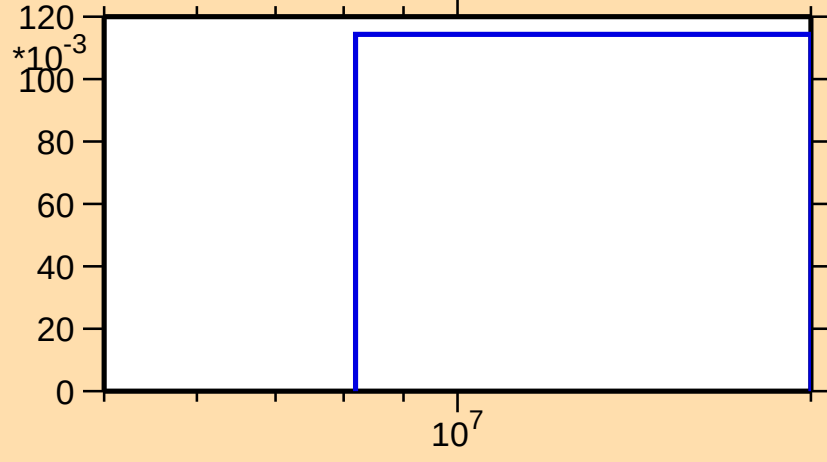
\sigma vs. E for ^{169}\text{Re}(n,2n)
