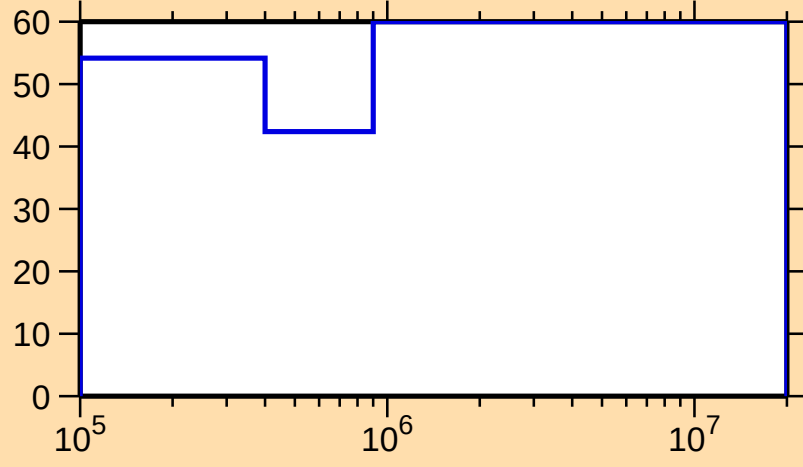
\Delta\sigma/\sigma vs. E for ^{169}\text{Re}(n,n_1)
