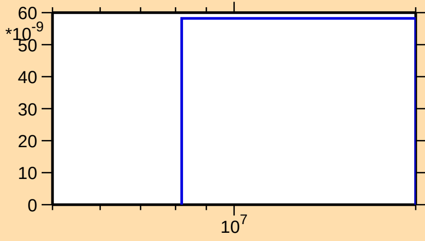
\sigma vs. E for ^{169}\text{Re}(n,\text{nd})
