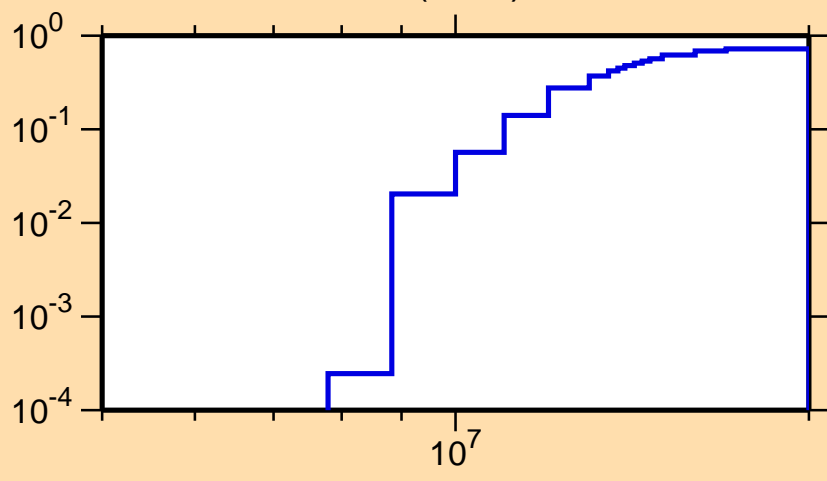
\sigma vs. E for ^{170}\text{Re}(n,2n)
