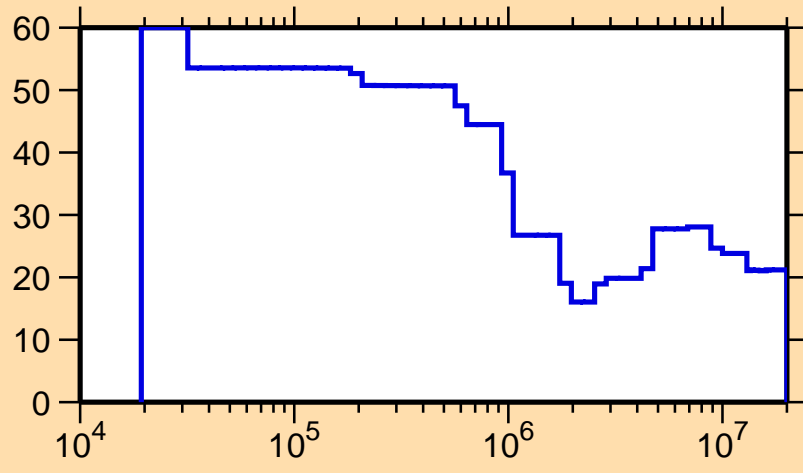
\Delta\sigma/\sigma vs. E for ^{170}\text{Re}(n,\text{nonel.})
