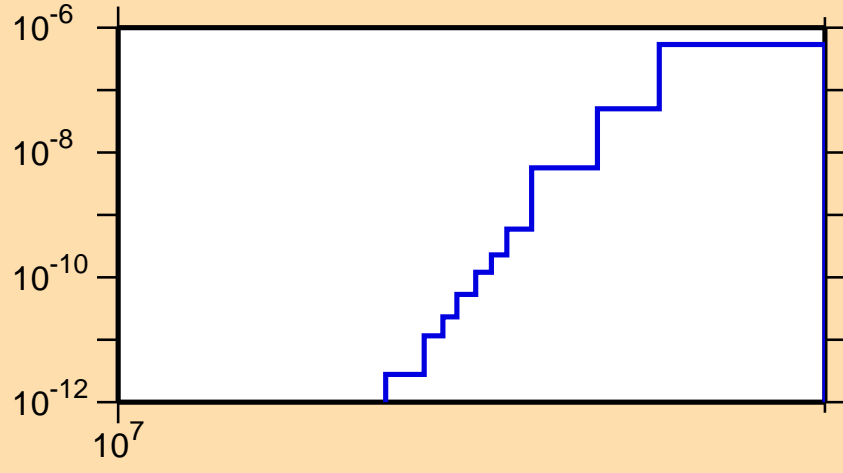
\sigma vs. E for ^{170}\text{Re}(n,\text{pt})
