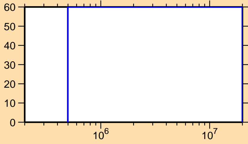
\Delta\sigma/\sigma vs. E for ^{170}\text{Re}(n,n\text{cont.})
