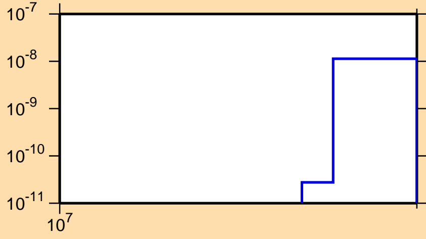
\sigma vs. E for ^{170}\text{Re}(n,nt)
