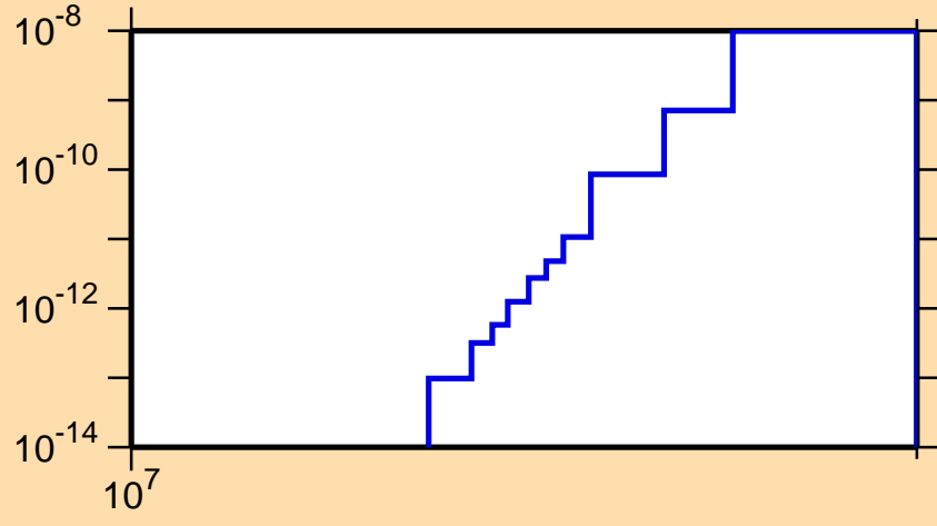
\sigma vs. E for ^{170}\text{Re}(\text{mt 34})
