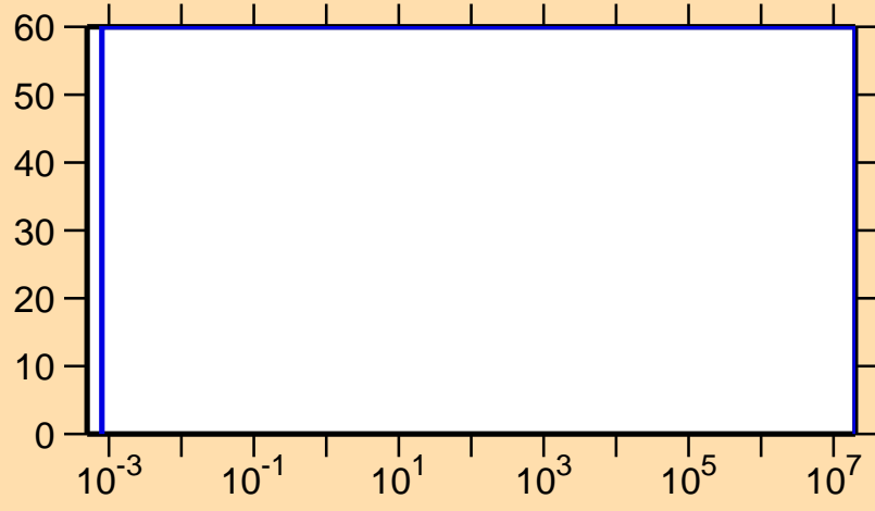
\Delta\sigma/\sigma vs. E for ^{170}\text{Re}(n,p)
