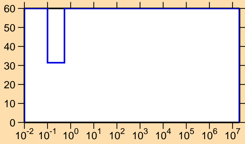
\Delta\sigma/\sigma vs. E for ^{170}\text{Re}(n,\gamma)
