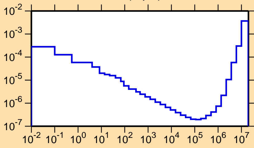
\sigma vs. E for ^{170}\text{Re}(n,p\alpha)
