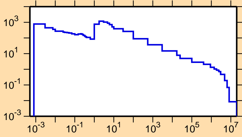
\sigma vs. E for ^{170}\text{Re}(n,\gamma)
