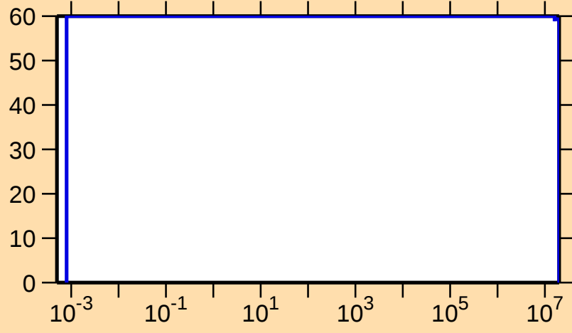
\Delta\sigma/\sigma vs. E for ^{172}\text{Re}(n,p)
