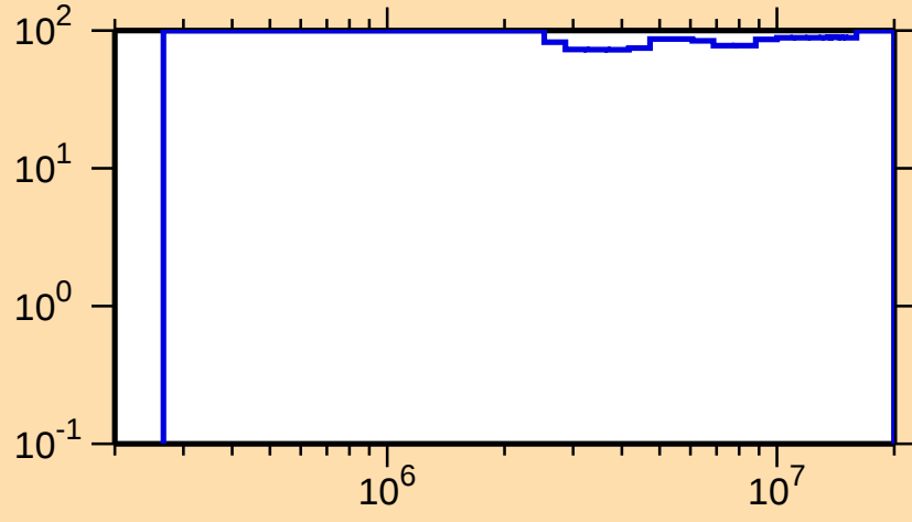
\Delta\sigma/\sigma vs. E for ^{172}\text{Re}(n,n_1)
