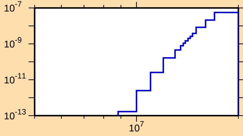
\sigma vs. E for ^{172}\text{Re}(\text{mt117})
