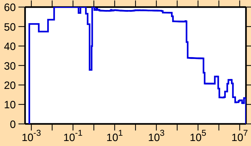
\Delta\sigma/\sigma vs. E for ^{172}\text{Re}(n,\text{tot.})
