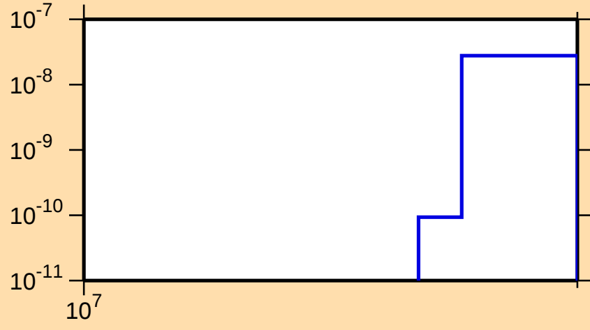
\sigma vs. E for ^{172}\text{Re}(n,nt)
