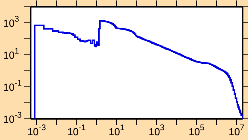
\sigma vs. E for ^{172}\text{Re}(n,\gamma)
