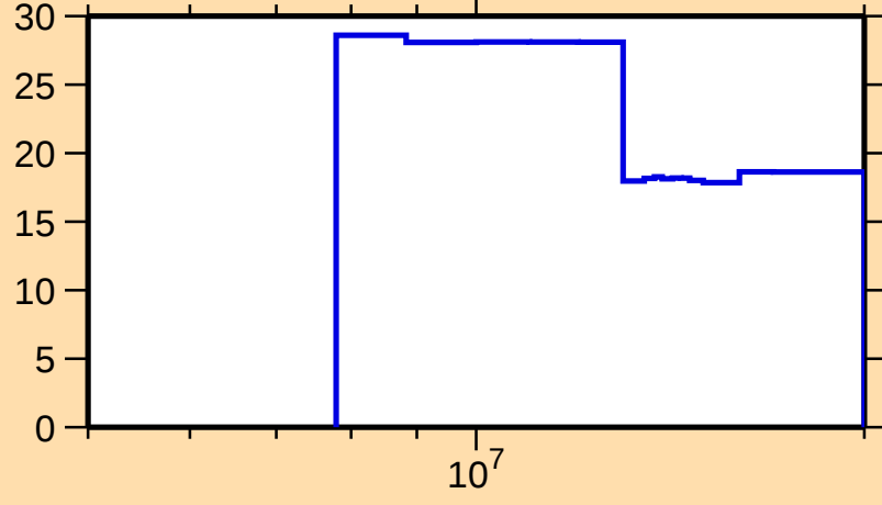
\Delta\sigma/\sigma vs. E for ^{172}\text{Re}(n,\text{el.})
