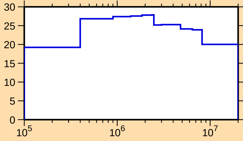
\Delta\sigma/\sigma vs. E for ^{172}\text{Re}(n,n\text{onel.})
