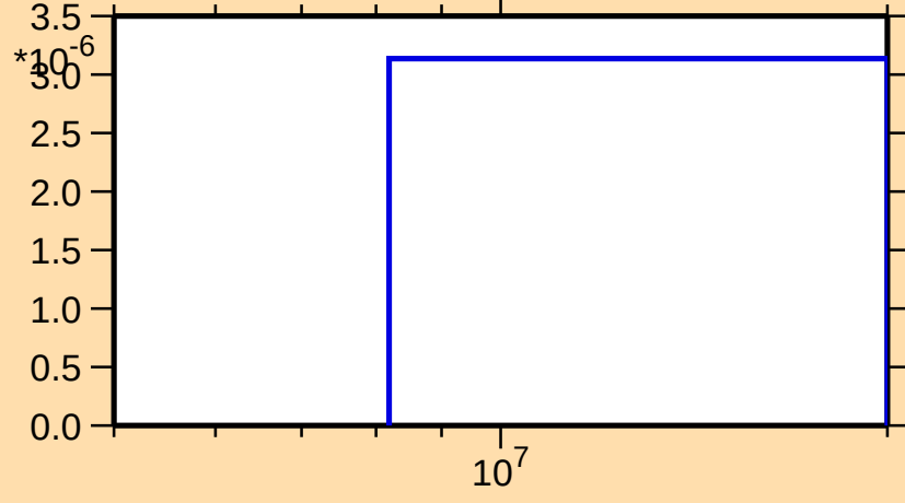
\sigma vs. E for ^{172}\text{Re}(n,\text{nd})
