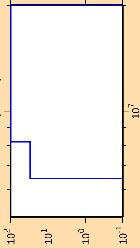
\Delta\sigma/\sigma vs. E for ^{172}\text{Re}(n,\text{He3})
