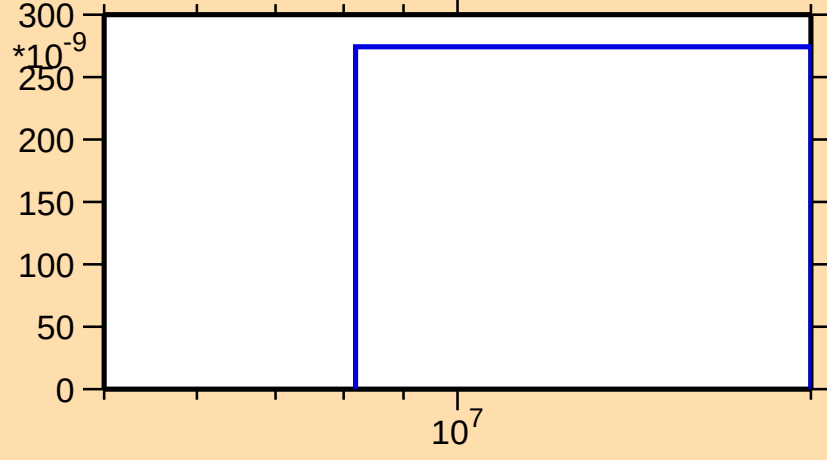
\sigma vs. E for ^{172}\text{Re}(n,3n)
