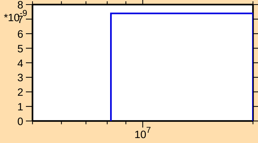
\sigma vs. E for ^{172}\text{Re}(n,\text{pd})
