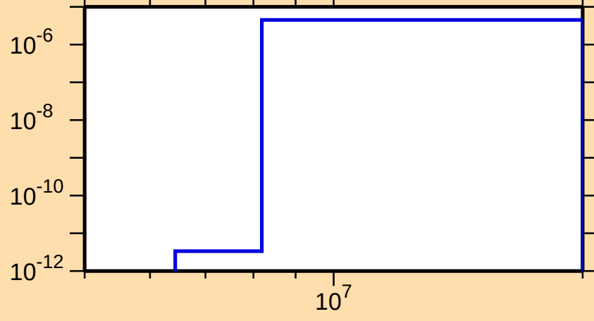
\sigma vs. E for ^{172}\text{Re}(n,\text{He3})
