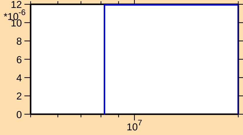
\sigma vs. E for ^{172}\text{Re}(n,2n\alpha)
