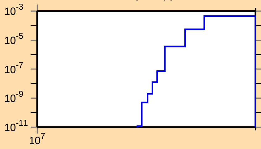
\sigma vs. E for ^{175}\text{Re}(n,2np)
