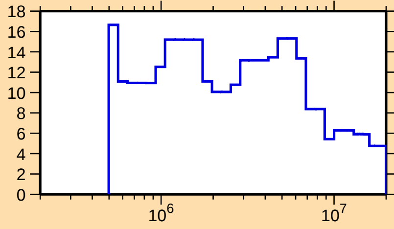
\Delta\sigma/\sigma vs. E for ^{175}\text{Re}(n,\text{el.})
