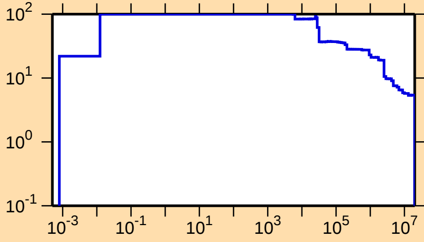
\Delta\sigma/\sigma vs. E for ^{175}\text{Re}(n,\text{nonel.})
