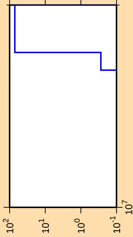
\Delta\sigma/\sigma vs. E for ^{175}\text{Re}(n,\text{pt})
