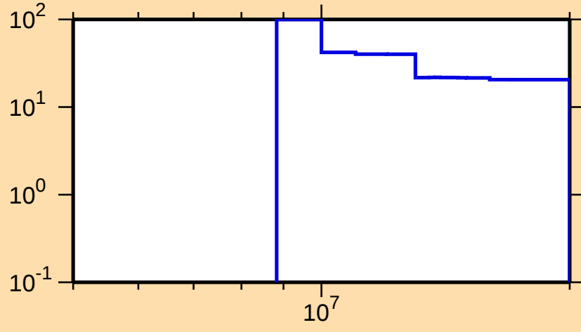
\Delta\sigma/\sigma vs. E for ^{175}\text{Re}(n,2n)
