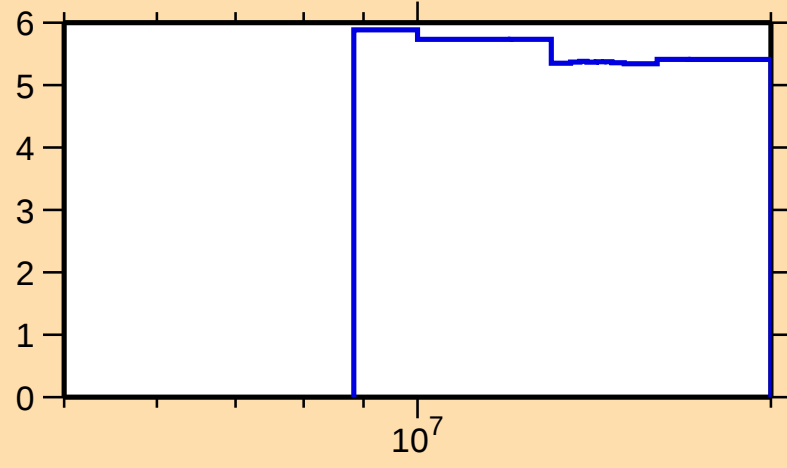
\Delta\sigma/\sigma vs. E for ^{175}\text{Re}(n,\text{nonel.})
