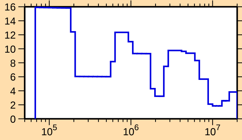
\Delta\sigma/\sigma vs. E for ^{175}\text{Re}(n,\text{tot.})
