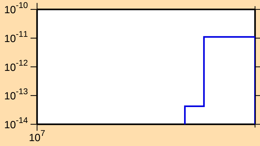
\sigma vs. E for ^{175}\text{Re}(n,\text{pt})
