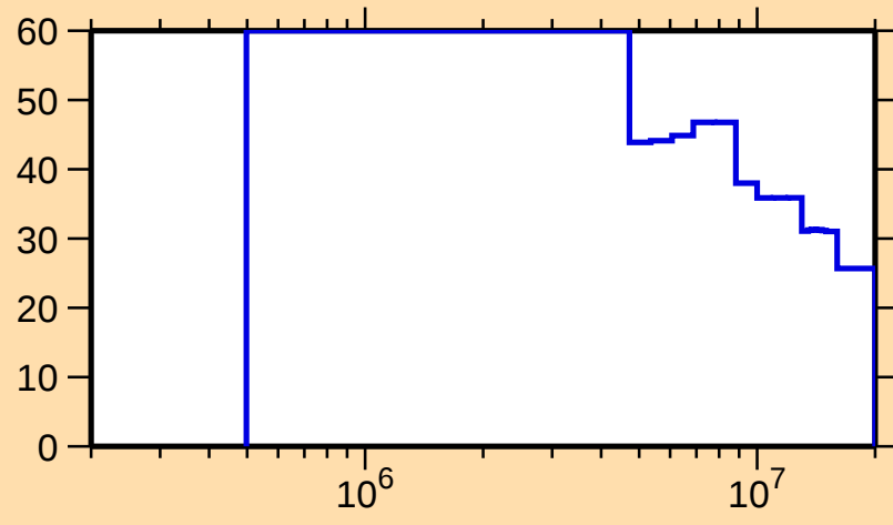
\Delta\sigma/\sigma vs. E for ^{175}\text{Re}(n,n_1)
