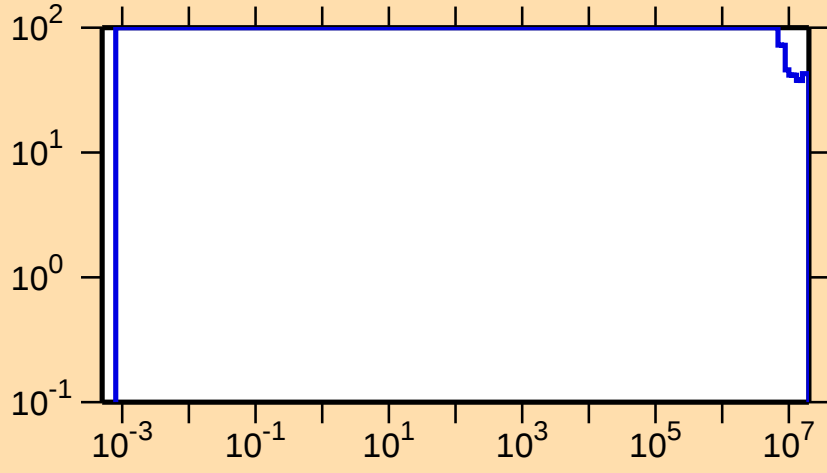
\Delta\sigma/\sigma vs. E for ^{175}\text{Re}(n,p)
