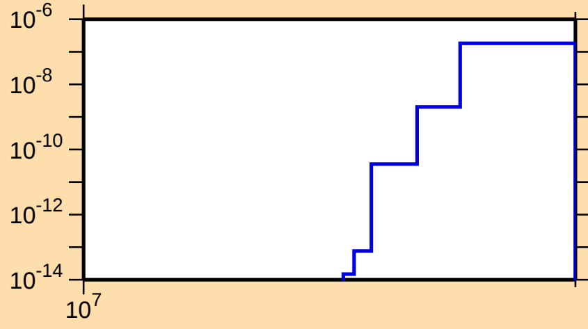
\sigma vs. E for ^{175}\text{Re}(n,nt)
