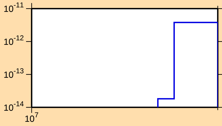
\sigma vs. E for ^{175}\text{Re}(\text{mt 34})
