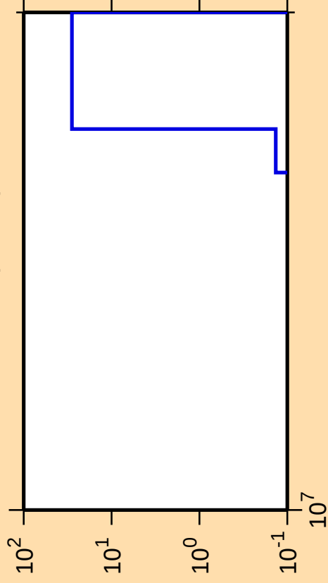
\Delta\sigma/\sigma vs. E for ^{175}\text{Re}(\text{mt 34})
