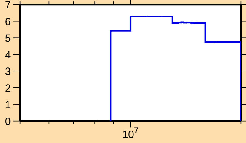
\Delta\sigma/\sigma vs. E for ^{175}\text{Re}(n,\text{el.})
