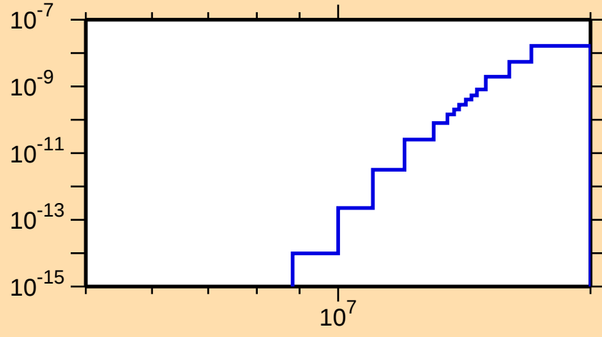
\sigma vs. E for ^{175}\text{Re}(\text{mt117})
