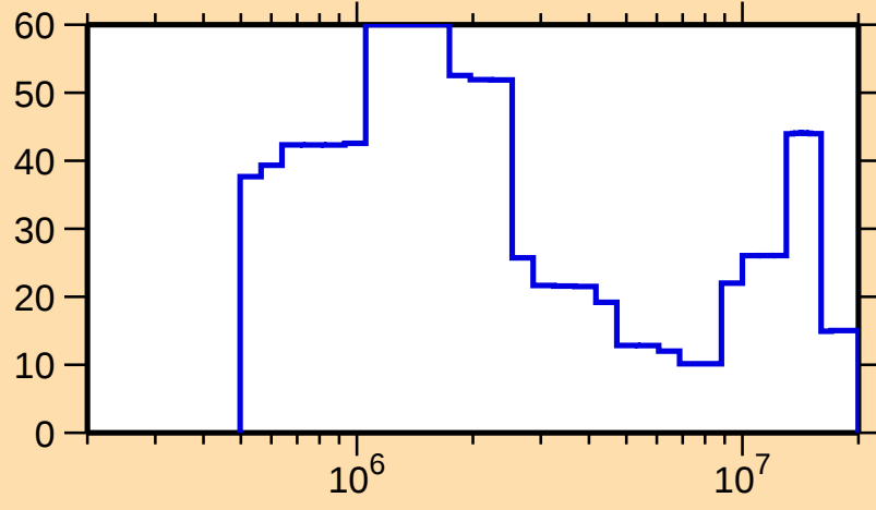
\Delta\sigma/\sigma vs. E for ^{175}\text{Re}(n,\text{inel.})
