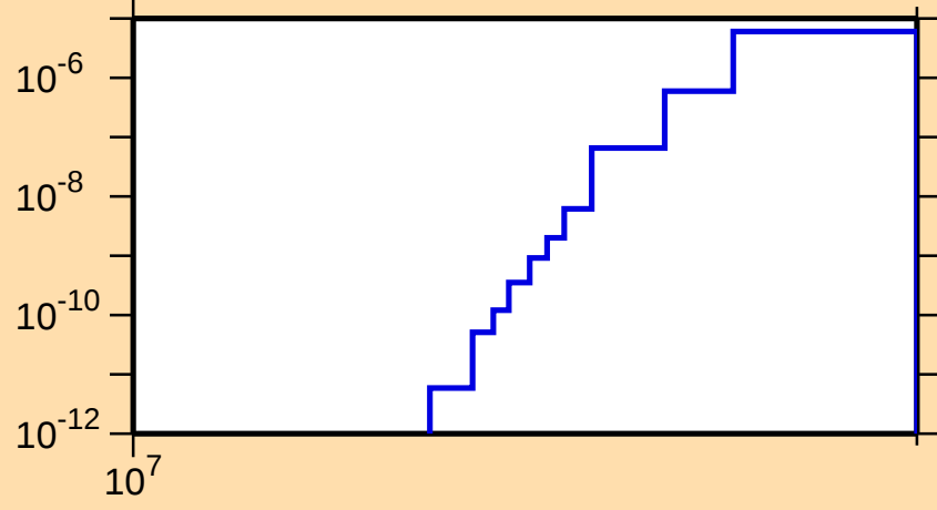
\sigma vs. E for ^{175}\text{Re}(n,\text{nd})
