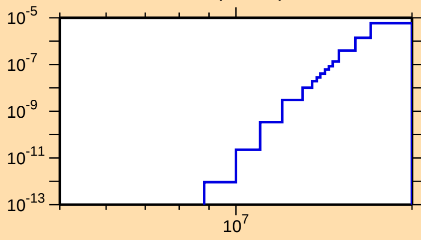
\sigma vs. E for ^{175}\text{Re}(n,\text{He3})
