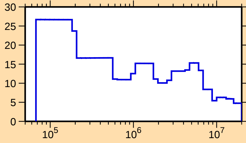
\Delta\sigma/\sigma vs. E for ^{175}\text{Re}(n,\text{el.})
