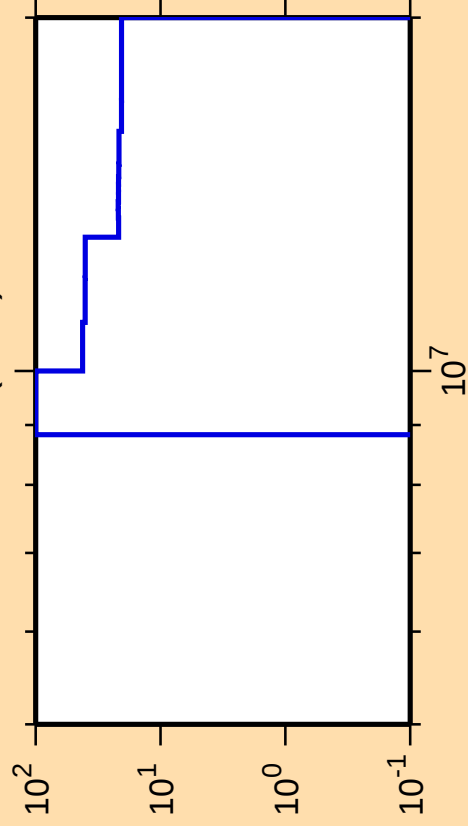
\Delta\sigma/\sigma vs. E for ^{175}\text{Re}(n,2n)
