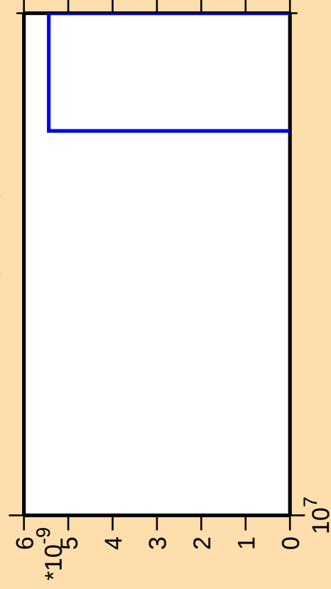
\Delta\sigma/\sigma vs. E for ^{175}\text{Re}(\text{mt } 42)
