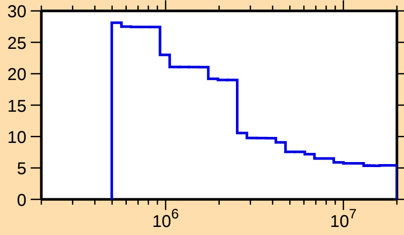
\Delta\sigma/\sigma vs. E for ^{175}\text{Re}(n,n\text{onel.})
