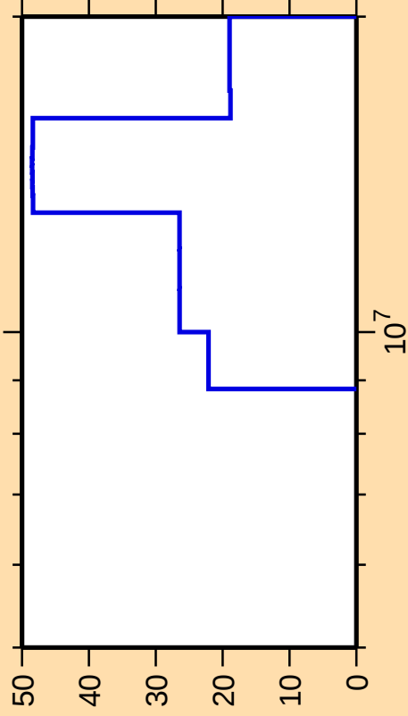
\Delta\sigma/\sigma vs. E for ^{175}\text{Re}(n,n\text{cont.})
